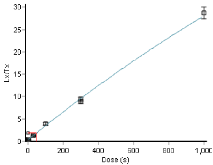
Figure 1: Simulation of dose determination using a laboratory irradiation of a natural K-feldspar sample, mounted in a stainless steel cup. This sample was exposed to the attenuated beta source for 50s, and this dose was treated as a natural dose, which was then recovered as an apparent dose of 51.2 \pm 5.6 s exposure. The signal used was the TL between 140 and 280°C. For reference, 1 s irradiation equates to about 1 days of burial.
