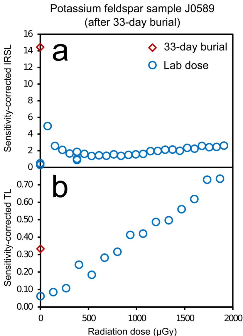
Figure 3: The luminescence responses produced after 33 days of burial are shown as red diamonds for the IRSL (a) and TL (b) signals of sample J0589, enriched K-feldspar separated from a natural sand collected in Southern California. Natural sunlight at the burial site was used to bleach (reduce) the stored electron population, before burial in the ground and subsequent recovery. The equivalent dose estimated with the TL signal ( 435 \pm 8 \mu\text{Gy} ; n=3 discs) agrees within 1\sigma with the known geologic dose of 431 \pm 25 \mu\text{Gy} . The IRSL signal appears to suffer from poor bleaching and dose artefacts, and does not appear suitable for dating in this low range using the protocol applied.
