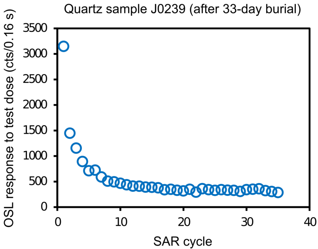
Figure 4: The systematic decrease in OSL sensitivity throughout subsequent SAR cycles implies that the measurement conditions may need to be optimized in order to measure very low doses in quartz. This behaviour, which produces growth curves that decrease with dose initially, represents the phenomenon of dose quenching (Bailey, 2001), and its form may have significant implications for the mechanisms responsible for quartz OSL and TL production.
