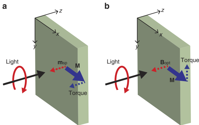
Figure 1 | Schematic representation of two orthogonal torques. Circularly polarized light, incident on magnetization of ferromagnet ( \mathbf{M} ), generates either spin polarization ( \mathbf{m}_{\text{sp}} ) via optical orientation or optomagnetic field ( \mathbf{B}_{\text{opt}} ) via inverse Faraday effect. (Black arrow indicates a wavevector of light along the z -direction, and red circular arrow indicates left-circular polarization.) (a) The \mathbf{m}_{\text{sp}} (red dotted arrow) rotates \mathbf{M} (blue solid arrow) to the z -direction by spin-transfer torque (blue dotted arrow). (b) The \mathbf{B}_{\text{opt}} (red dotted arrow) rotates \mathbf{M} (blue solid arrow) to the y -direction by field-like torque (blue dotted arrow).
