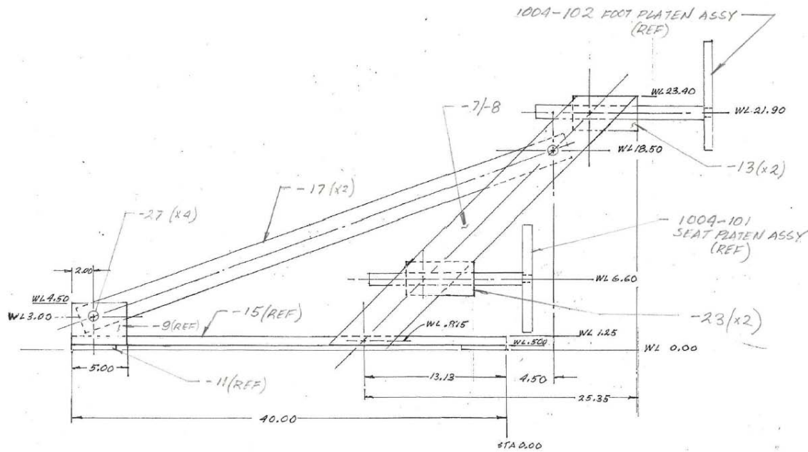
Figure 3: Carriage Assembly
