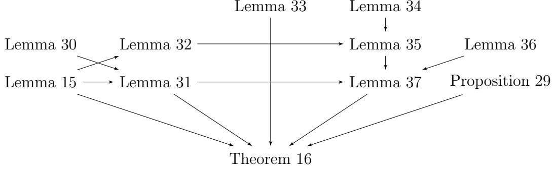
Figure 11. A directed graph to illustrate the development of the Lemmas in proving Theorem 16 where the predecessor of a statement is included in the statement’s proof.
