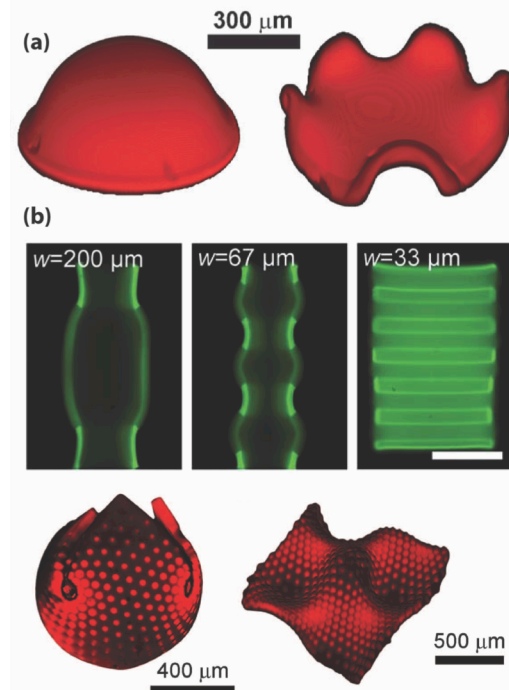
Figure 2. (a) Programmed shapes prepared by grayscale lithography. (b) Sheets with alternating stripe width w roll for large w but remain flat for small w (scale bar: 400 \mu\text{m} ). (c) Programmed shapes prepared by halftone lithography.
