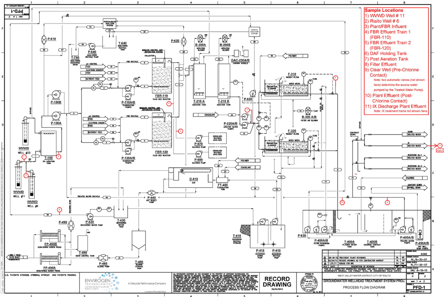
Figure 5.17 Sampling locations in Groundwater Treatment Plant.
