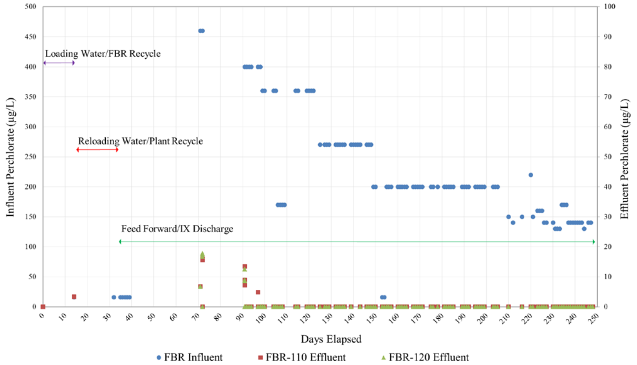
Figure 5.18 Perchlorate Treatment across the FBRs.
