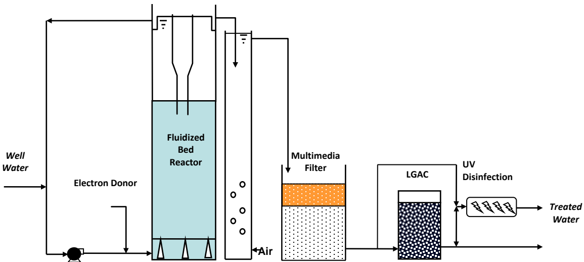
Figure 2.3 Schematic of Pilot-scale FBR Treatment Plant (Webster and Togna, 2009).
