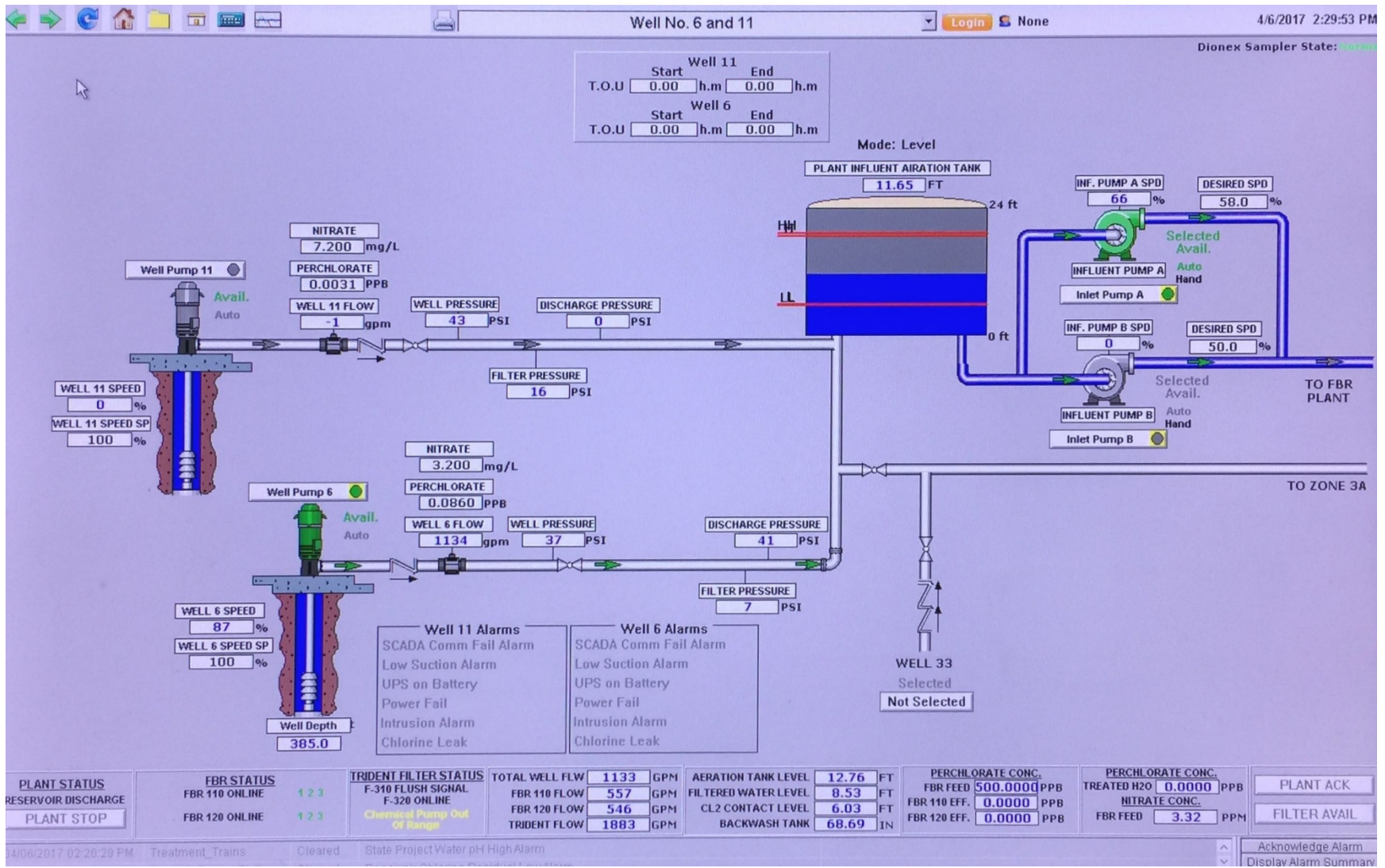
Figure 5.5 SCADA Screenshot of Feed System.
