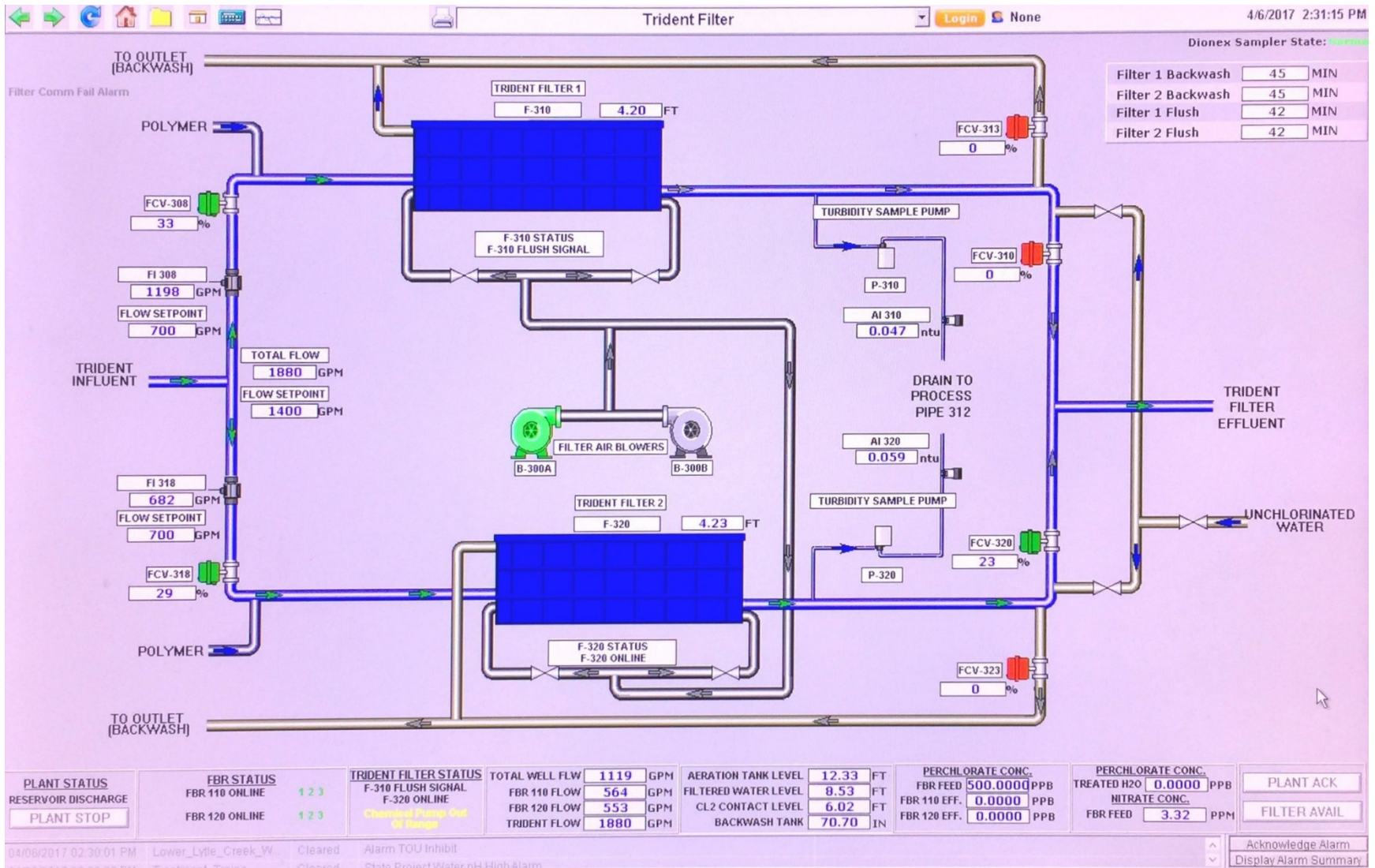
Figure 5.7 SCADA Screenshot of Filtration System.
