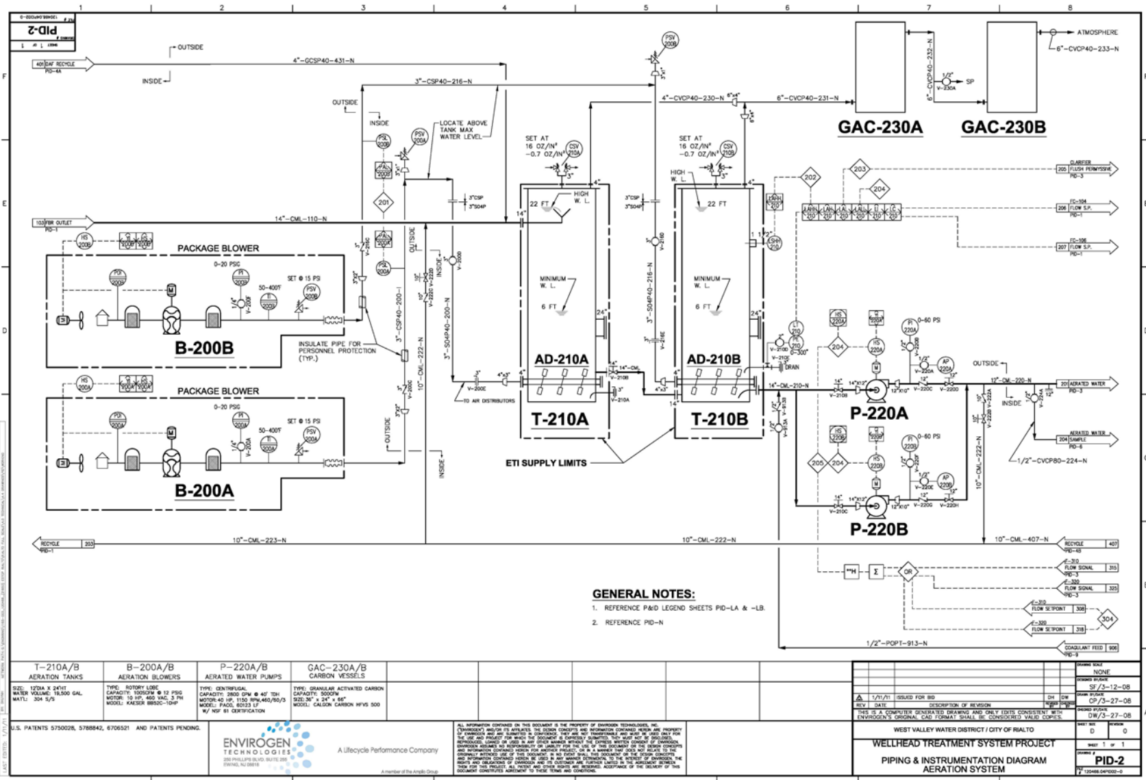
Figure 5.10 Aeration System.
