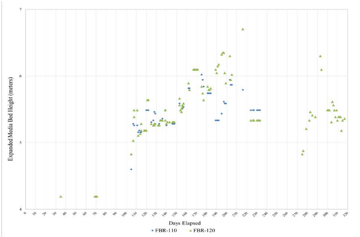
Figure 5.21 Expanded Media Bed Heights for the FBRs.
