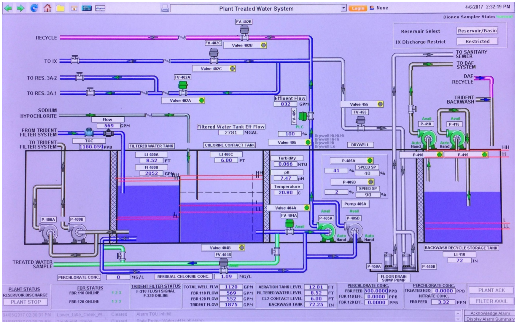
Figure 5.8 SCADA Screenshot of Water Holding System/chlorination System.
