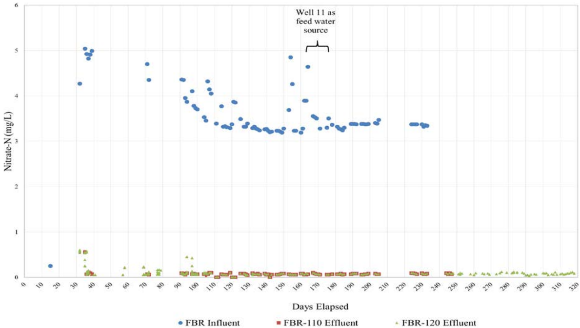
Figure 5.19 Nitrate Treatment across the FBRs.
