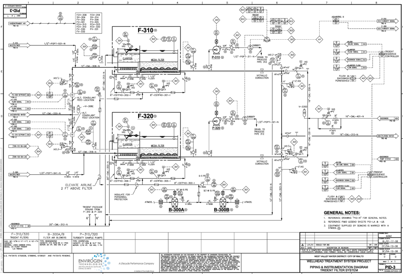
Figure 5.11 Solids Removal - TridentSystem.
