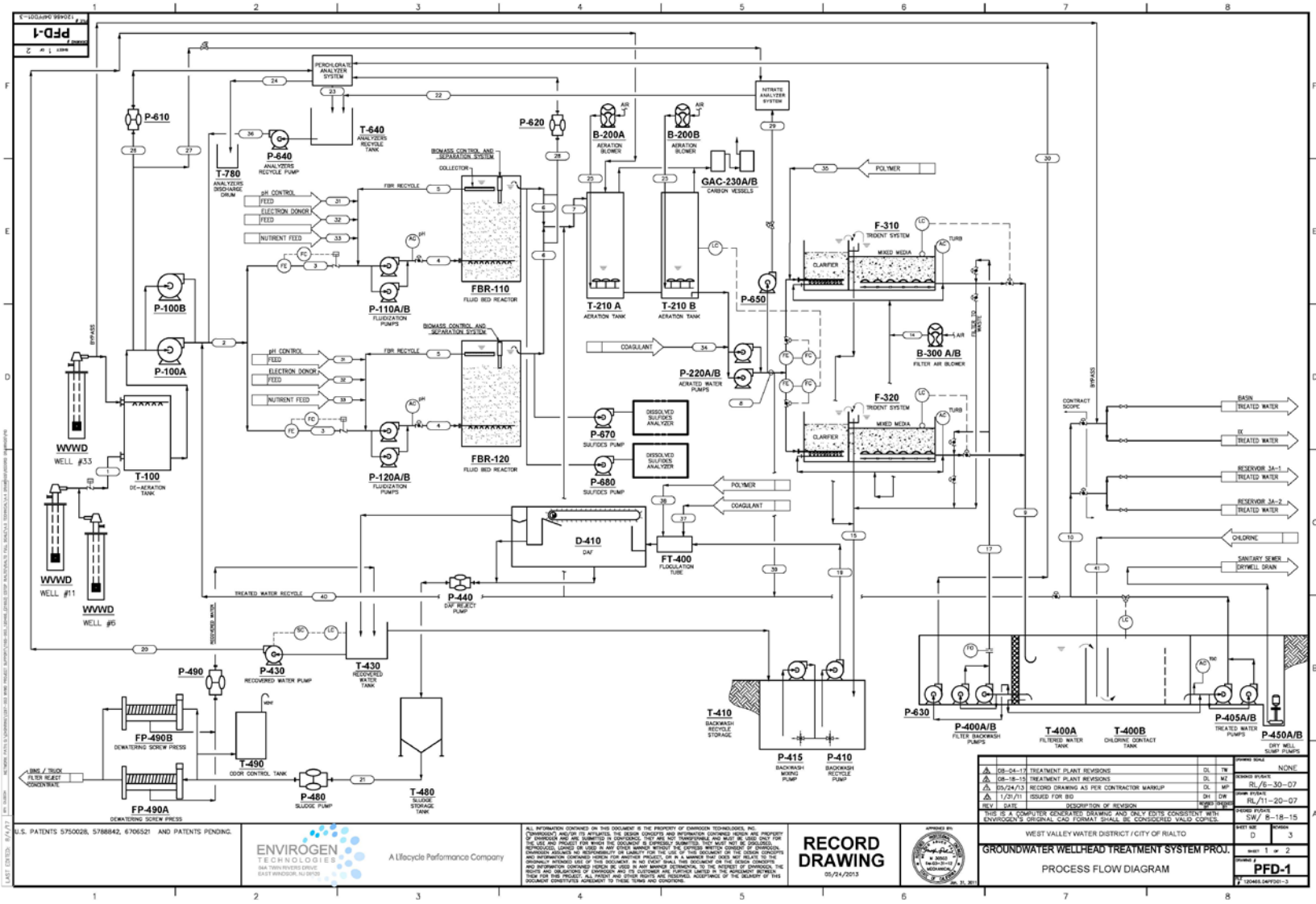
Figure 5.3 Plant Process Flow Diagram.
