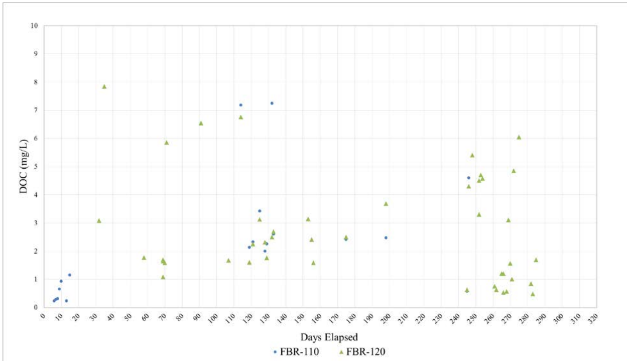
Figure 5.20 Residual Dissolved Organic Carbon for the FBRs.
