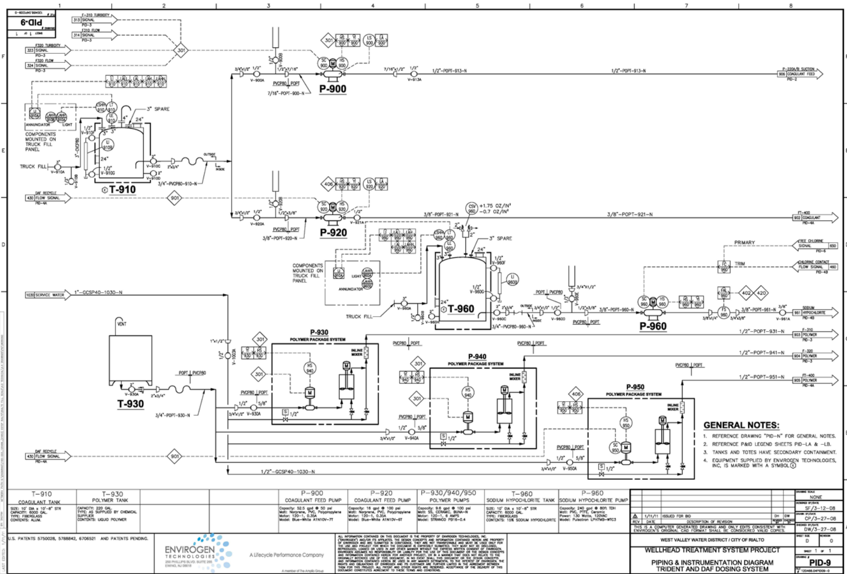
Figure 5.15 Chemical Addition System 2.
