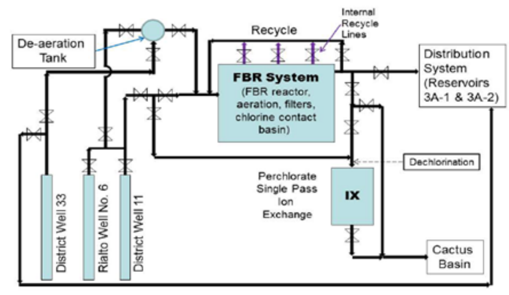
Figure 5.1 Overall Area Process Flow Diagram.
