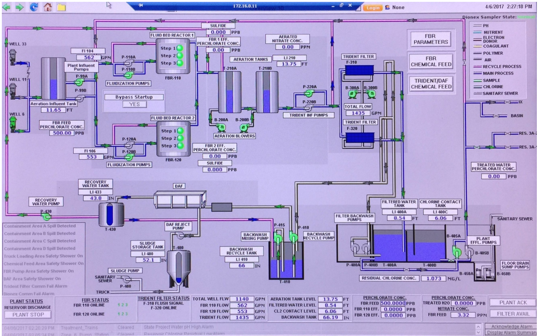
Figure 5.4 SCADA Screenshot of Treatment Plant.
