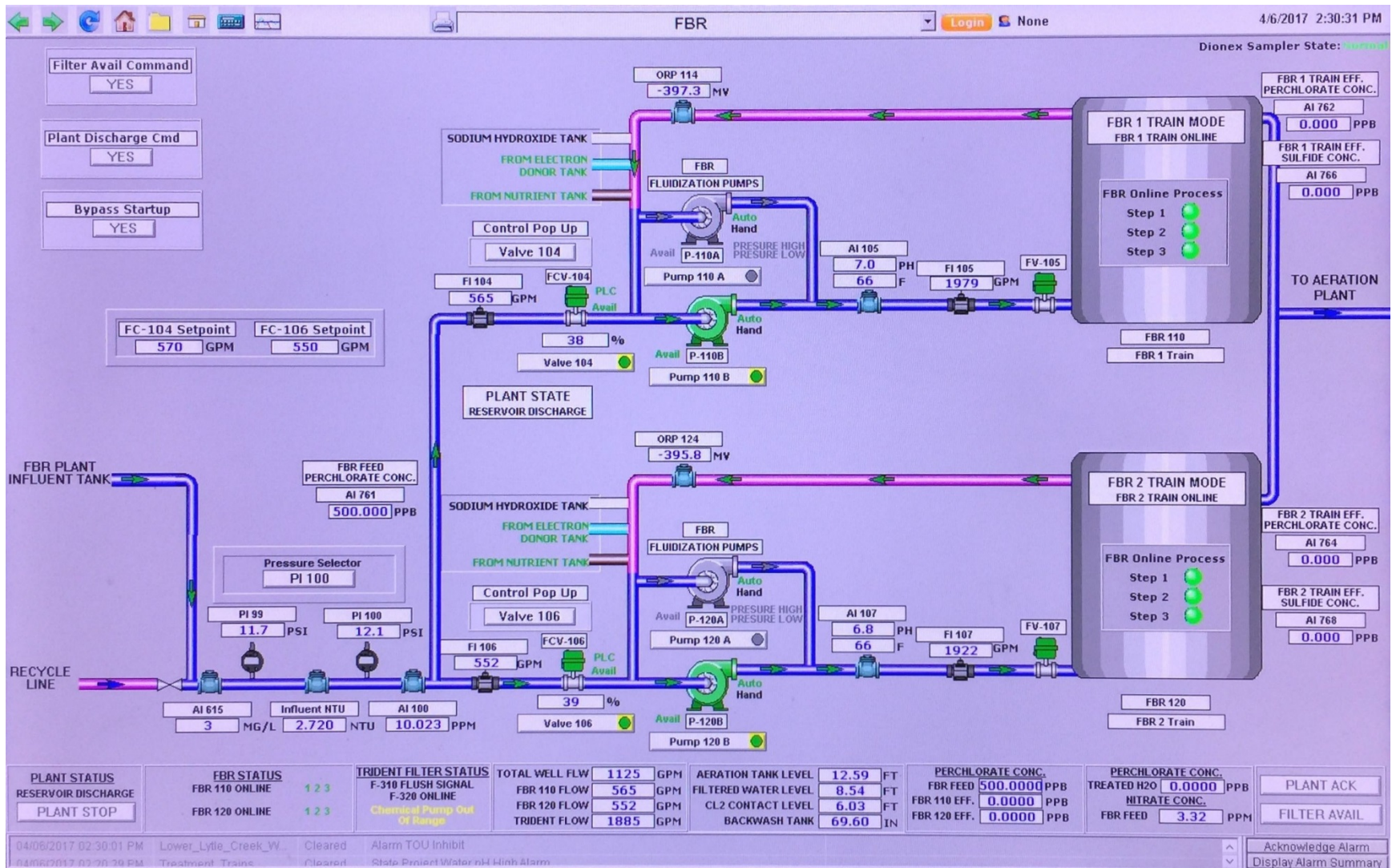
Figure 5.6 SCADA Screenshot of FBR System.
