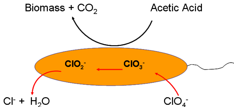
Figure 2.1 Biological Treatment of Perchlorate (from Webster and Togna 2009).
