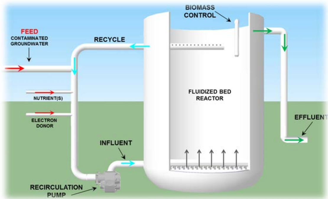
Figure 2.2 Typical Fluidized Bed Reactor Schematic.
