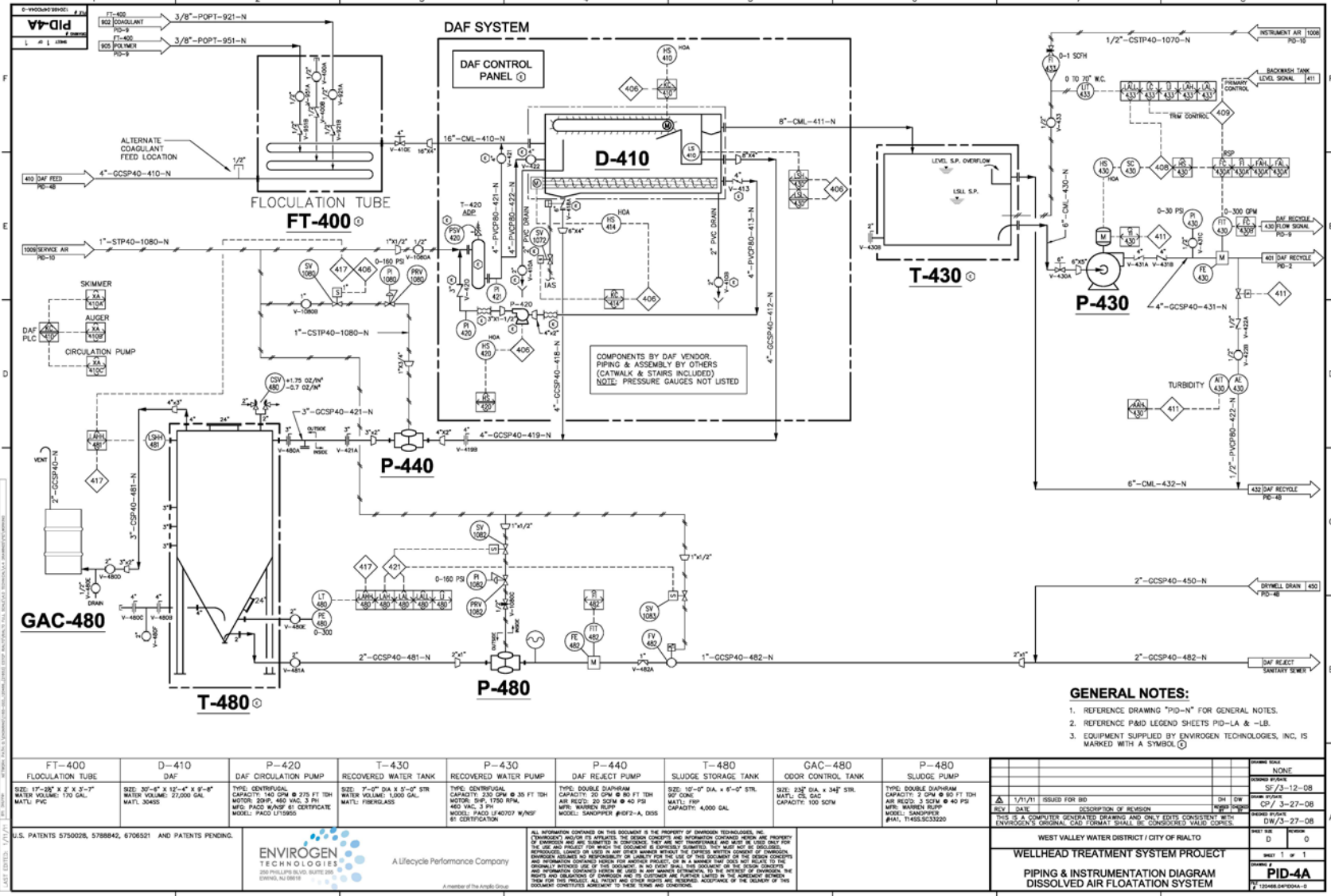
Figure 5.12 Solids Removal- DAF System.
