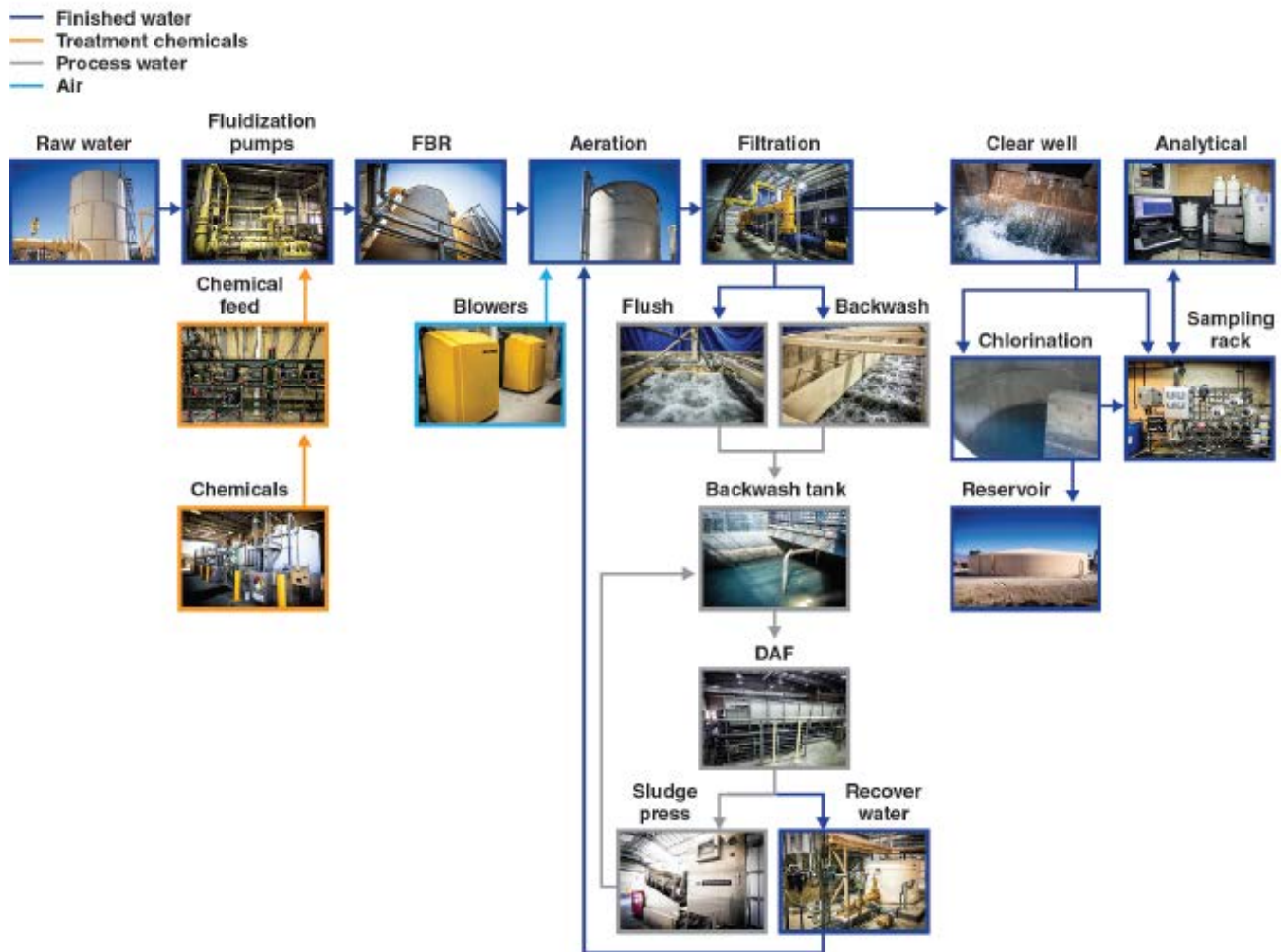
Figure 5.2 Process Flow Layout of Plant (Webster and Litchfield, 2017).
