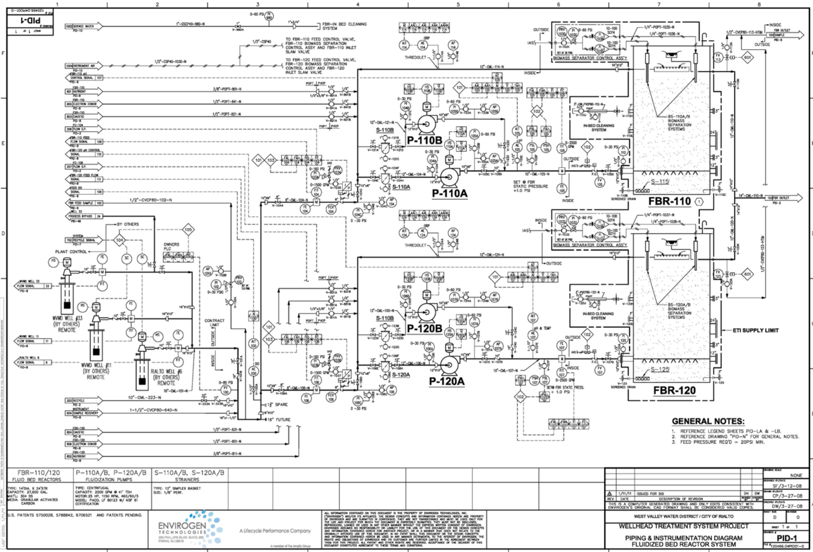
Figure 5.9 FBR System.
