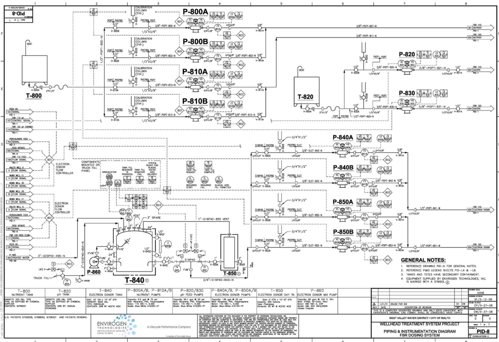
Figure 5.14 Chemical Addition System 1.
