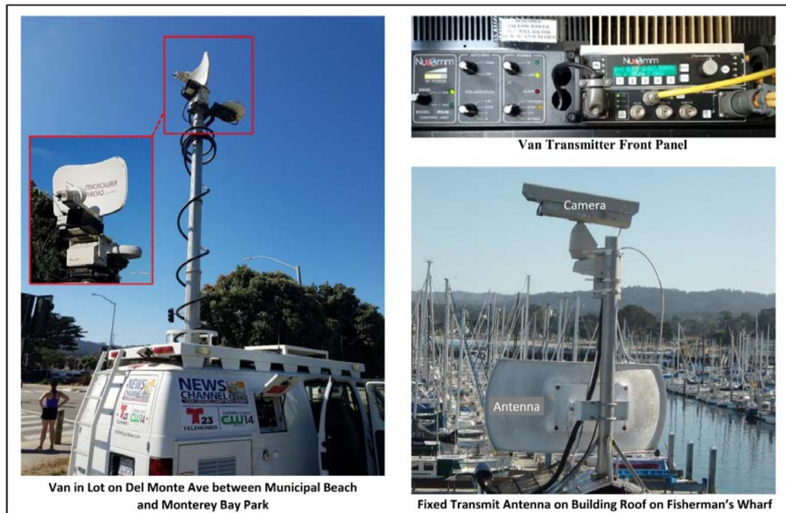
Figure 15. Mobile and Fixed ENG Transmitters [25].
