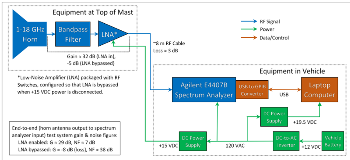
Figure 19. EM Spectrum Analysis Equipment Diagram. Source [25].
