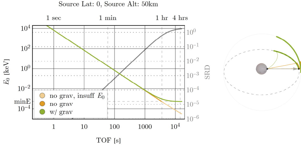
Figure 32: Emission energy as a function of time of flight from an equatorial source at 50 km to a detector at \Delta\alpha = 0^\circ at time of emission with and without gravity.
