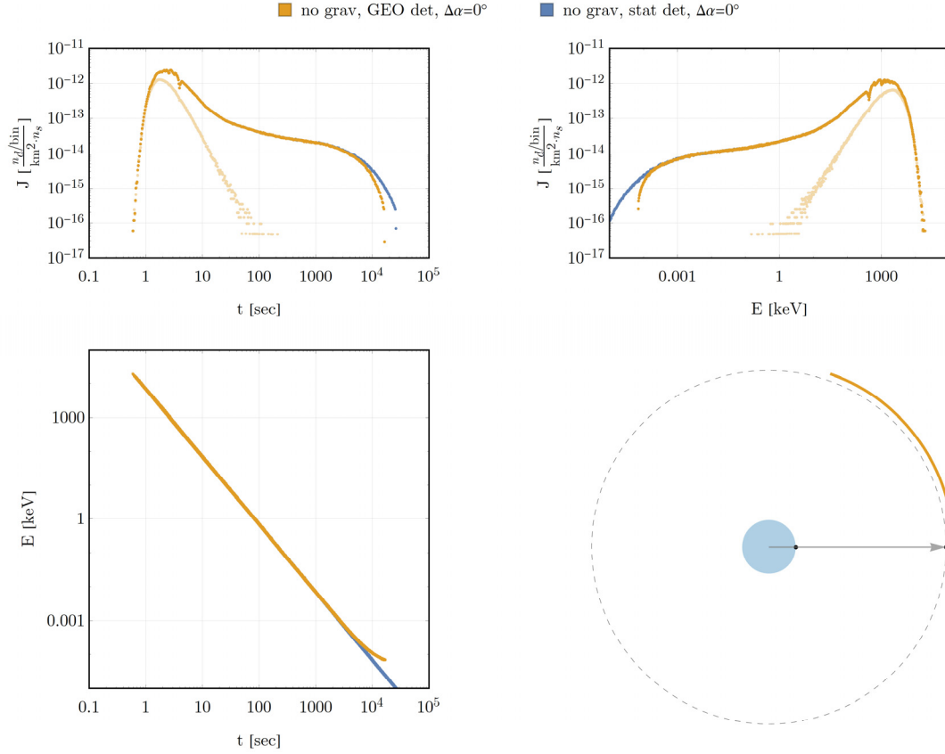
Figure 17: Intercepted neutron current density as a function of time-energy computed by HATS-n for an equatorial Watt-fission-235 neutron source at 50 km as seen by stationary and geostationary detectors at \Delta\alpha = 0^\circ at time of emission.
