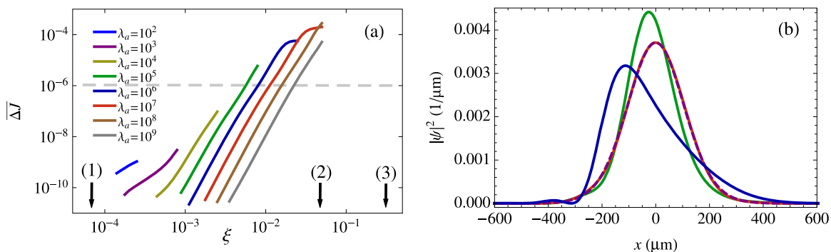
Figure 7. (a) Mean improvement of the optimization functional, \overline{\Delta J} (averaged over 100 iterations), versus relative size of the wavepacket \xi for different optimization weights \lambda_a , cf equation (10), ranging from \lambda_a = 10^2 (leftmost line) to \lambda_a = 10^9 (rightmost line) in powers of ten. The arrows indicate: (1) the parameters corresponding to current trap technology, (2) good convergence of quantum OCT with the invariant based IEA still being valid, (3) fast convergence of quantum OCT with invariant based IEA starting to fail. (b) Final wavefunction amplitudes for \xi = 0.4 (arrow (3) in (a)) and classical optimization (blue, fidelity of 83.8%), IEA (green, 94.6%), quantum OCT (red, fidelity of 99.9%). Also plotted is the target state (purple dashed).
