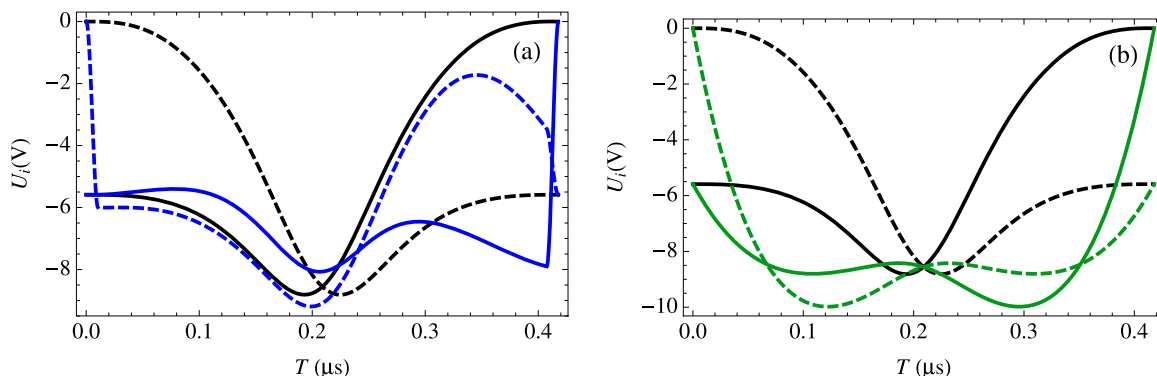
Figure 2. Control voltages applied to electrodes for transporting a ^{40}\text{Ca}^+ ion from electrode 1 (solid lines) to electrode 2 (dashed lines) within 418 ns for an initial trap frequency of \omega = 2\pi \cdot 1.3 MHz: initial guess voltage ramps (a and b, black) and ramps obtained by classical optimization (a, blue) and the invariant based inverse engineering (b, green).
