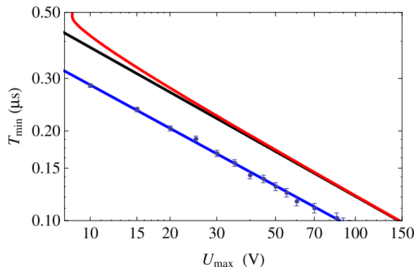
Figure 6. Minimum transport time T_{\min} versus maximum electrode voltage U_{\max} obtained by the invariant based inverse engineering approach: the compensating force method for a trap frequency of \omega = 2\pi \cdot 1.3 MHz using the transport function of equation (B.1) (red) and for the limiting case of vanishing trap frequency (black). Also shown is the classical result from figure 4 (blue).
