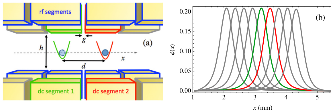
Figure 1. (a) Ion shuttling in a segmented linear trap. The dc electrodes (gray, green, red) form the axial potential for the ion transport along the x -axis. The rf electrodes (blue) ensure confinement of the ions along the x -axis. (b) Axial electrode potentials formed by applying a dc voltage to a facing pair of trap segments. For the specific scenario presented in this manuscript, we use d = 280 \mu\text{m} , g = 30 \mu\text{m} and h = 500 \mu\text{m} . Each potential is generated from a single pair of segments, depicted in red in (a) and biased to 1 V with all the other dc electrodes grounded.
