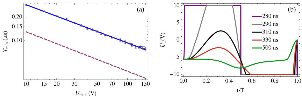
Figure 4. (a) Minimum transport time T_{\min}^{\text{opt}} versus maximum electrode voltage U_{\max} , obtained from numerical optimization of classical transport dynamics (blue dots) along with a fit to equation (28). We also indicate the analytic bang-bang result, equation (31), derived for idealized, purely harmonic potentials (purple dashed line) being proportional to 1/\sqrt{U_{\max}} . The slopes of the curves are clearly similar, indicating the negligible impact of anharmonicities on the scaling of T_{\min}^{\text{opt}} with U_{\max} . (b) Optimized voltages for the left electrode with U_{\max} = 10 V: the shorter the transport time, the more the ramp approaches a square shape. The rectangular bang-bang-like solution is attained at T = 280 ns, where the classical control of energy neutral transport breaks down due to an insufficient voltage range.
