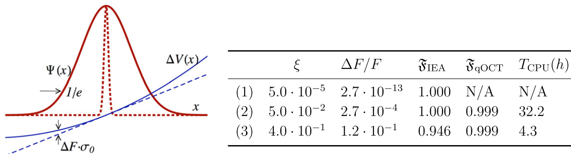
Figure 8. Limitation of the compensating force approach. A force inhomogeneity \Delta F = \sum_i [\phi'_i(\alpha(t) + \sigma_0) - \phi'_i(\alpha(t) - \sigma_0)] \delta U_i(t) across the wavefunctions is caused by anharmonicities of the potential \Delta V = F(t)x used to implement the compensating force. The relative spread of the force \Delta F/F across the wavefunction is taken at the point in time, where the acceleration \ddot{\alpha}(t) is maximal. \Delta F/F increases to the range of several percent for large wavefunction extents. This leads to a drop in the fidelity \mathfrak{F}_{\text{IEA}} . Also shown is the fidelity \mathfrak{F}_{\text{qOCT}} obtained by optimizing the quantum dynamics. The CPU time T_{\text{CPU}} required for optimization could be easily reduced by a factor of 8 in case (3) compared to case (2) due to the better convergence of quantum OCT in this regime.
