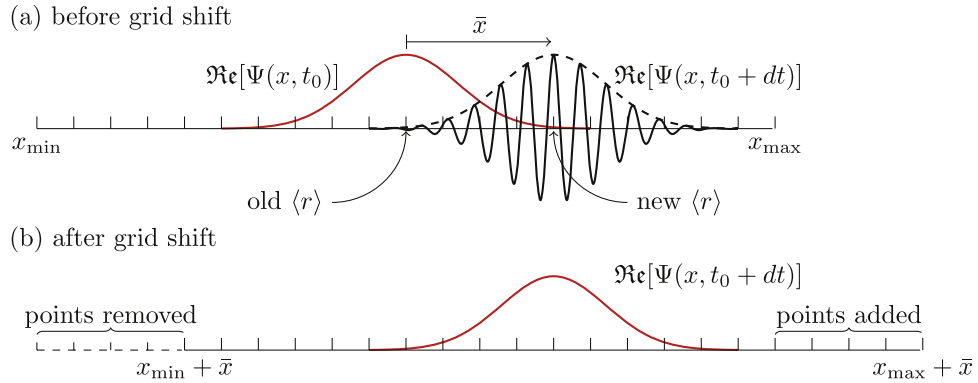
Figure A1. Illustration of the moving grid procedure. The propagation of the wave function \Psi(x, t_0) for a single time step is shown in (a). The resulting wave function has moved in position and has non-zero momentum. After shifting the grid in coordinate and momentum space, the propagated wave function is now centered on the new grid and has zero momentum (b).
