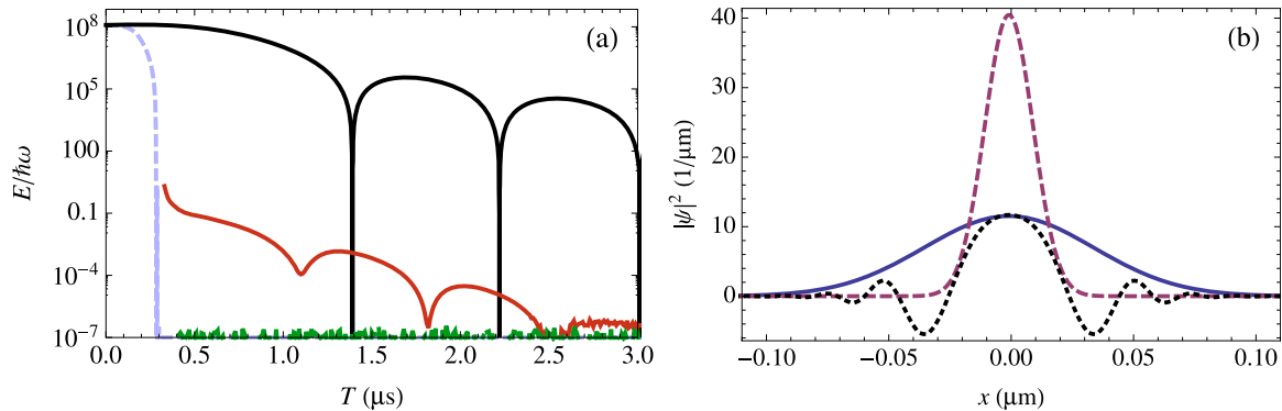
Figure 5. Testing control strategies obtained with classical dynamics for wavepacket motion: (a) final excitation energy of the ion wavepacket with the initial guess (black) and the optimized voltage ramps with U_{\text{max}} = 10 \text{ V} (red). Also shown is a solution obtained by invariant based inverse engineering for a quantum mechanical harmonic oscillator (green). For comparison, the final excitation energy obtained by solving the classical equation of motion with the optimized ramp is shown in light blue. Note that for the initial guess (black), the relative difference between wavepacket and classical motion is not visible on the scale of the figure (less than 10^{-3} ). (b) Final wavefunction |\Psi(T)|^2 (blue) for classically optimized transport with T = 320 \text{ ns} and U_{\text{max}} = 10 \text{ V} and target wave function |\Psi^{\text{tgt}}|^2 (purple dashed). Also shown is the scaled real part of the final wavefunction \Re(\Psi(T)) (black dotted). The clearly visible spread of the wavepacket corresponds to squeezing of the momentum.
