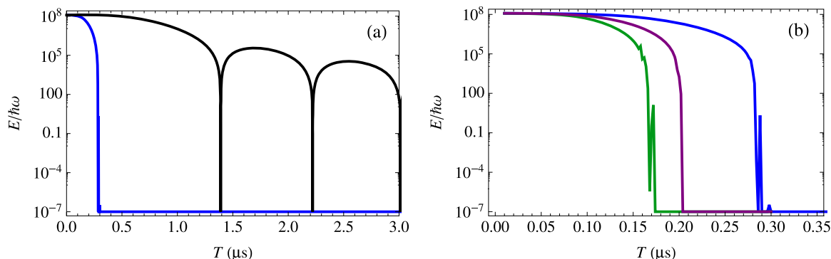
Figure 3. Final energy versus transport time for different voltage ramps and classical dynamics. (a) Shows the improvement over the initial guess (black) by numerical optimization for a maximum voltage of 10 V (blue) and (b) compares the results of numerical optimization for maximum voltages of 10 V (blue), 20 V (purple) and 30 V (green). The spikes in (b) are due to voltage truncation.
