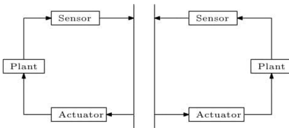
Fig. 1: Control loops
