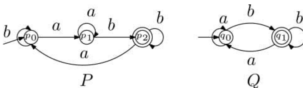
Fig. 2: Individual automaton
