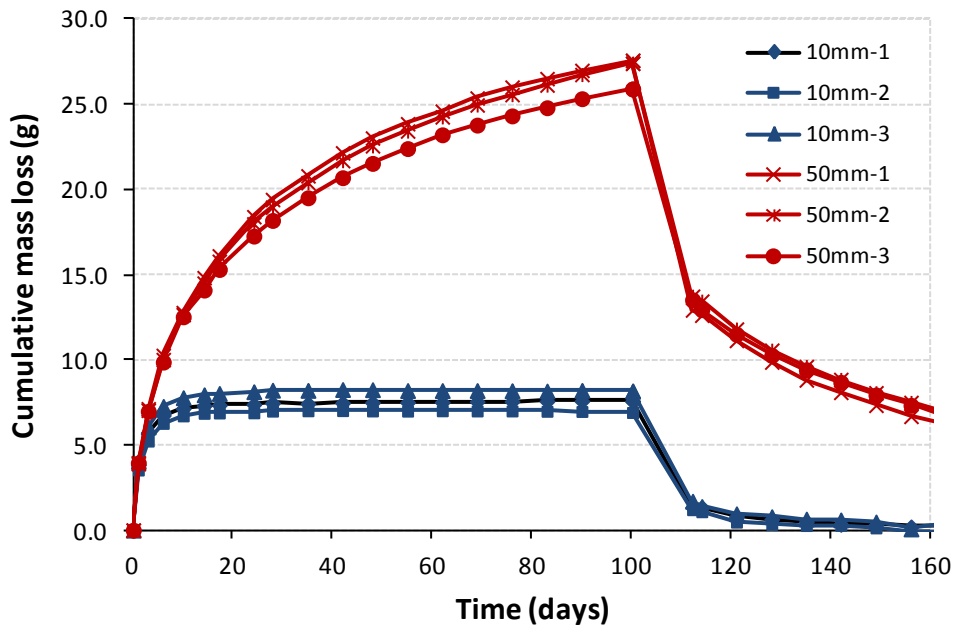
27 - Result of drying-75%RH/absorption for M6 (0.55 w/c+Hycrete-2gal)-91d
