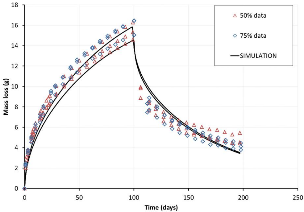
Figure 34 - Simulation of drying/absorption - 0.45 w/b FA mix + 2 gal/yd 3
