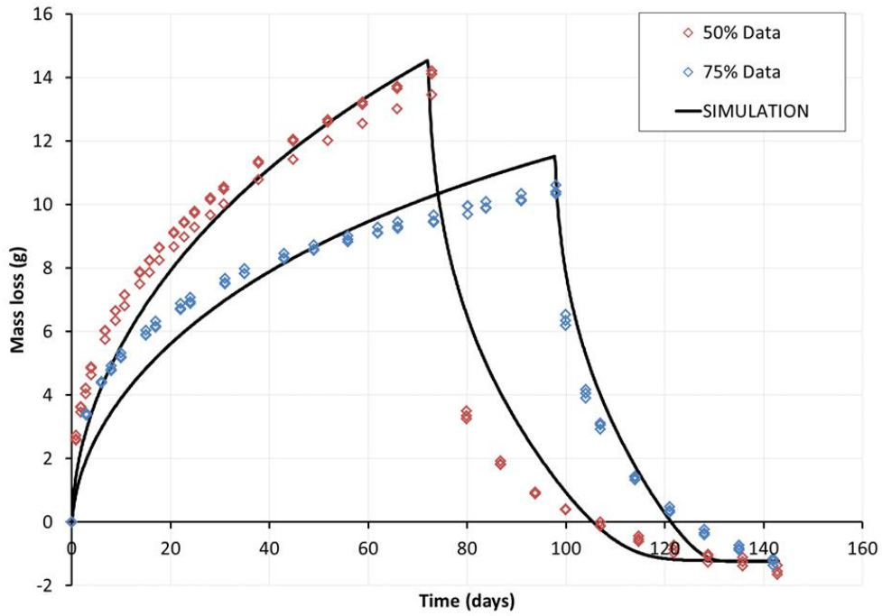
Figure 31 - Simulation of drying/absorption - 0.4 w/c OPC mix w/o Hycrete®
