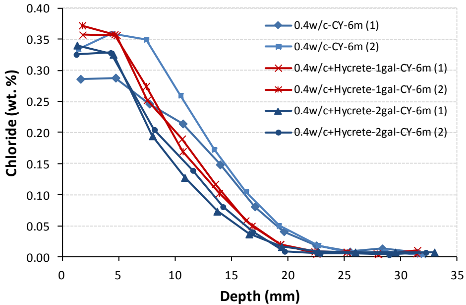
10 - Effect of Hycrete® on mixtures of 0.4 w/c after 180 days' cyclic ponding
