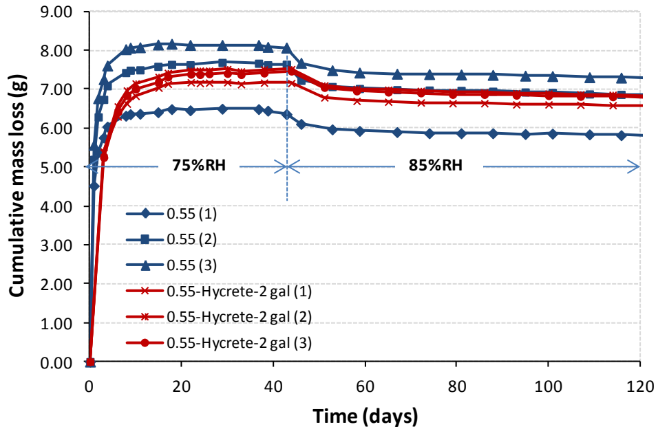
43 - Result for M4 & M6 (0.55 w/c): drying at 75%RH & 85%RH
