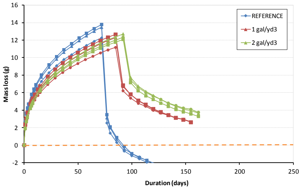
Figure 10 - Drying/absorption of the 0.4 w/c OPC mix cured 28 days and dried at 50% RH
