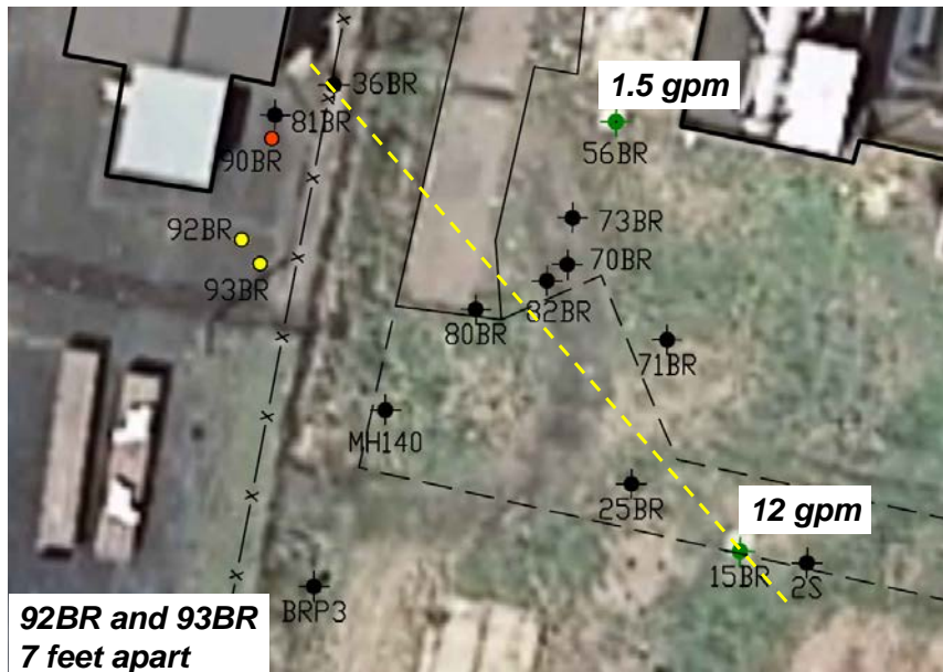
Figure 4.1. Demonstration Location at the NAWC Site.
