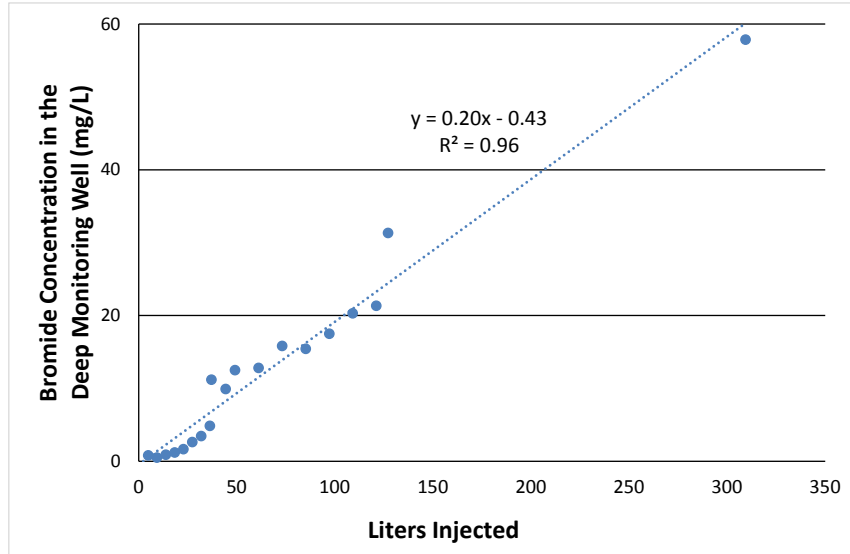
Figure 5.4. Increases in Bromide Concentration in the Deep Interval of MW07-46R as a Function of Volume Injected into MW07-05R.
