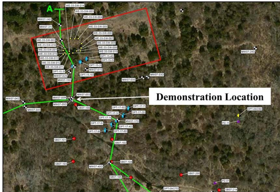
Figure 4.3. Close-up View of the Demonstration Location at CPP. Centered at existing bedrock well MW07-05R.
