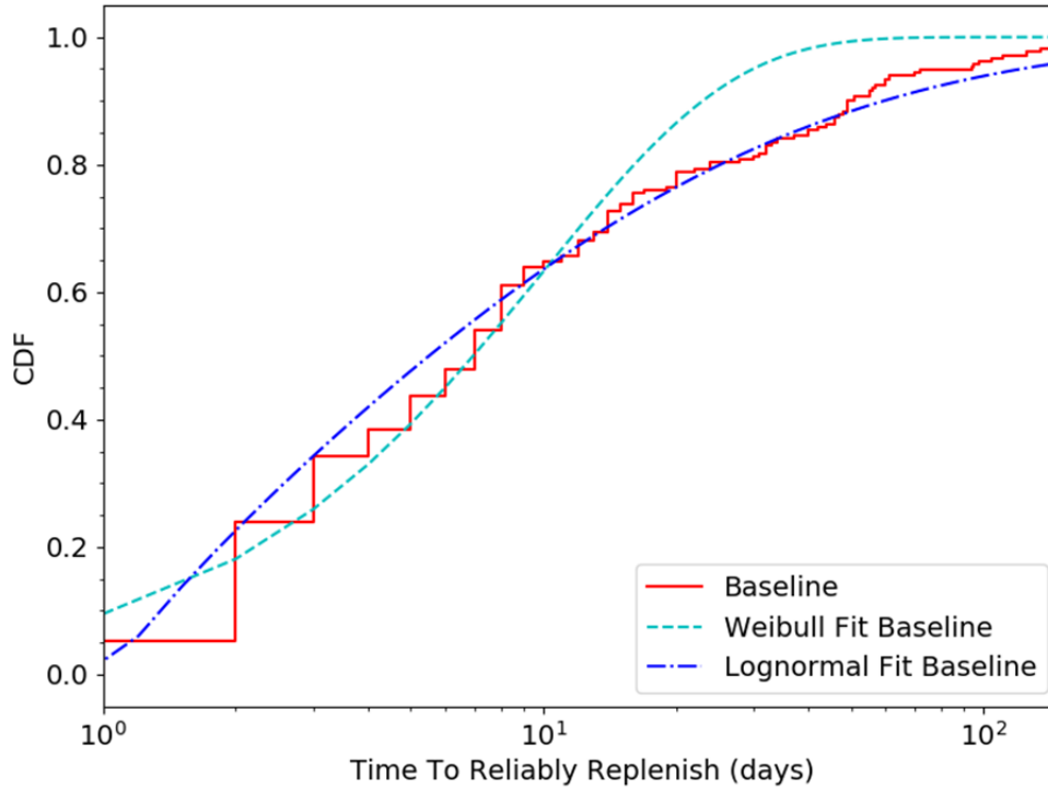
Figure 5. Illustration of Weibull and lognormal CDF fit to the baseline distribution
