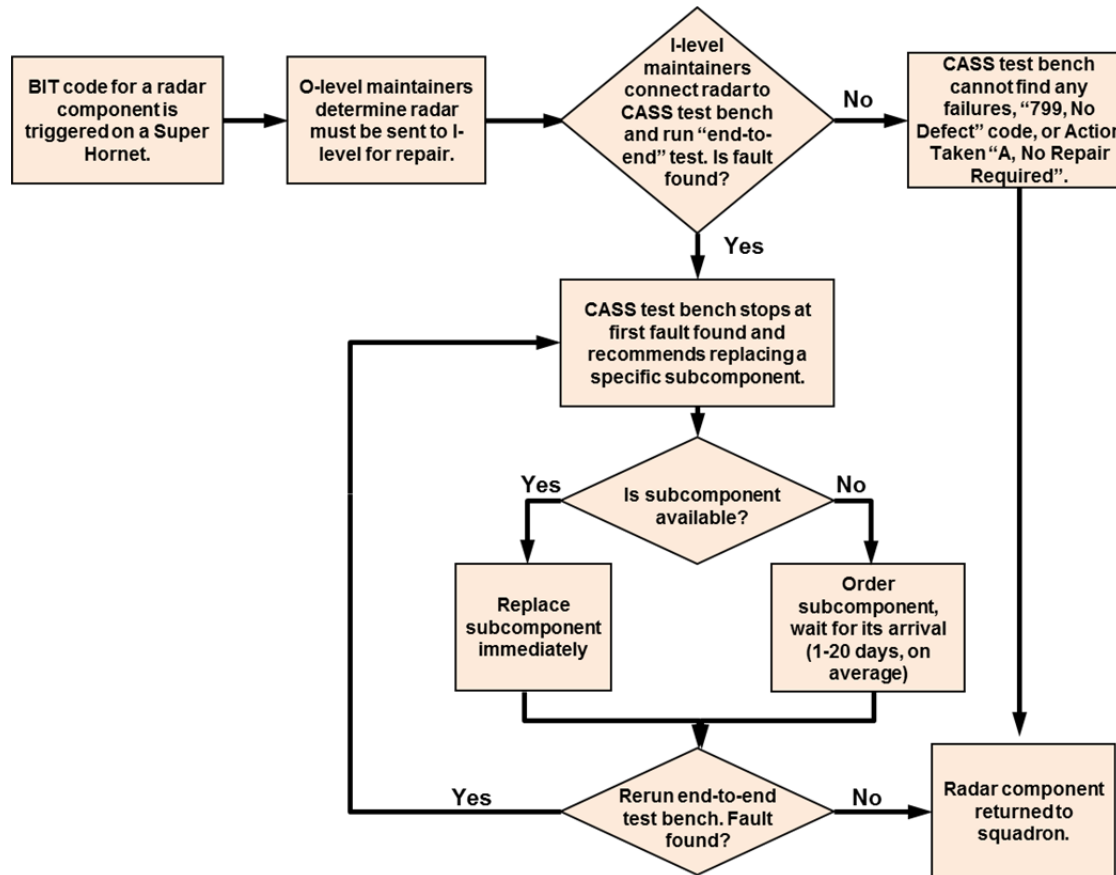
Figure 1. Traditional repair flow from O- to I-level
