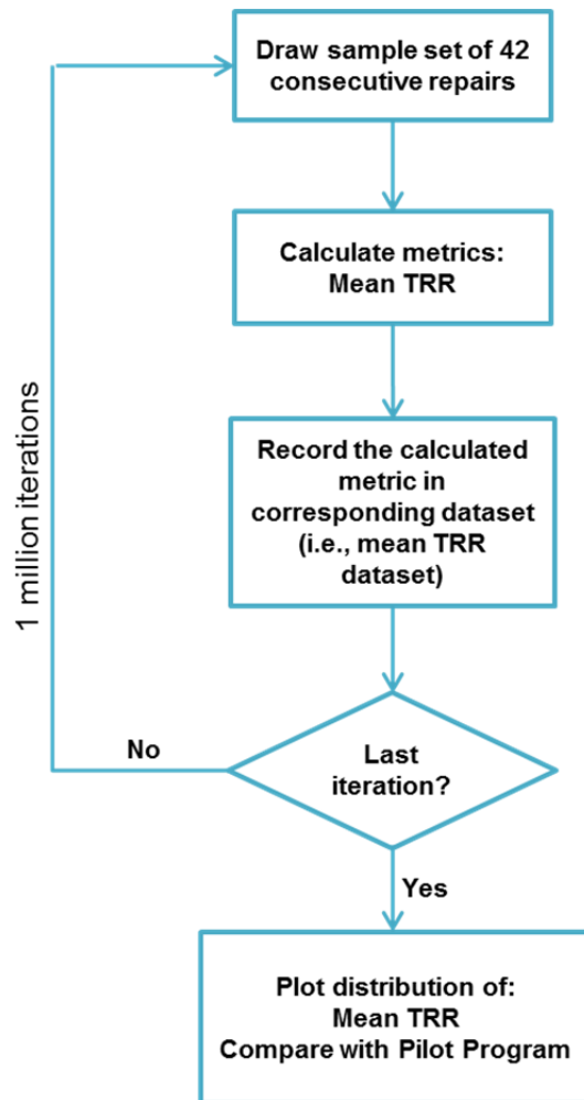
Figure 6. Monte Carlo approach diagram
