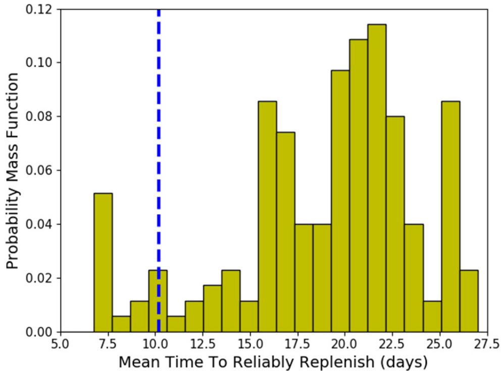
Figure 4. Monte Carlo comparison of baseline program versus pilot program data mean TRR a
