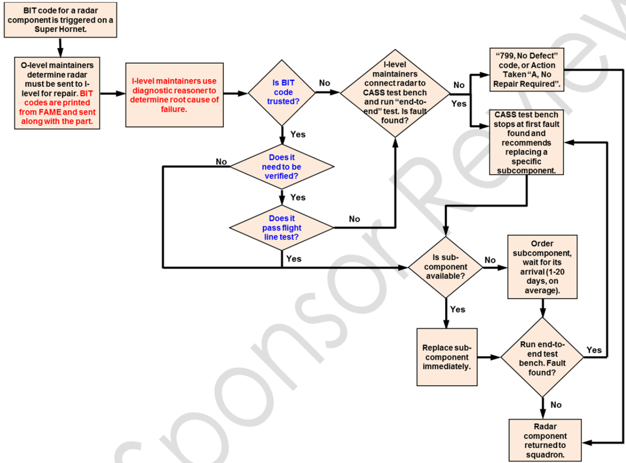
Figure 2. Pilot program repair flow from O- to I-level
