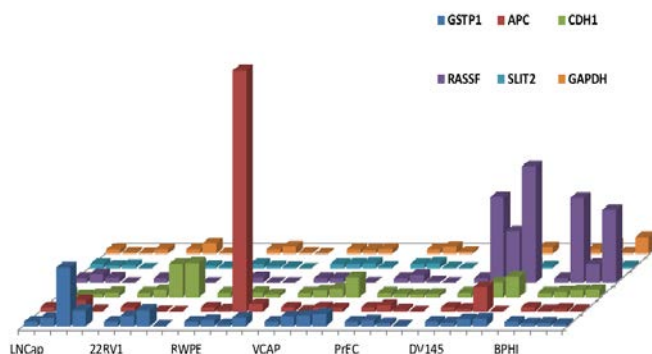
Fig.1 5mCSL and 5hmCSL pull down using DNA from various prostate cancer cell lines. The enriched DNA was then subjected to QPCR analysis of 5 previously reported methylated genes in prostate cancer (GSTP1, APC, CDH1, RASSF2, SLIT2) and a control gene (GAPDH). For each gene at each condition, shown on the left are 5hmC and on the right are 5mC with duplicates.
