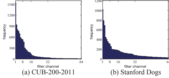
Figure 3. Response distributions of the top scored 10K patches on VGG-M (512 channels). The top scored responses only focus on a few channels. We remove the channels with lower response frequency for better visualization.
