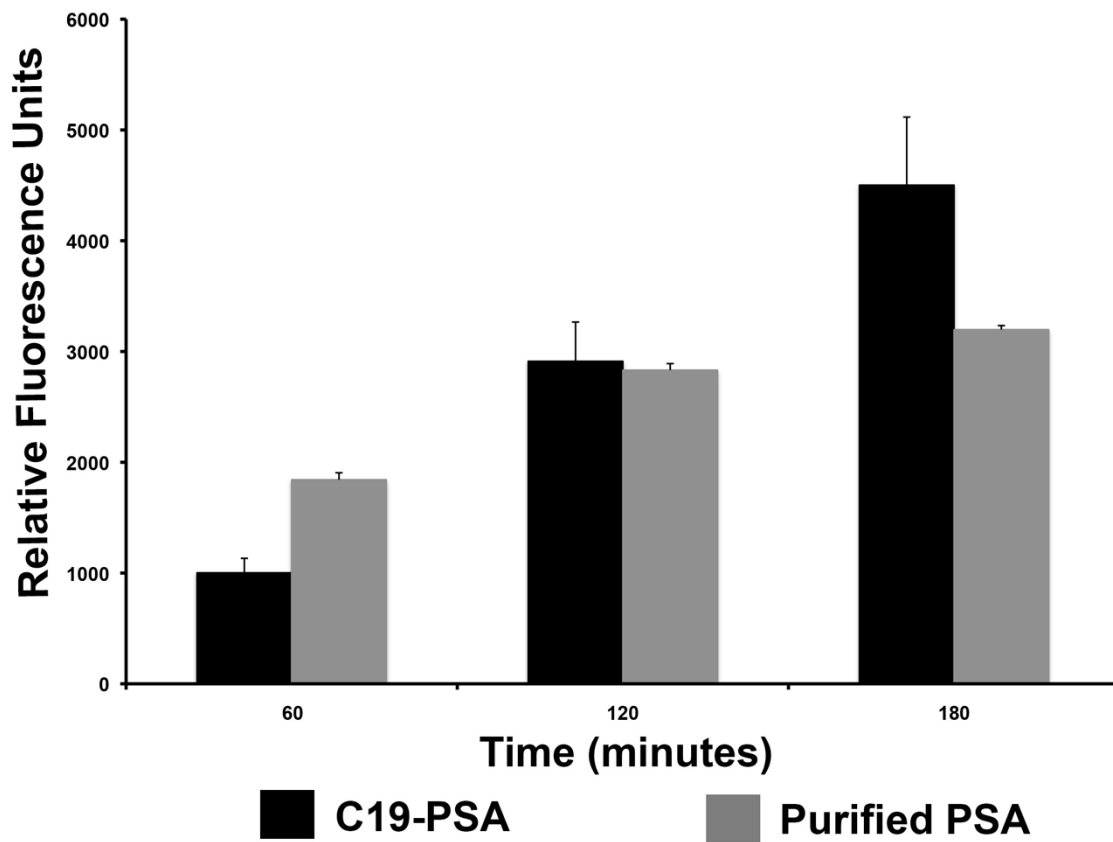
Figure 7. PSA activity assay. Conditioned media from C19 cells transduced to constitutively express PSA was collected and pooled. Activity of secreted PSA was determined using an AMC linked substrate specific for PSA. Activity of C19 secreted PSA is compared with 1ug of purified Human PSA.
