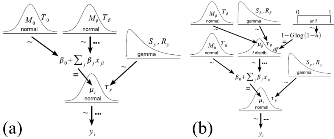
Figure 15. JPM diagrams for two multiple linear regression models. Source: Kruschke (2014). The panel on the left (a) depicts a non-hierarchical model in which the hyperparameters are fixed. The panel on the right (b) depicts a hierarchical model in which the hyperparameters of the Bayesian priors are treated as random variables and influenced by the data via hyperpriors. Standard, non-hierarchical priors with fixed hyperparameters (i.e., hyperpriors) are placed on the hierarchical hyperparameters.
