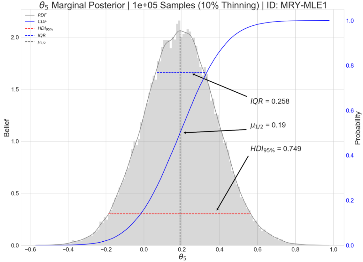
Figure 32. Distribution of discrete posterior parameter samples obtained from “thinning” the “Similar” (blue) Markov chain in Figure 31. Posterior samples are indicated with a grey histogram and superimposed KDE for the PDF; the cumulative distribution function (CDF) is plotted in solid blue over the model parameter. The sample median is indicated with a dashed black line; the narrowest interval containing (50%) 95% of the probabilistic mass is indicated with a dashed (blue) red line.
