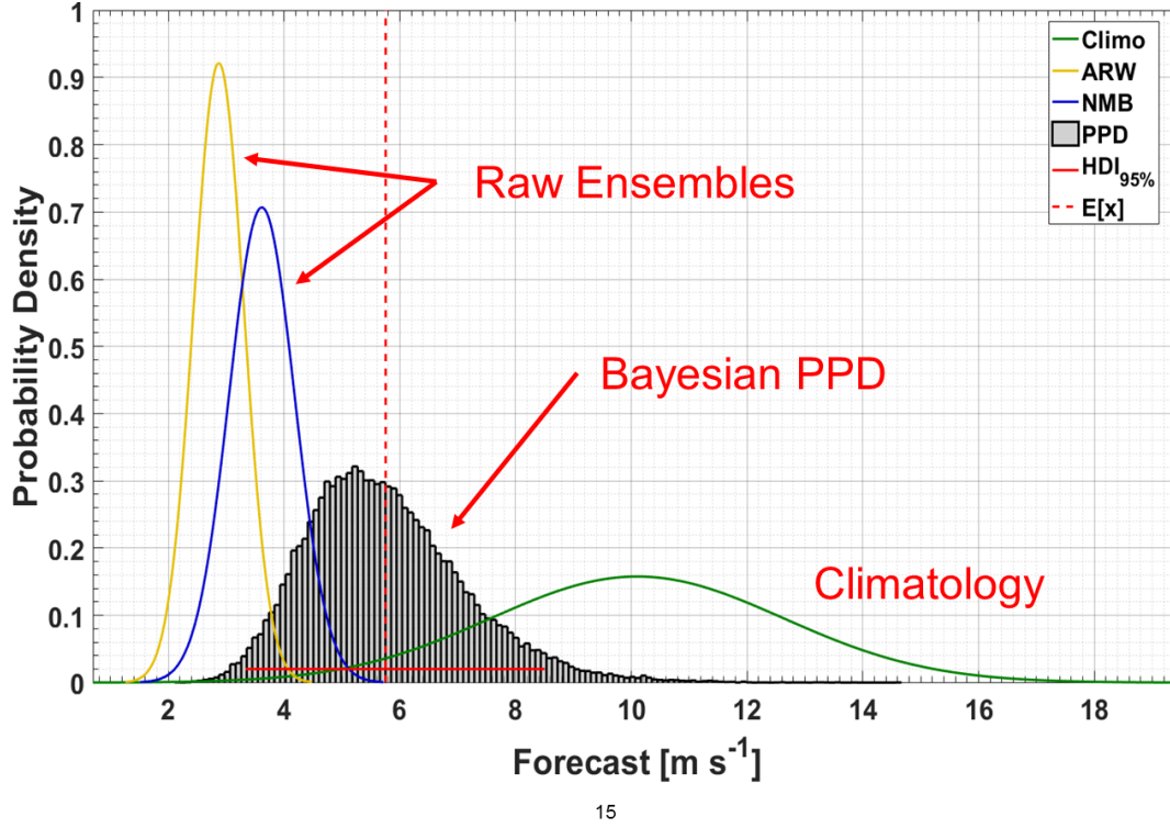
Figure 4. Predictive distributions for 24-hour forecasts of diurnal maximum surface wind speed. The raw ensemble output (yellow and blue) is sharper (i.e., more concentrated) than Bayesian (histogram) and climatological (green) estimates. A highest density interval (HDI; solid red) describes the narrowest portion of the PPD containing a specified probabilistic mass fraction (e.g., 95% as shown).
