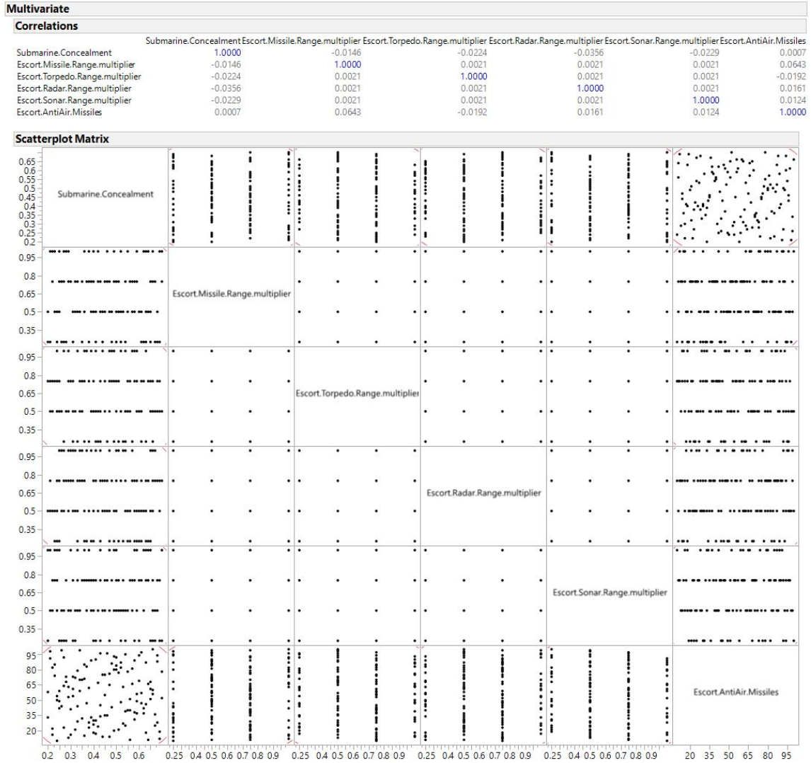
Figure 20. NOLH design of experiment — scatter plot matrix.
