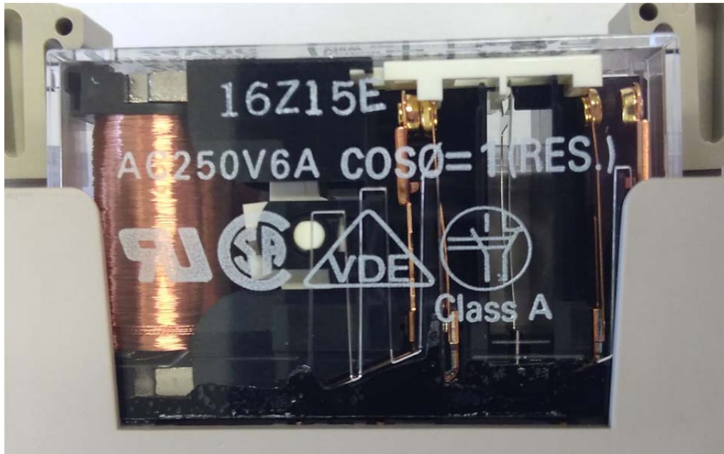
Figure 20 Electromagnetic Relay
