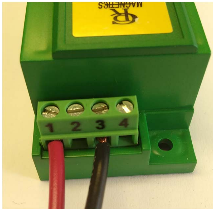
Figure 35 Voltage Transducer Input Terminal
