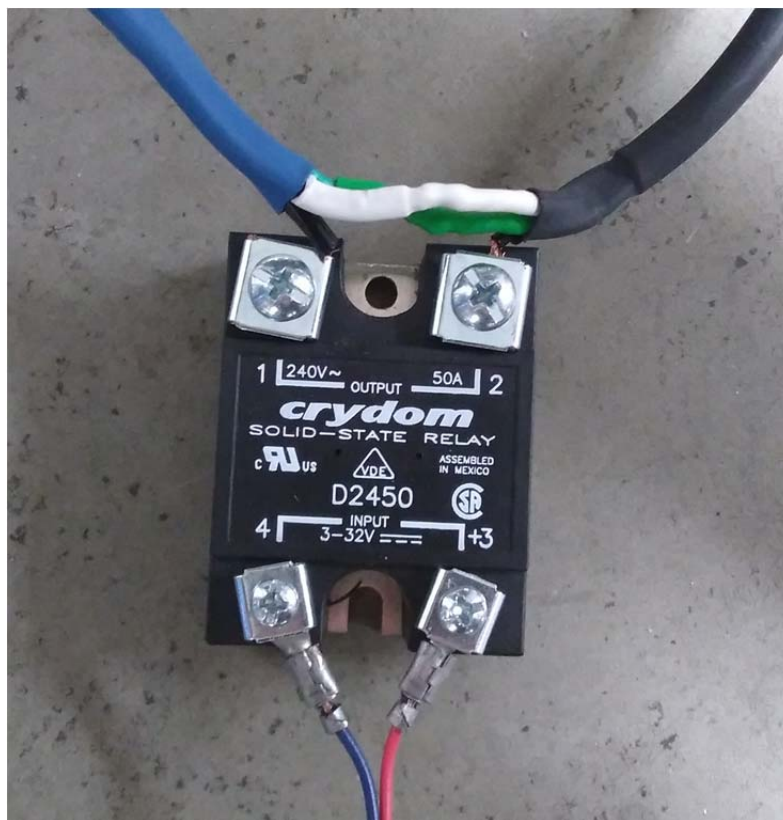
Figure 40 SSR with Solenoid and Micro 850 Attached
