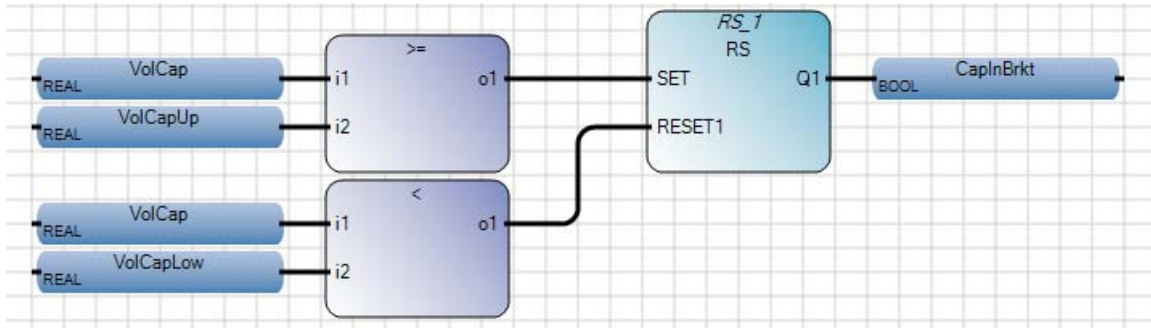
Figure 51 Boundary Checking Sub Program
