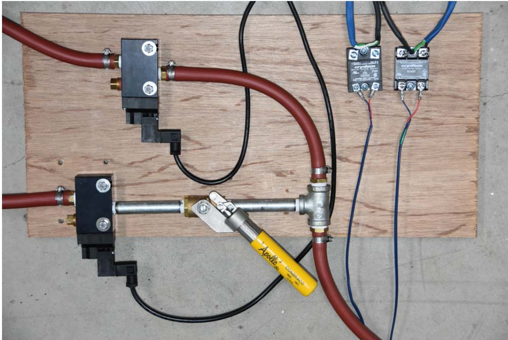
Figure 25 Control Manifold
