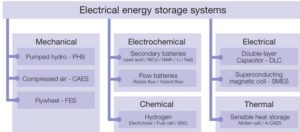
Figure 3 Electrical Energy Storage Systems Classified by Energy. Source: [16].
