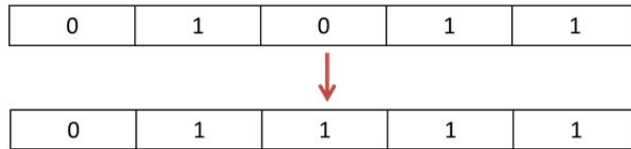
Figure 8. Mutation Operations on a Chromosome. Mutation operations choose one or two random alleles to flip in a chromosome vector. The resulting vector is then introduced into the set of most fit candidates for the next generation.
