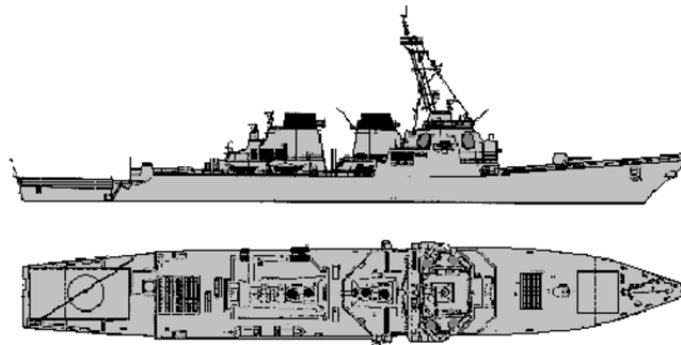
Figure 2. Arleigh-Burke Class Guided Missile Destroyers (DDG 51–119). These destroyers have up to 96 cells across eight installed modules in the aft part of the ship and four installed modules in the forward part of the ship. Source: FAS (2016b).
