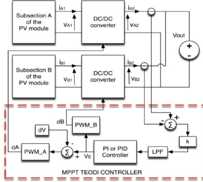
Figure 20. Topology of TEODI-Based MPPT Controller.
