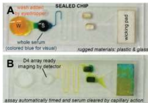
Fig. 5: Self-calibrating chip. (A-B) Sealed, self-clearing, assay chip made from cheap, rugged materials (laser-cut plastic & glass). Images immediately after addition of sample (S; whole serum) and at conclusion of assay. Wash (W) and sample colored with food coloring for ease of visualization . Assay automatically timed and goes to completion after addition of serum, based on capillary action.
