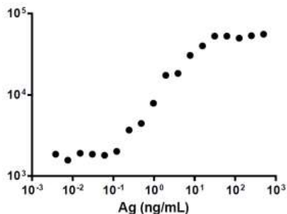
Fig 3: Analytical performance of D4 chips utilizing streptavidin-QD/biotin-dAb conjugates as labeling strategy, showing sub-nanogram/mL sensitivity.
