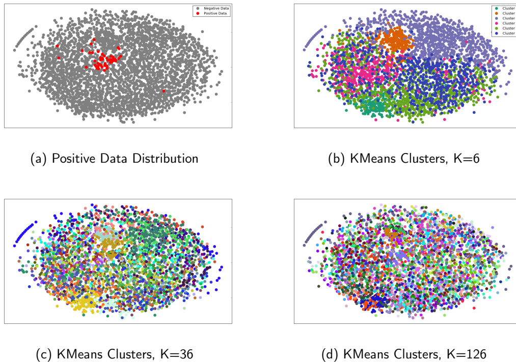
Figure 4.2. Document Clusters in TF-IDF Space.
