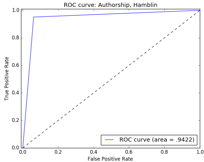
Figure 3.2. ROC Curve for Authorship Detection.
