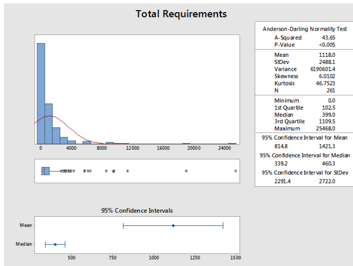
Figure 2: Functional Size
