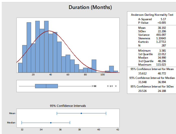
Figure 11: Duration
