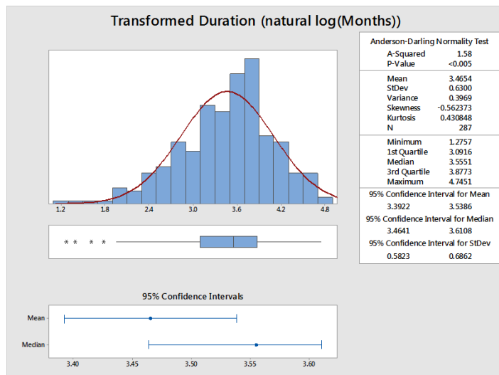
Figure 12: Duration, Normalized
