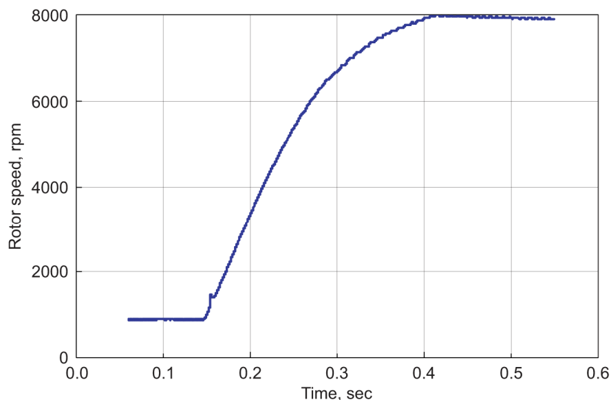
Figure 16.—Speed as a function of time for a fast acceleration.
