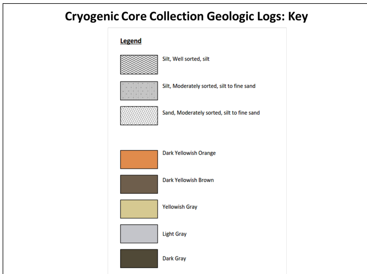
Figure 43g. Key for Geologic Logs.
