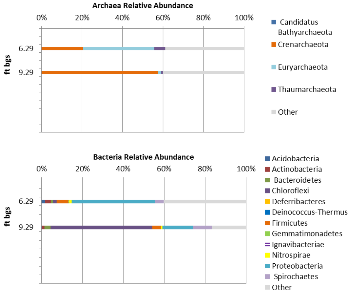
Figure G-13: Archaeal and Bacterial Community Composition of Subsamples Collected from Core DG2A: Phylum Level.
