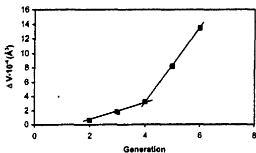
Figure 13. Volume change between neutral and low pH as a function of generation. Volumes were calculated as R_G assuming a spherical dendrimer model. Lines are added to show linear regions.
