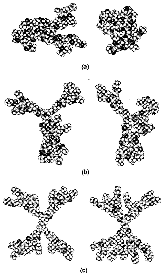
Figure 2. Final simulated configurations at (a) high, (b) neutral, and (c) low pH, starting from the initial configuration number one (left) and number two (right). Water molecules, explicitly included in the actual simulation, are not shown.
