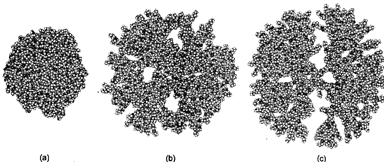
Figure 9. Final configuration of G6 PAMAM dendrimer after 100 ps MD simulations (a) at high pH (no amine is protonated), (b) at neutral pH (primary amines are protonated), and (c) at low pH (all amines are protonated).
