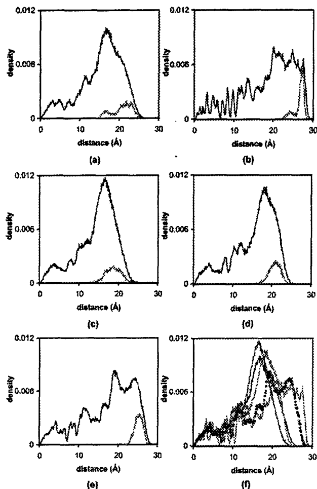
Figure 8. Atom densities (blue) and the densities of terminal nitrogen atoms (red) in G2 dendrimers at low pH. The nonbonded interaction conditions of models without explicit water molecules are (a) D = 1 and r_c = 11 Å, (b) D = 1 and r_c = \infty , (c) D = r and r_c = 11 Å, and (d) D = r and r_c = \infty . They are compared with (e) the results of simulation with water, which are the average values of results from ICN1 and ICN2. To improve the visual comparison, all density profiles of terminal nitrogen atoms are increased to 3 times their real value. The atom densities of all models are compared in (f): D = 1 and r_c = 11 Å (blue line), D = 1 and r_c = \infty (pink line), D = r and r_c = 11 Å (green line), D = r and r_c = \infty model (red line), and models with water molecules (purple circle).
