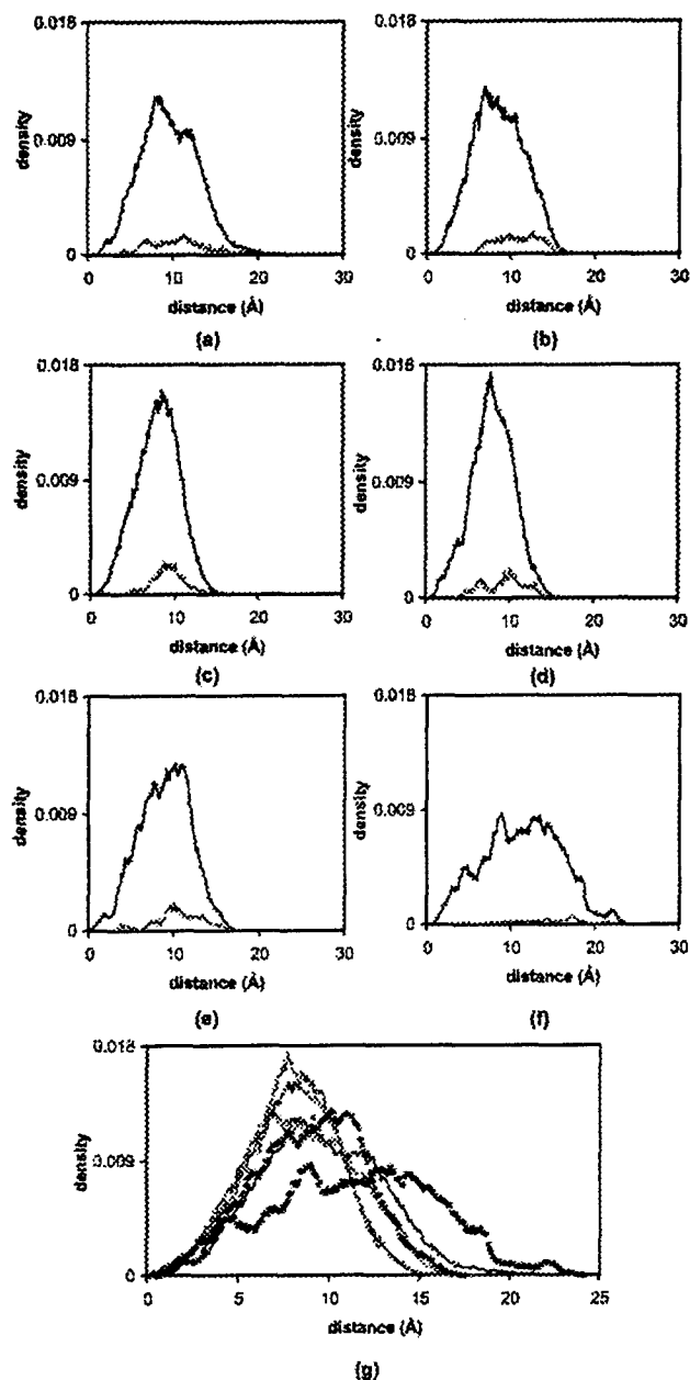
Figure 6. Atom densities (blue) and the densities of terminal nitrogen atoms (red) in G2 dendrimers at high pH. The nonbonded interaction conditions of models without explicit water molecules are (a) D = 1 and r_c = 11 Å, (b) D = 1 and r_c = \infty , (c) D = r and r_c = 11 Å, and (d) D = r and r_c = \infty . They are compared with the results of simulation with water from (e) ICN1 and (f) ICN2. To improve the visual comparison, all density profiles of terminal nitrogen atoms are increased to 3 times their real value. The atom densities of all models are compared in (g): D = 1 and r_c = 11 Å (blue line), D = 1 and r_c = \infty (pink line), D = r and r_c = 11 Å (green line), D = r and r_c = \infty (red line), ICN1 (purple circle), and ICN2 model (brown circle).
