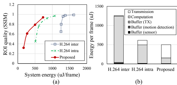
Fig. 10. (a) Quality-energy and (b) energy @ROI quality=0.8 of different rate controllers.
