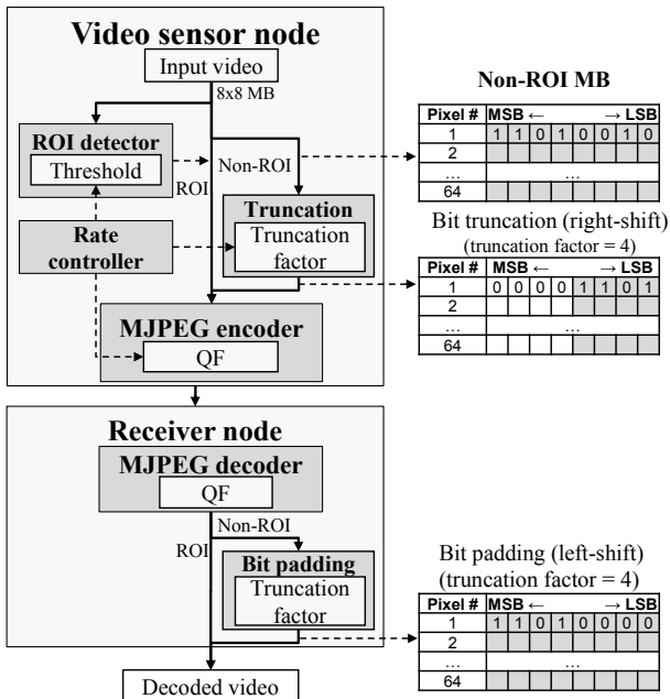
Fig. 6. Diagram of the proposed non-ROI bit truncation method.
