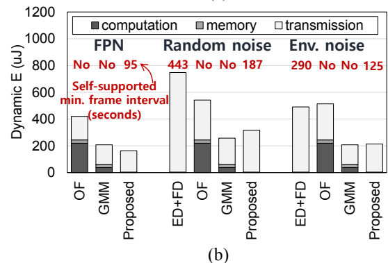
Fig. 11. (a) Data reduction and (b) system dynamic energy consumption through different moving object detection methods under noise.
