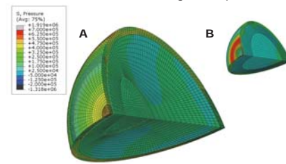
Fig. 3. Pressure during during blast loading for the (A) human and (B) baseline rat models.
