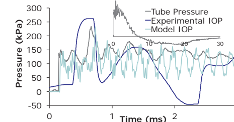
Fig. 4. IOP results compared to experimental IOP for initial peak. Tube pressure represents input to model. Peak IOP predicted by the model was within 12% of experimental data. Inset: Complete input pressure.
