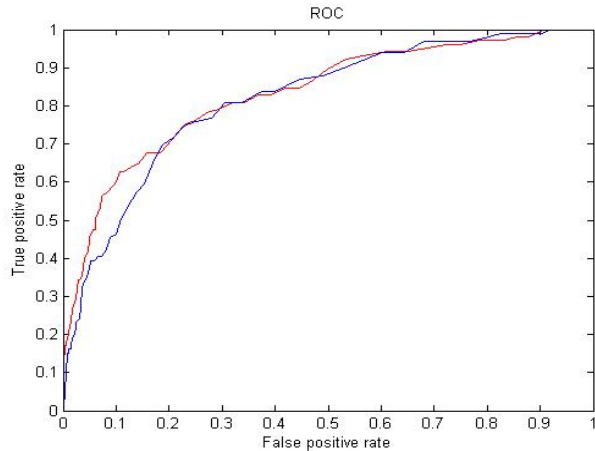
Figure 1. Receiver operating characteristics curve (ROC) analysis of ALT (blue) and SLT (red).
