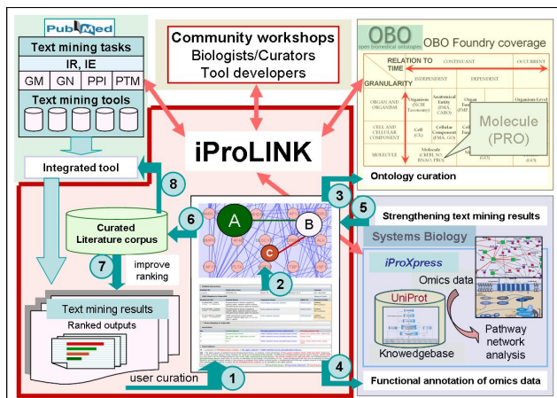
Figure 1. Overview of the iProLINK framework
