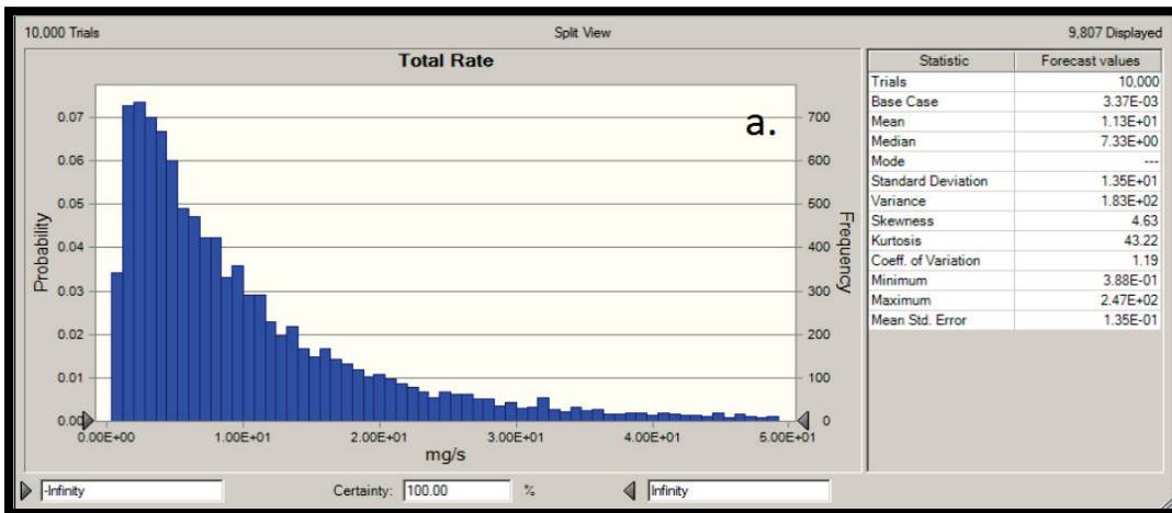
Figure 62. Explosive D total site release function distribution F' (F applied to the distribution of munitions at the site).
