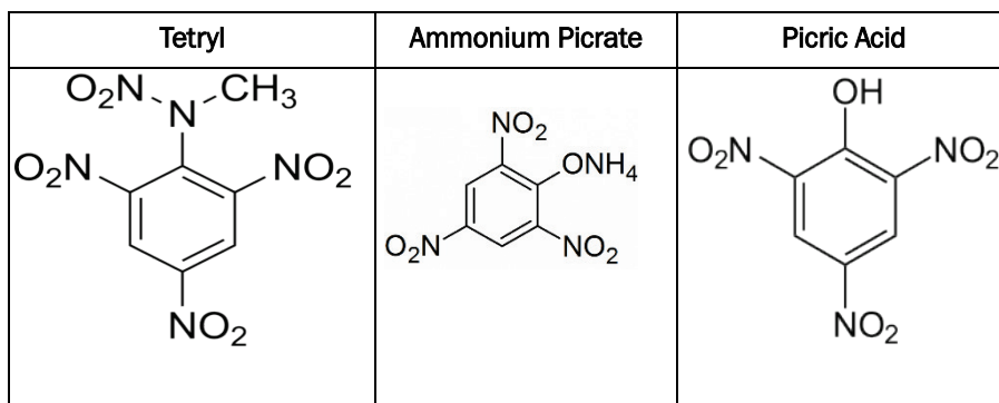
Figure 4. Chemical structure of tetryl, ammonium picrate (Explosive D), and picric acid.
