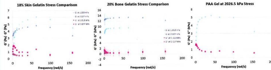
Figure 11: Dynamic shear for Bovine Skin Gelatin, Bovine Bone Gelatin and Polycrylamide (PAA) at a given applied stress. Error bars represent calculated standard error.
