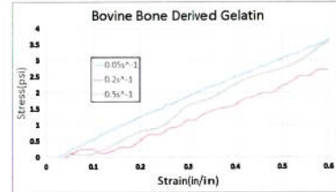
Figure 8: Average stress-strain curve for bovine bone-derived gelatin at three strain rates
