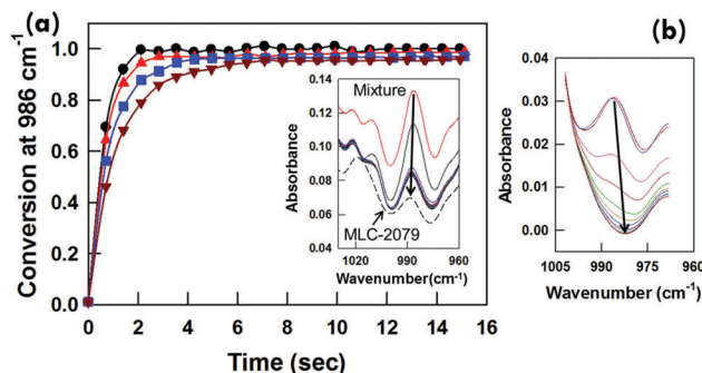
Fig. 4 (a) Normalized conversion of acrylate double bonds during the photopolymerization of 10 wt% RM82 initiated with 1 wt% I-369 with exposure to 365 nm UV light ranging from (▼) 70 \text{ mW cm}^{-2} , (■) 120 \text{ mW cm}^{-2} , (▲) 230 \text{ mW cm}^{-2} , and (●) 350 \text{ mW cm}^{-2} . The peak at 986 \text{ cm}^{-1} observable in PSCLCs prepared with (inset) MLC-2079 and (b) E7 decreases in magnitude during exposure of 350 \text{ mW cm}^{-2} intensity. The mixture was formulated by mixing 1 wt% I-369, 10 wt% RM82, 5 wt% R1011, and 84 wt% (a) MLC-2079 or (b) E7.
