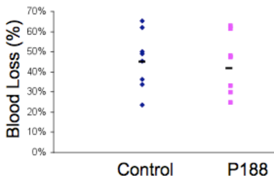
Figure 6. Effects of P188 on bleeding in uncontrolled hemorrhagic shock.
