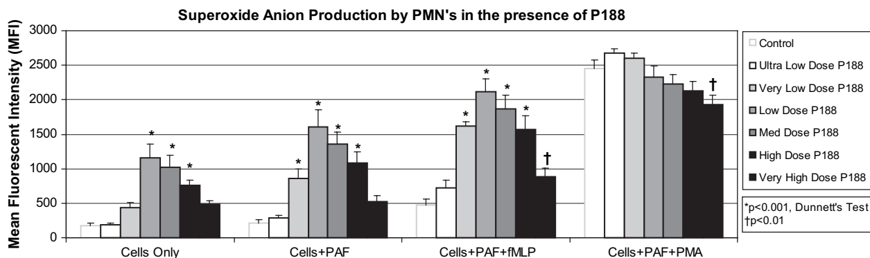
Fig 1. Superoxide anion production by PMNs in the presence of P188. After incubation with DHE and priming (PAF), P188 (in the following final doses: Ultra low dose: 0.005 mg/ml, very low dose: 0.05 mg/ml, low dose: 0.5 mg/ml, medium dose: 2.0 mg/ml, high dose: 6.0 mg/ml, very high dose: 15 mg/ml) was added to the human PMNs. Cells were then activated (fMLP or PMA). Mean fluorescent intensity (MFI), a surrogate for superoxide anion production, was measured by flow cytometry. Unstimulated, primed, and activated (with fMLP) PMNs exhibited increased superoxide anion production in the presence of P188 in a dose-dependent fashion. Among the maximally activated PMNs, addition of very high dose P188 reduced superoxide anion production.
