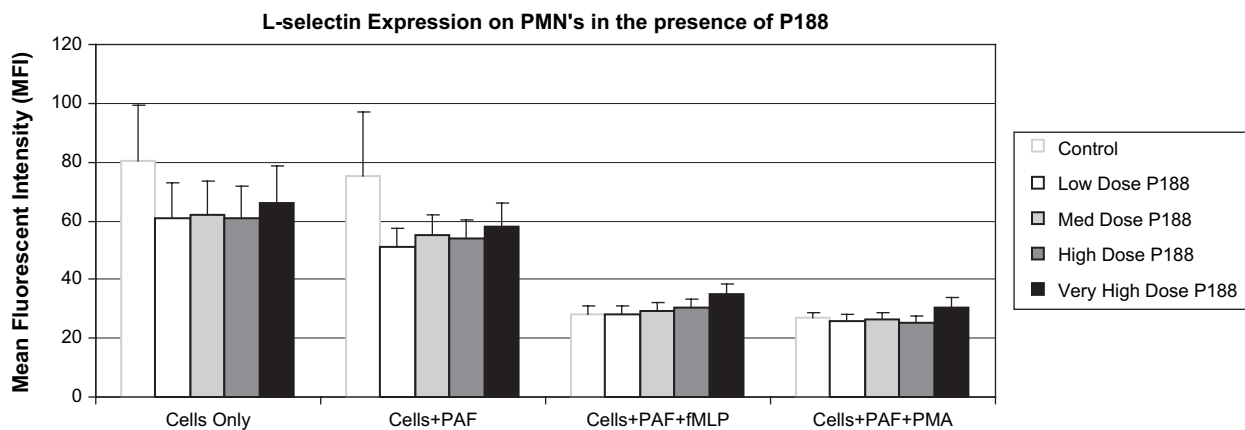
Fig 3. L-selectin expression on PMNs in the presence of P188. Incubation of the PMNs with P188 did not lead to any significant change in L-selectin expression, irrespective of dose used or stimulation status of the cells.
