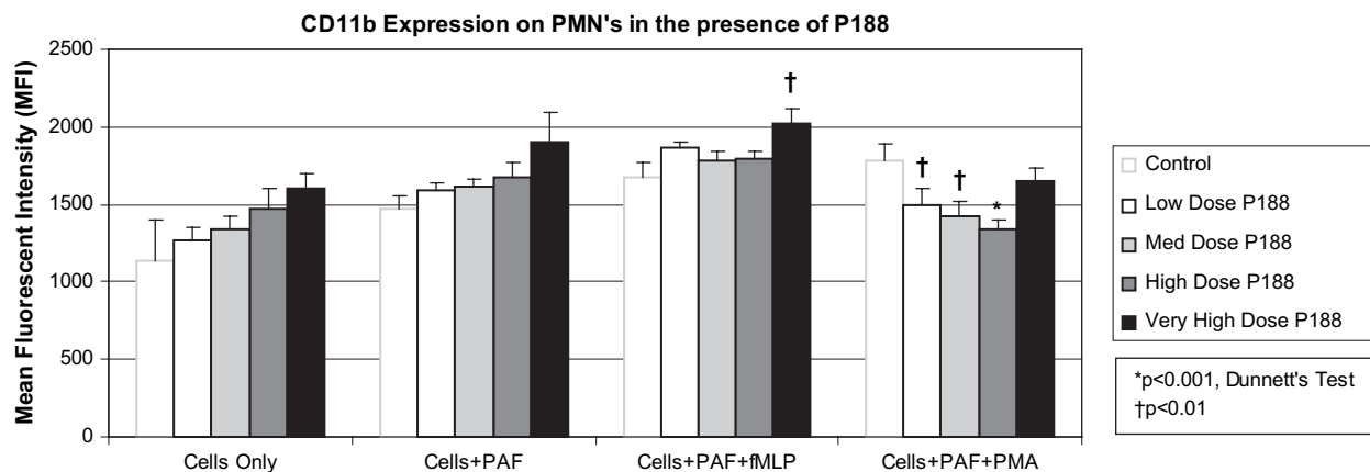
Fig 2. CD11b expression on PMNs in the presence of P188. After priming (PAF), P188 (in the following final doses: low dose: 0.5 mg/ml, medium dose: 2.0 mg/ml, high dose: 6.0 mg/ml, very high dose: 15 mg/ml) was added to the human PMNs. Cells were then activated (fMLP or PMA) and PE conjugated antibodies specific for human CD11b antibodies were added. Mean fluorescent intensity (MFI), a surrogate for CD11b marker expression, was measured by flow cytometry. Among unstimulated or primed PMNs, P188 did not alter CD11b marker expression. Primed and activated (fMLP) PMNs increased CD11b expression in the presence of very high dose P188. Primed and activated (PMA) PMNs decreased CD11b expression in the presence of low, medium, and high dose P188.
