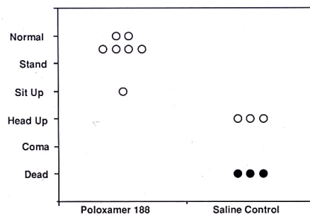
Figure 2. Neurologic Function Following DHCA. Beagle dogs were subjected to 2.5 hours of DHCA with or without P188 and were then monitored for 7 days. Each symbol represents the neurologic status of one dog at the end of the study. P188 protected brain function in a highly significant fashion in that the worst dog treated with P188 was better than the best control (6).
