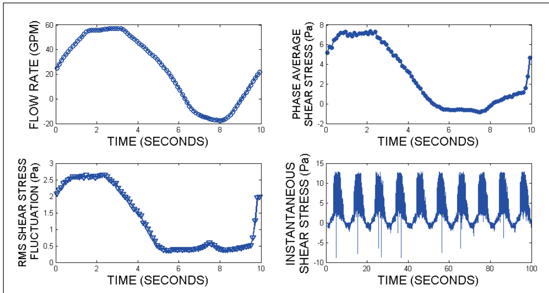
Figure A6. Shear-stress results for operating condition 50_10_open_on.
