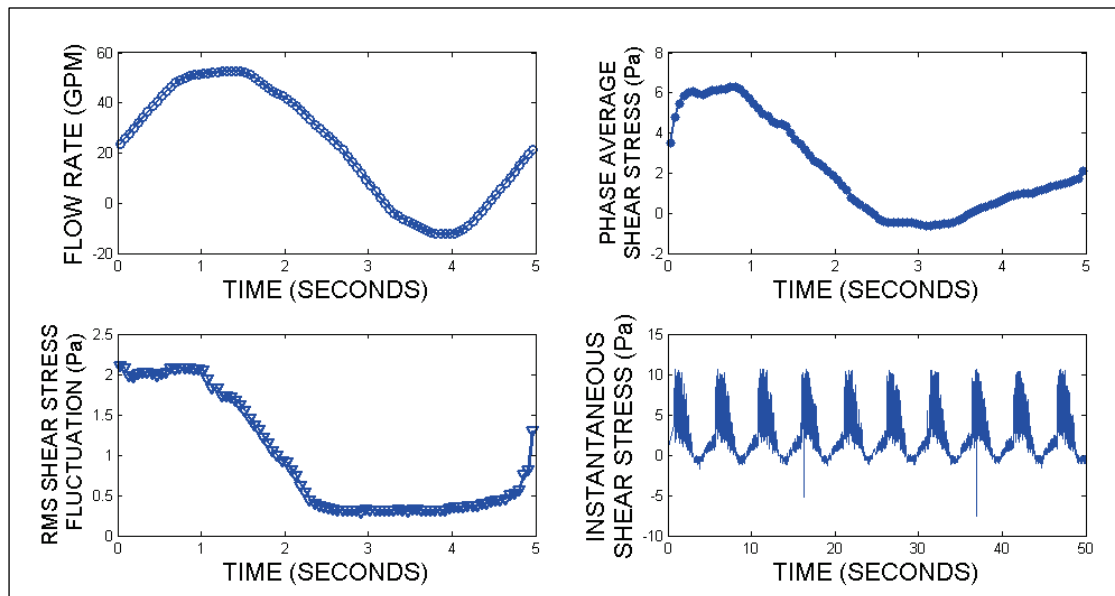
Figure A22. Shear-stress results for operating condition 50_5_open_on.
