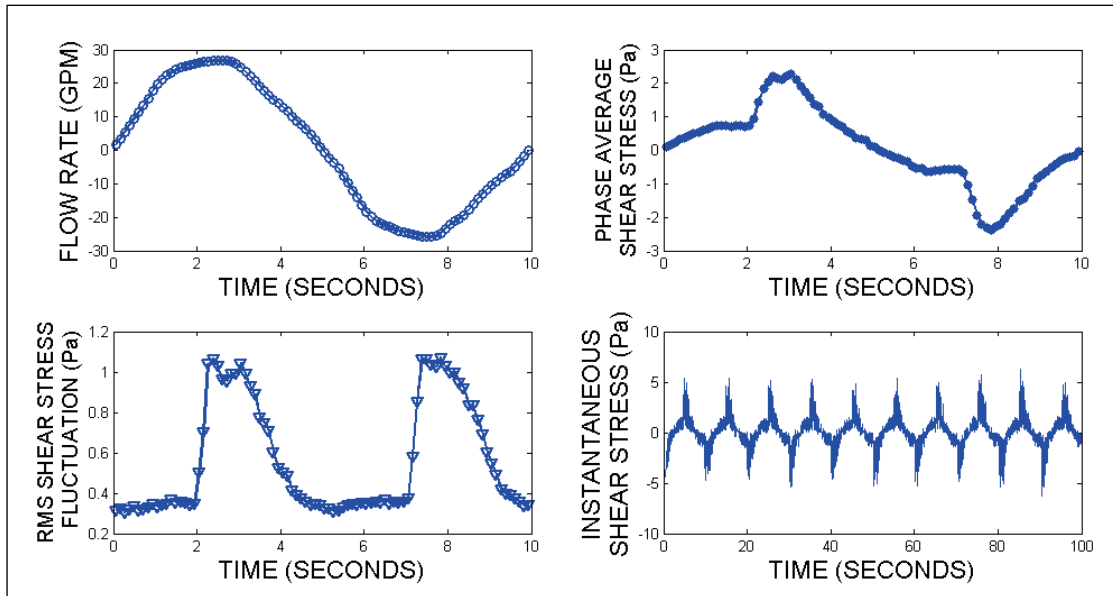
Figure 30. Phase-averaged data for operating condition 40_10_open_off.
