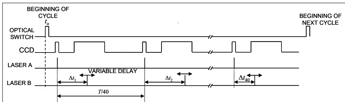
Figure 7. Timing diagram for PIV measurements in oscillating flow.
