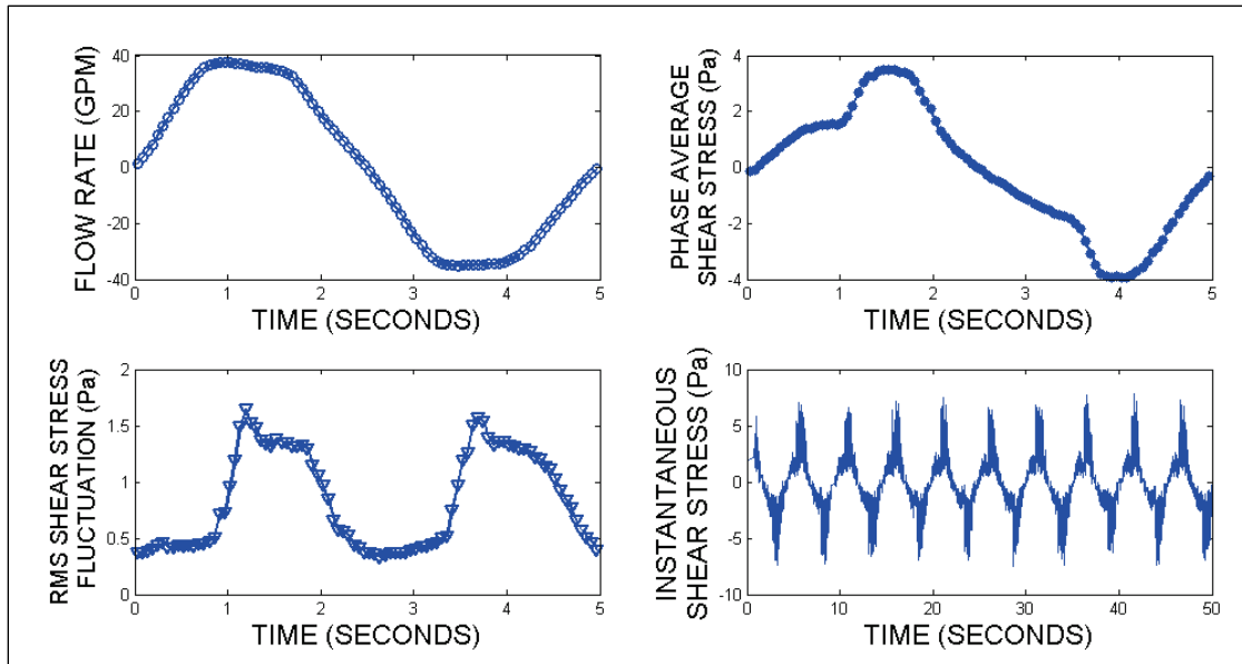
Figure A21. Shear-stress results for operating condition 40_5_60_off.
