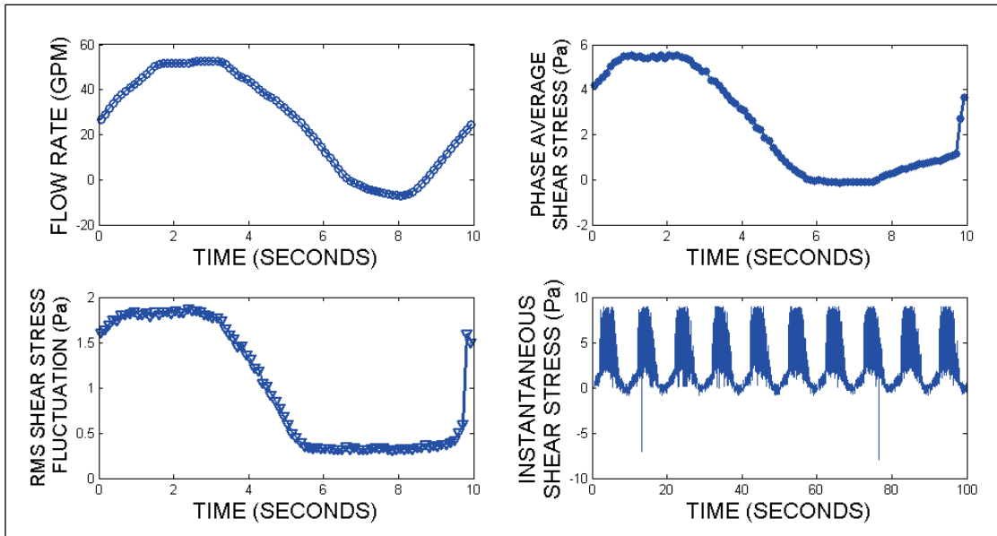
Figure A15. Shear-stress results for operating condition 40_10_open_on.
