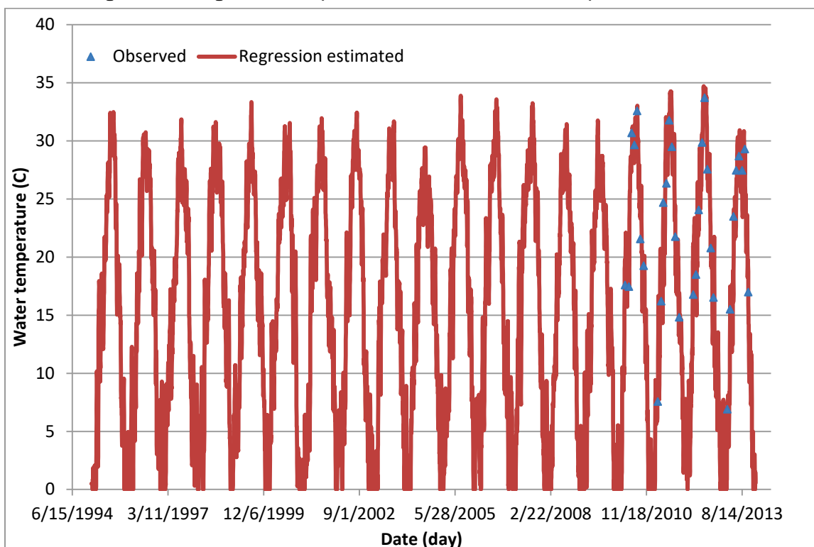
Figure C17. Regression computed versus observed water temperatures at BC17.
