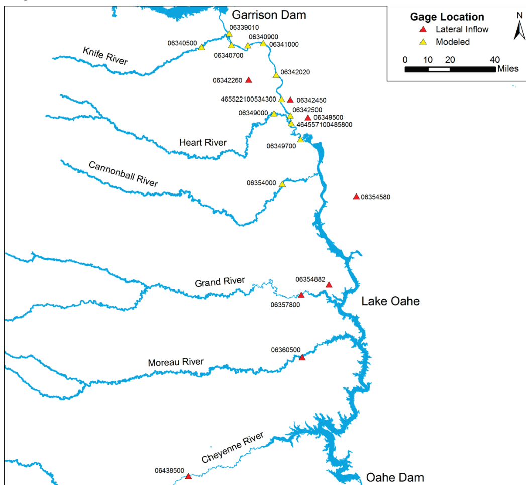
Figure 21. HEC-RAS model extent for the Garrison Dam to Oahe Dam reach (USACE 2015).
