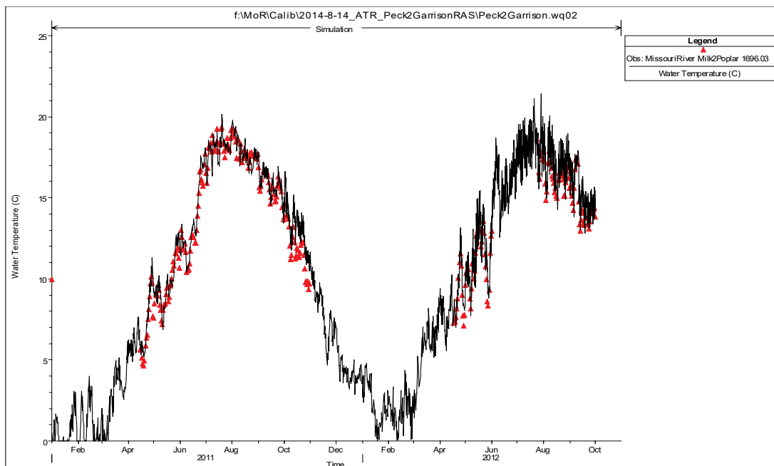
Figure 17. HEC-RAS predicted versus observed water temperatures of the Missouri River at Wolf, MT.
