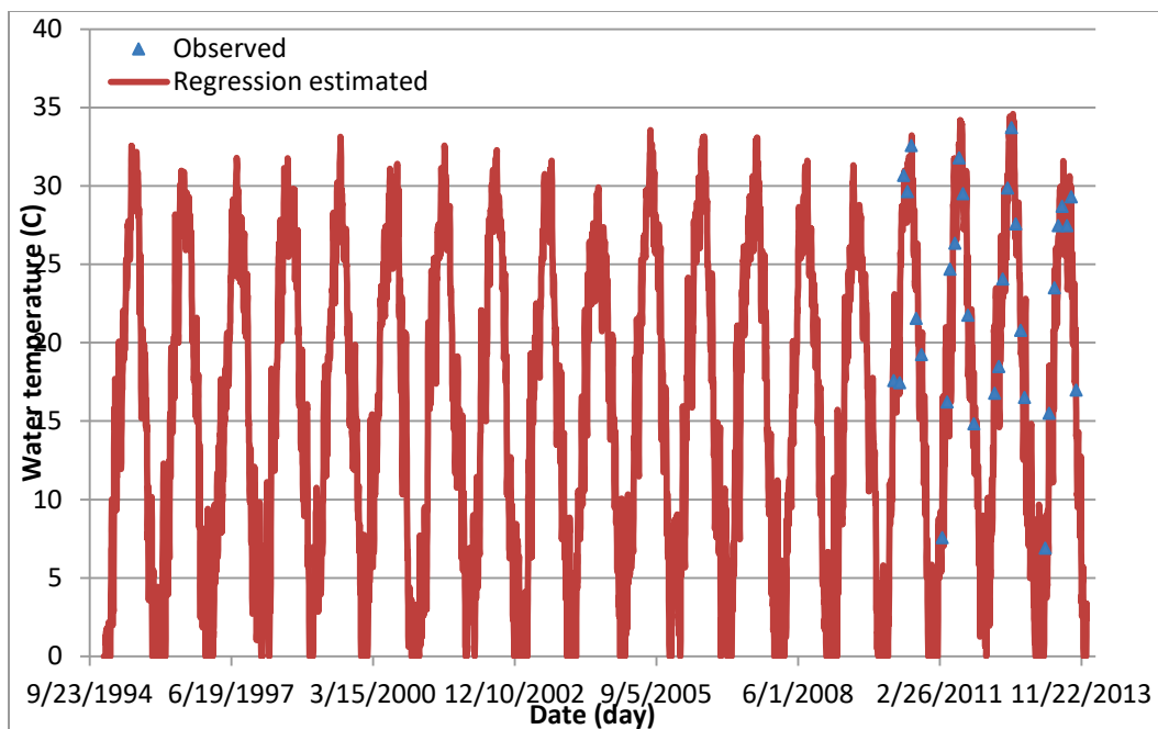
Figure C23. Regression computed versus observed water temperatures at BC23.
