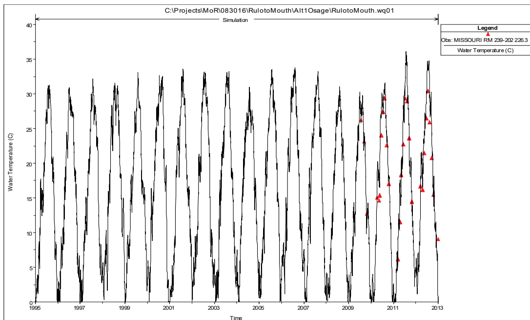
Figure 44. HEC-RAS predicted versus observed water temperatures of the Missouri River at Gasgaw, MO (USGS 06906500).
