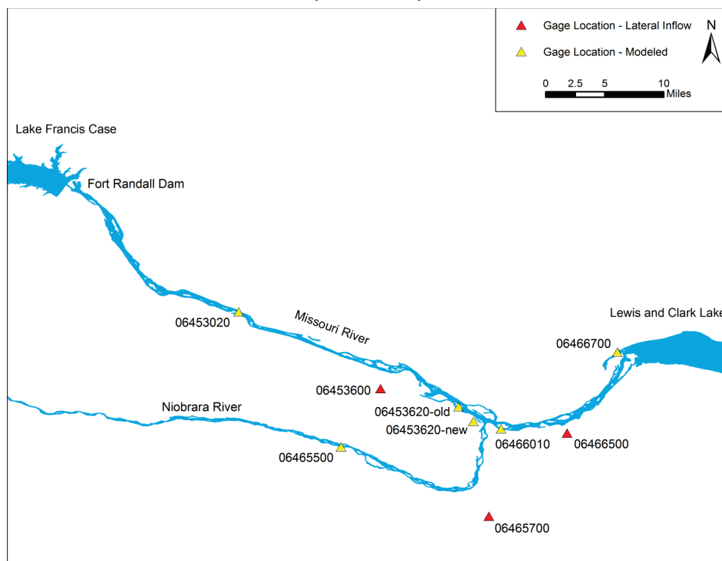
Figure 26. HEC-RAS model extent for the Fort Randall Dam to Gavins Point Dam reach (USACE 2015).
