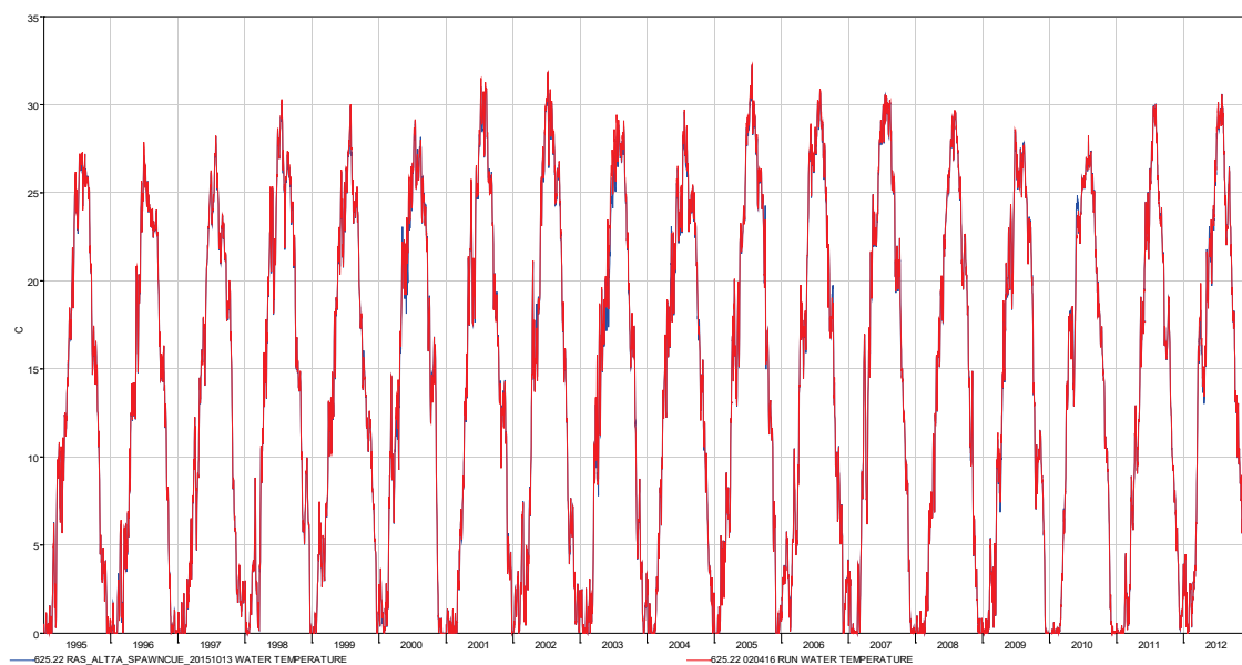
Figure 47. Model predicted daily mean water temperatures at Missouri River RM 625.22 for alternatives 1 and 7.
