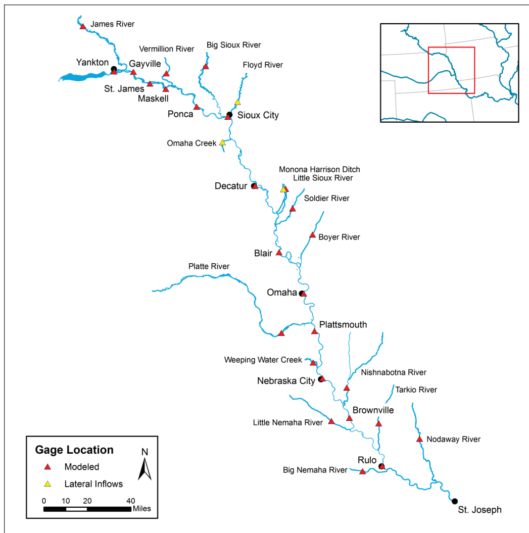
Figure 28. HEC-RAS model extent for the Gavins Point Dam to Rulo reach (USACE 2015).
