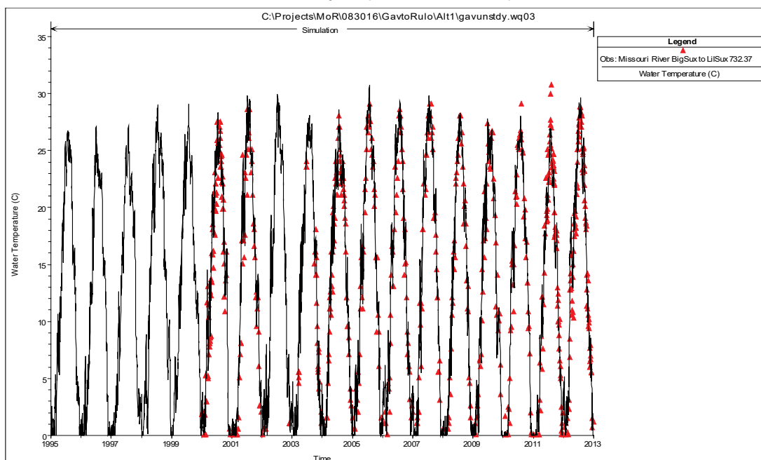
Figure 33. HEC-RAS predicted versus observed water temperatures of the Missouri River at Sioux City, IA (USGS 06486000).
