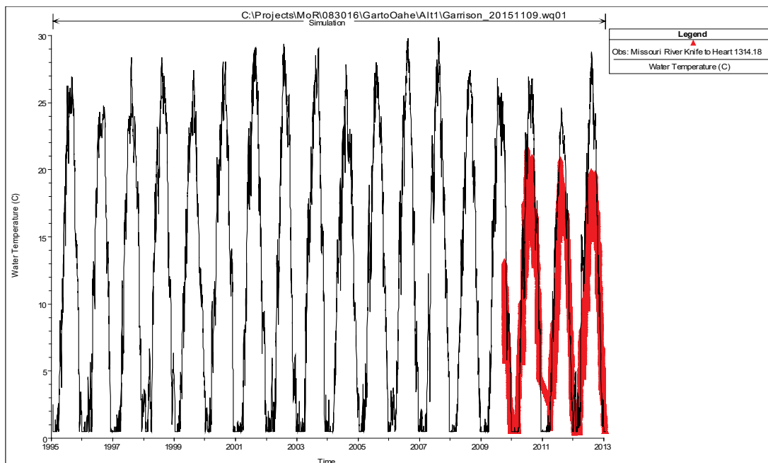
Figure 25. HEC-RAS predicted versus observed water temperatures of the Missouri River at Bismarck, ND (USGS 06342500).
