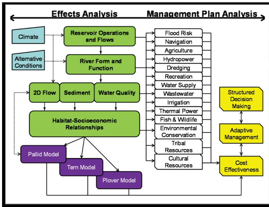
Figure 1. Missouri River modeling framework for the effects analysis and the management plan analysis (Fischenich et al. 2014).
