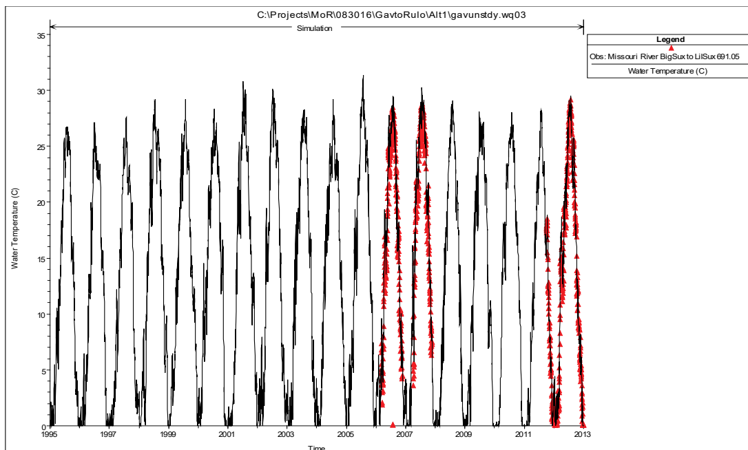
Figure 34. HEC-RAS predicted versus observed water temperatures of the Missouri River at Decatur, NE (USGS 06601200).
