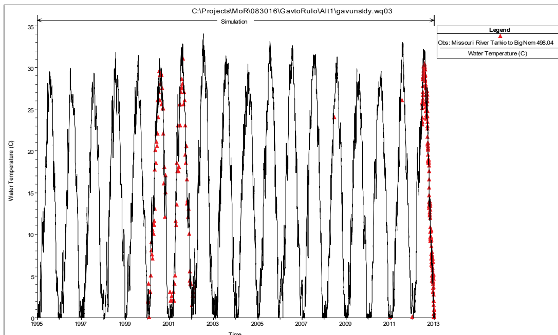
Figure 37. HEC-RAS predicted versus observed water temperatures of the Missouri River at Rulo, NE (USGS 06813500).
