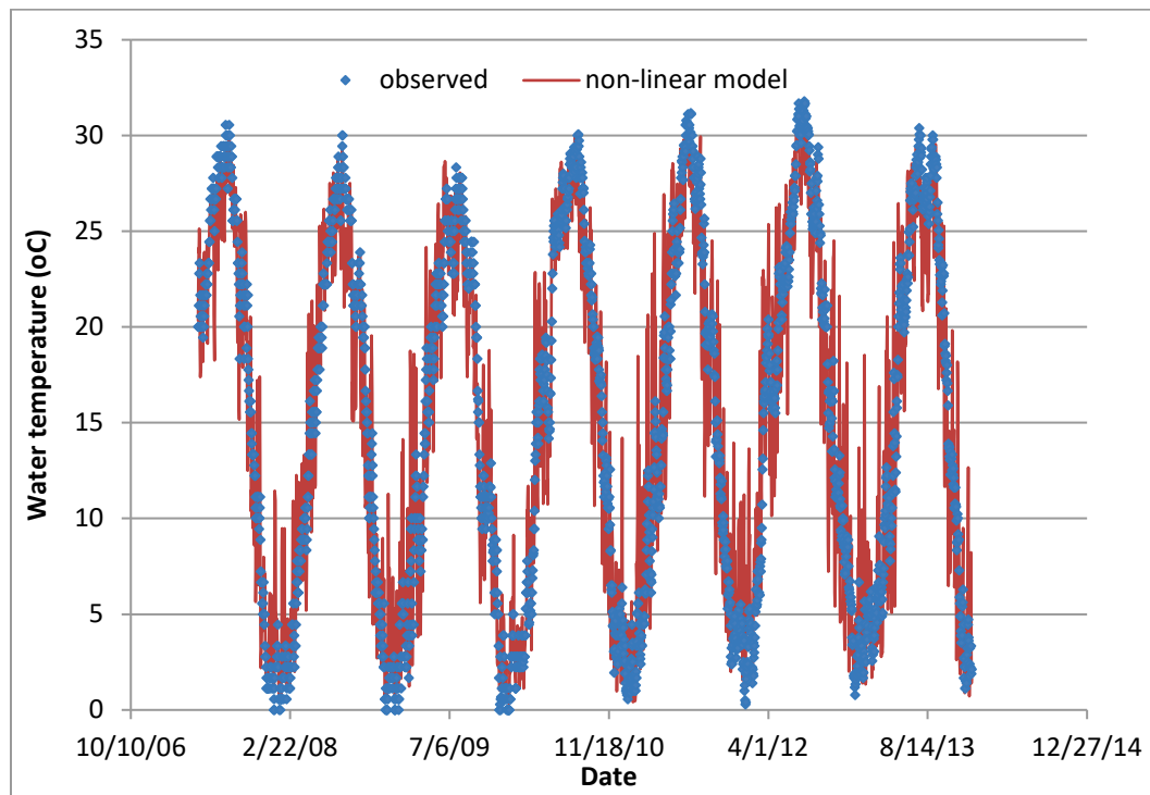
Figure 11. Observed vs regression computed water temperatures at USGS 0689300.
