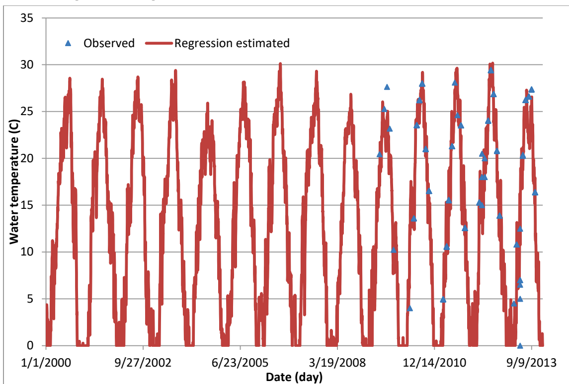
Figure C10. Regression computed versus observed water temperatures at BC10.
