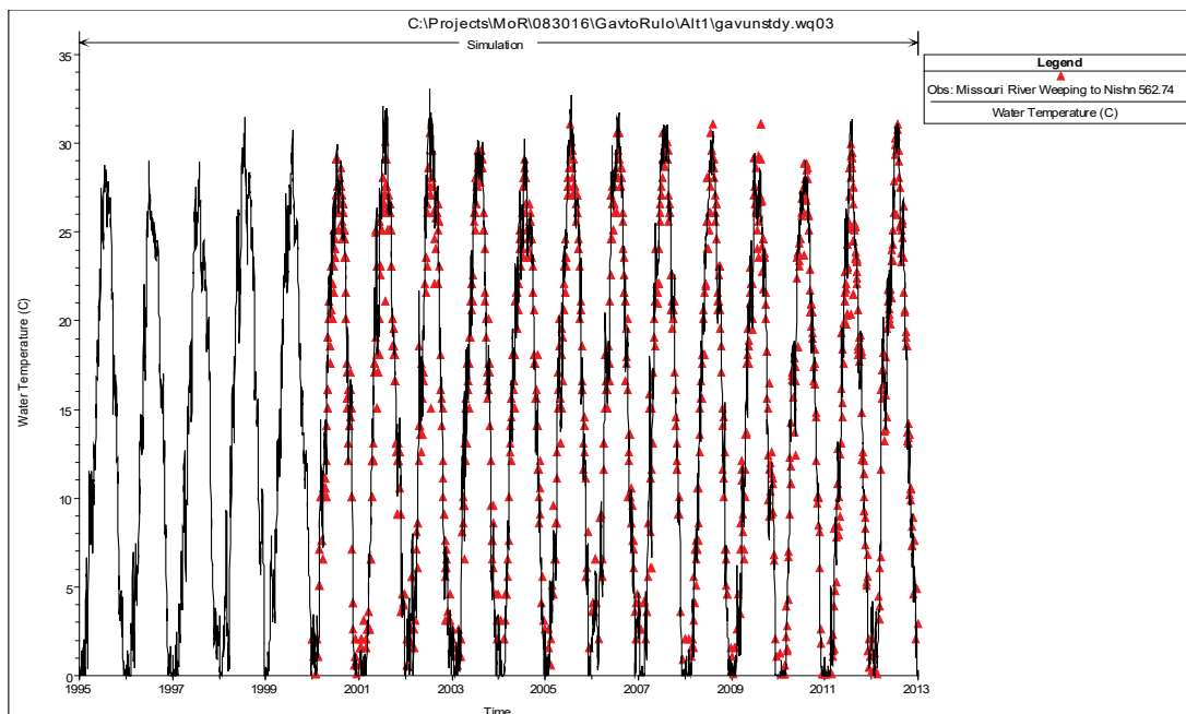
Figure 36. HEC-RAS predicted versus observed water temperatures of the Missouri River at Nebraska City, NE (USGS 06807000).
