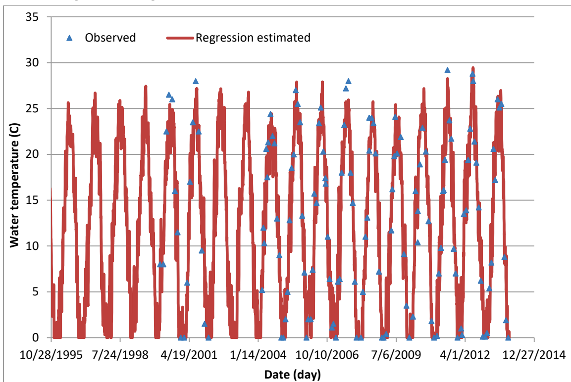
Figure B14. Regression computed versus observed water temperatures at BC14.
