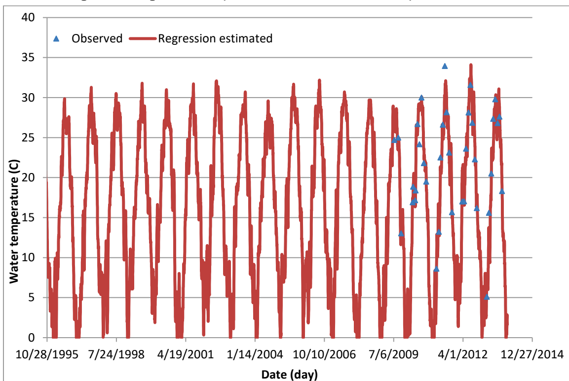
Figure B7. Regression computed versus observed water temperatures at BC7.
