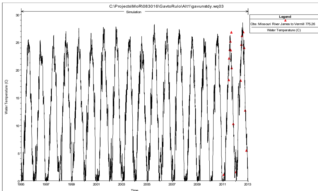
Figure 32. HEC-RAS predicted versus observed water temperatures of the Missouri River near Maskell, NE (USGS 06478526).
