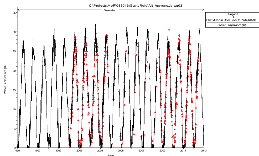
Figure 35. HEC-RAS predicted versus observed water temperatures of the Missouri River at Omaha, NE (USGS 06610000).
