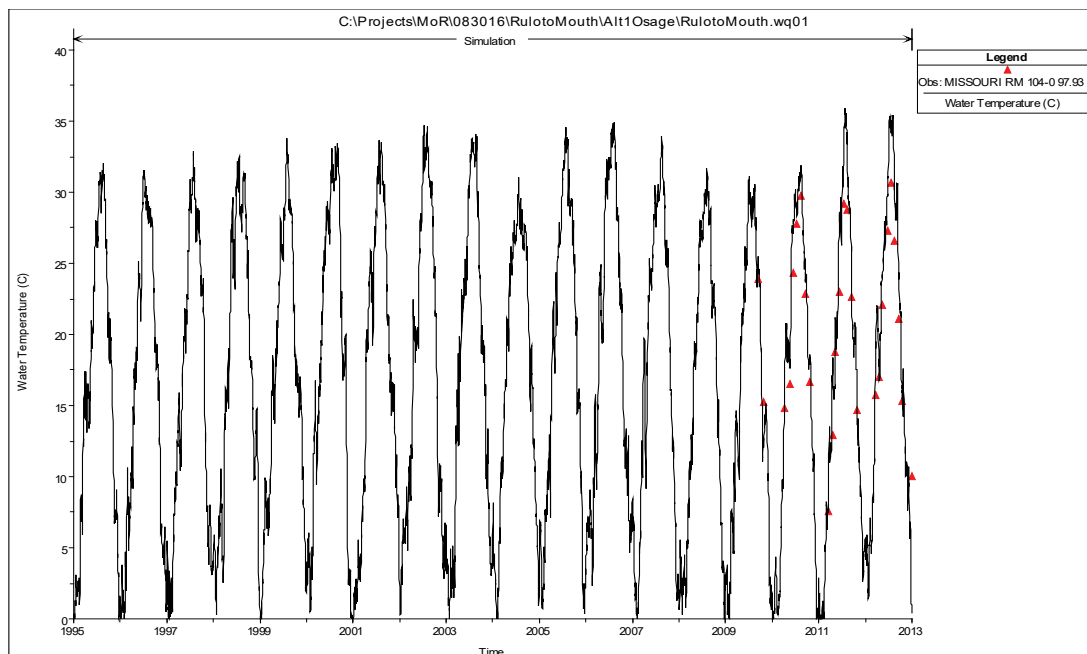
Figure 45. HEC-RAS predicted versus observed water temperatures of the Missouri River at Hermann, MO (USGS 06934500).
