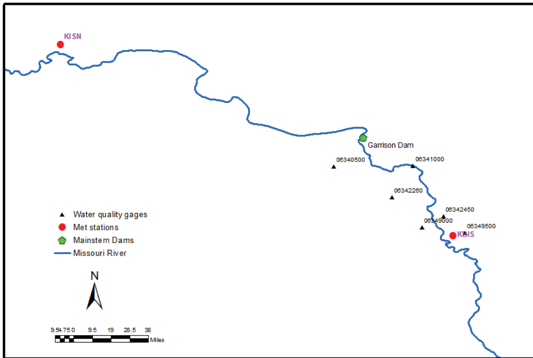
Figure 13. Water quality monitoring gages and correlated meteorological stations for the Garrison Dam to Oahe Dam reach.
