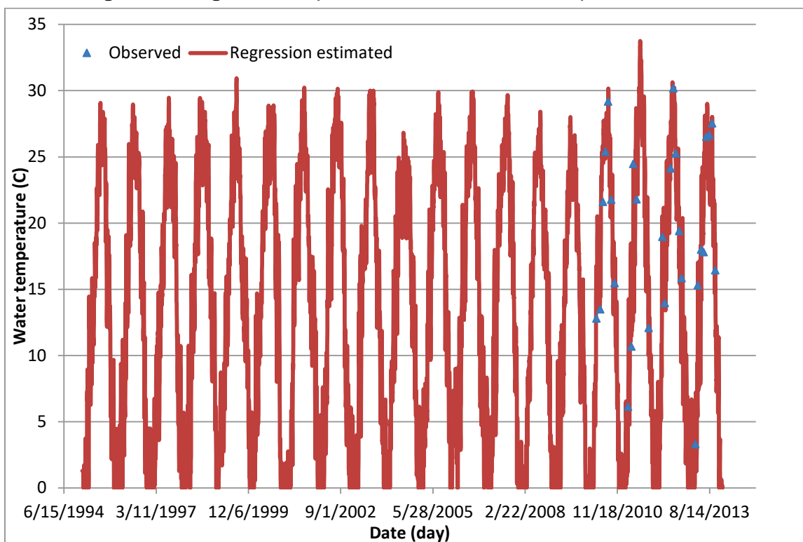
Figure C19. Regression computed versus observed water temperatures at BC19.
