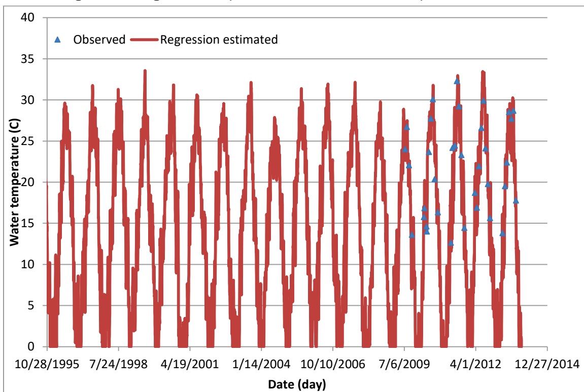
Figure C13. Regression computed versus observed water temperatures at BC13.
