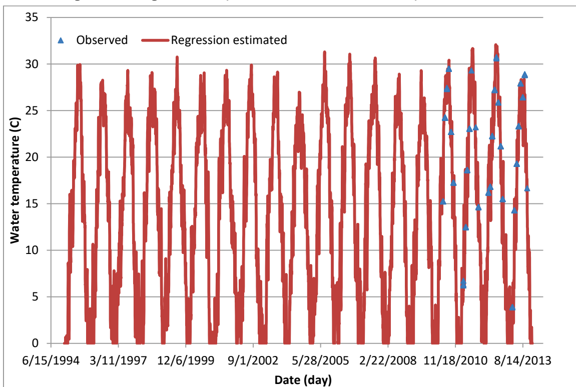
Figure C15. Regression computed versus observed water temperatures at BC15.
