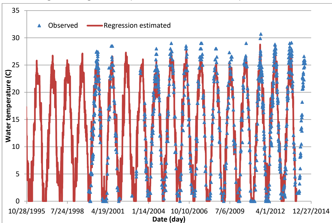
Figure B9. Regression computed versus observed water temperatures at BC9.
