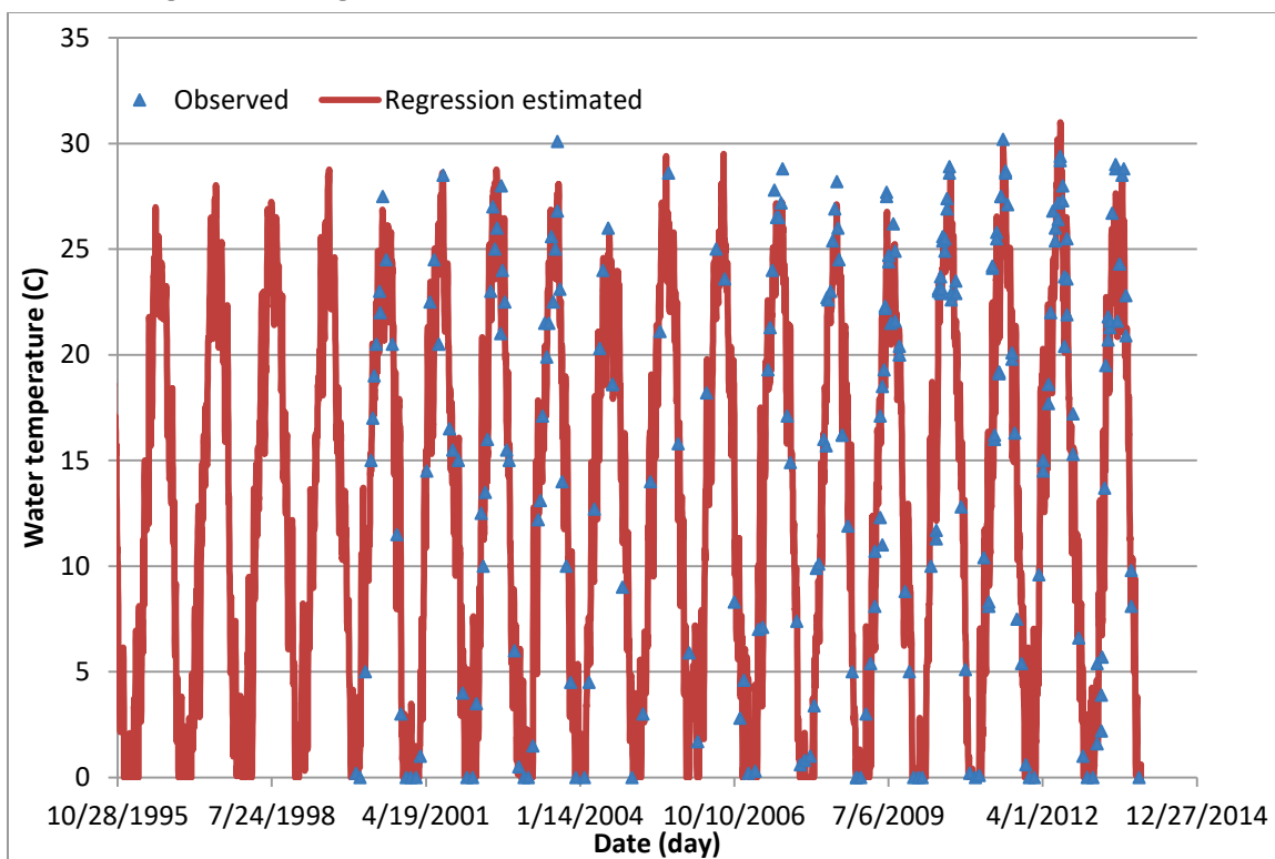
Figure B12. Regression computed versus observed water temperatures at BC12.
