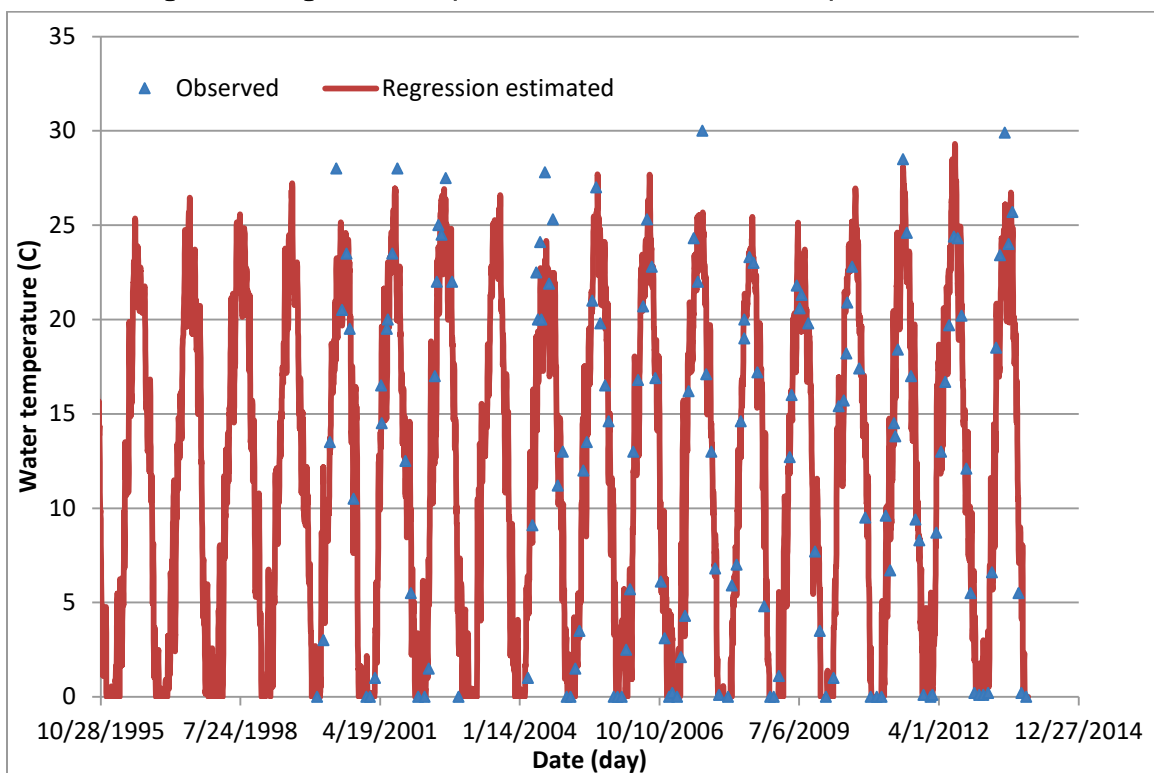
Figure B3. Regression computed versus observed water temperatures at BC3.
