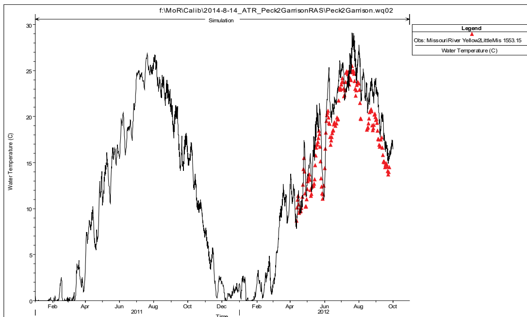
Figure 20. HEC-RAS predicted versus observed water temperatures of the Missouri River at Williston, MT.
