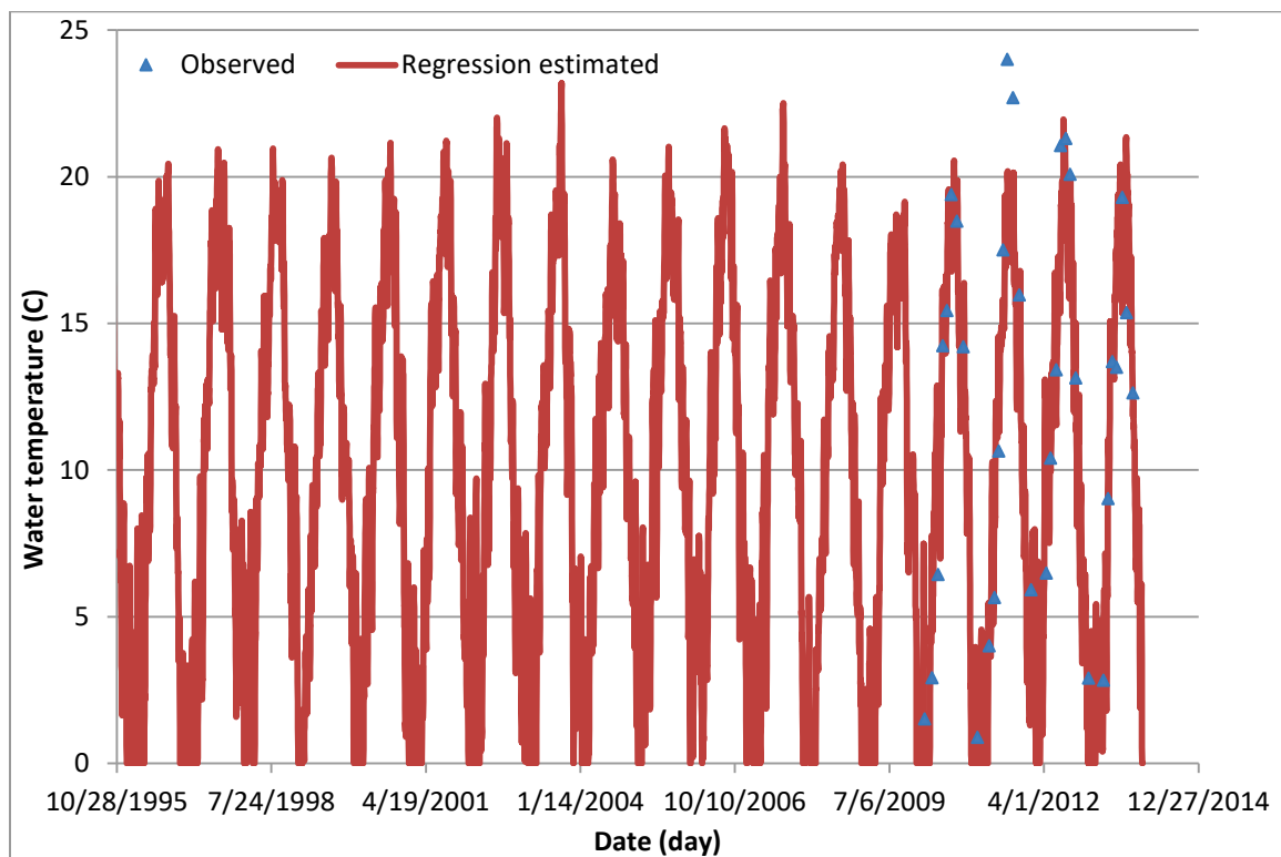
Figure A1. Regression computed versus observed water temperatures at BC1.
