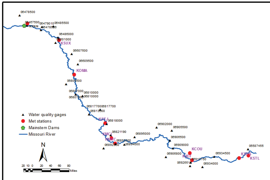
Figure 14. Water quality monitoring gages and correlated meteorological stations for the lower Missouri River from the Givens Point Dam to the mouth of the Missouri River.
