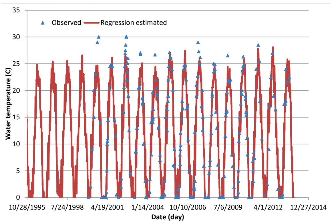
Figure B2. Regression computed versus observed water temperatures at BC2.
