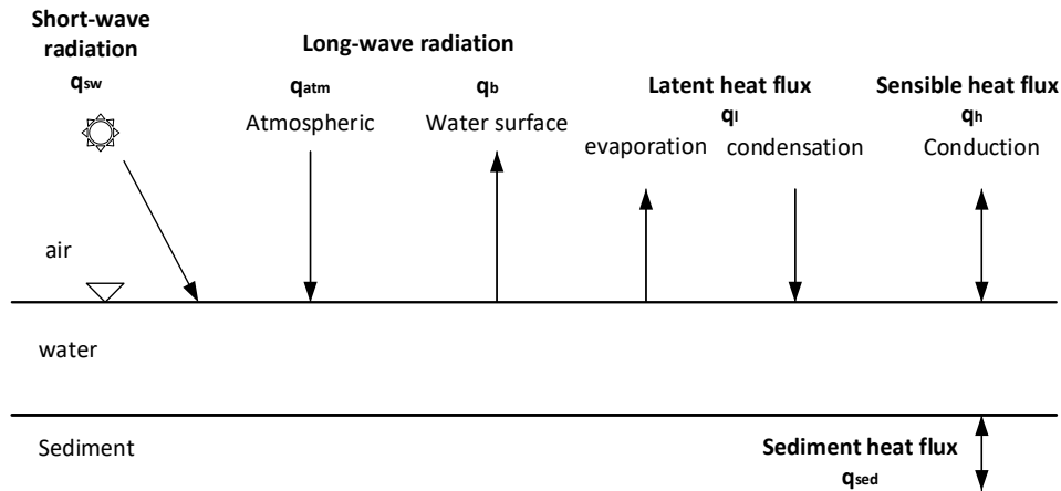
Figure 3. Sources and sinks of heat energy at the atmospheric and sediment interfaces (Deas and Lowney 2000).
