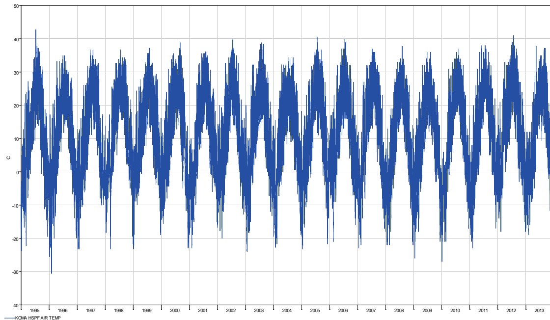
Figure 6. Hourly air temperature at KOMA, NE.
