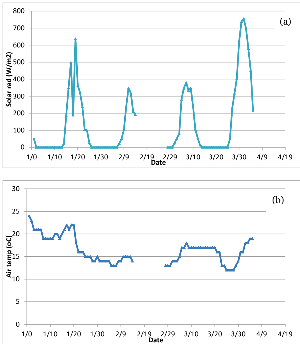
Figure 5. Data gaps of observed hourly (a) solar radiation and (b) air temperature at KOMA, NE.
