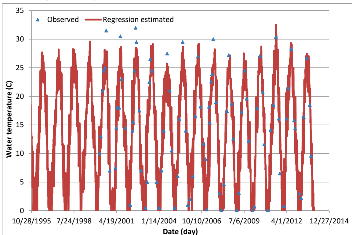
Figure B15. Regression computed versus observed water temperatures at BC15.
