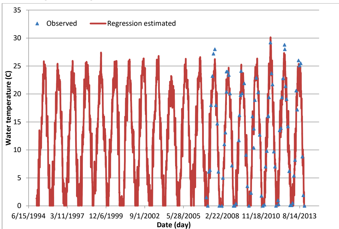
Figure C18. Regression computed versus observed water temperatures at BC18.
