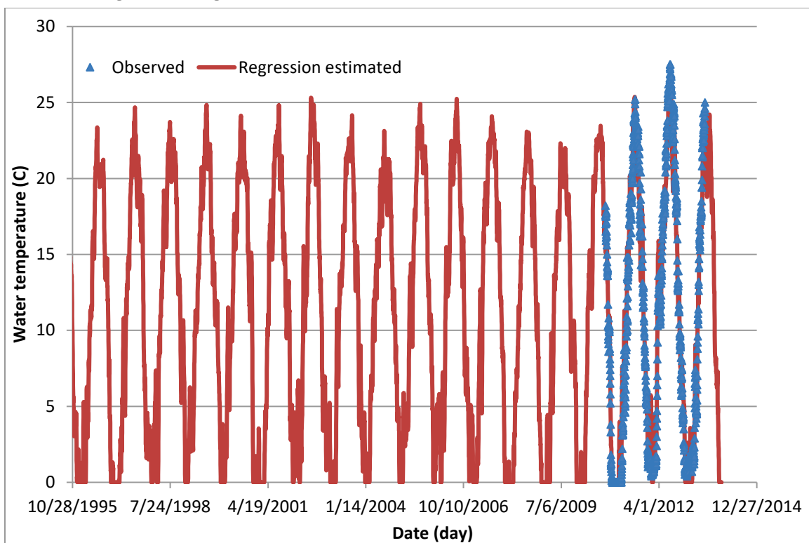
Figure B6. Regression computed versus observed water temperatures at BC6.
