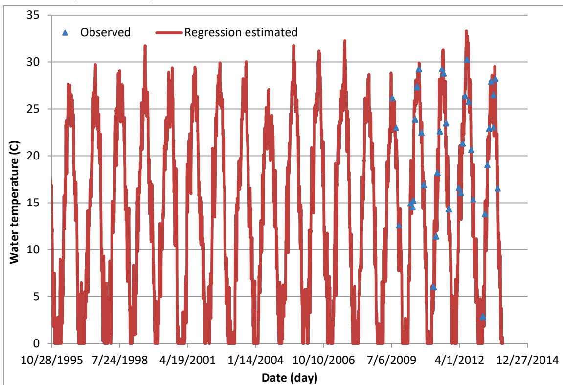
Figure C14. Regression computed versus observed water temperatures at BC14.
