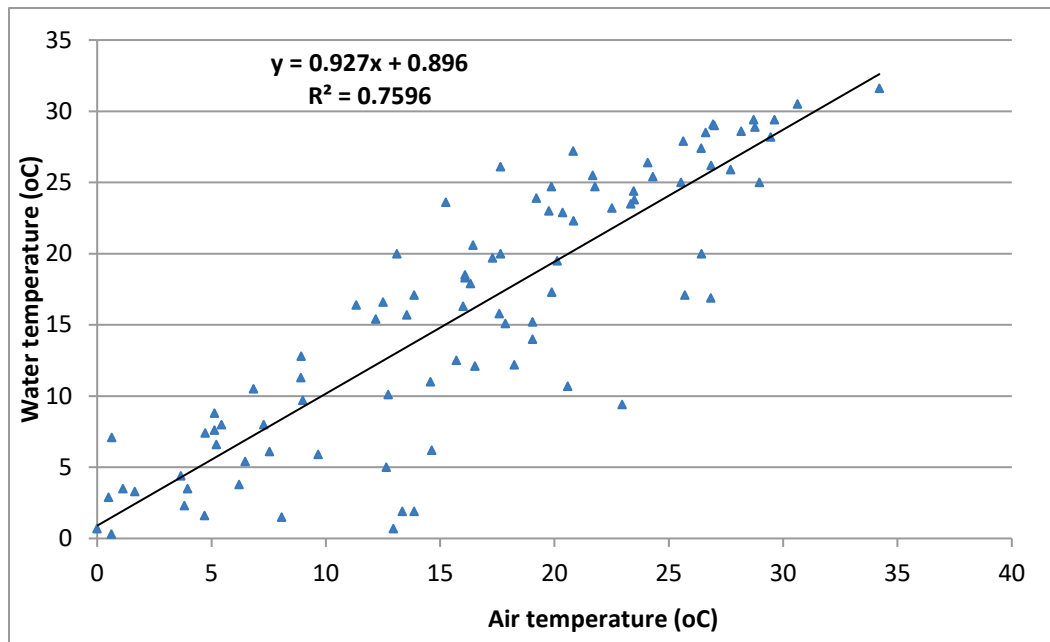
Figure 9. Scatter plot of observed water versus air temperatures at USGS 05587455.
