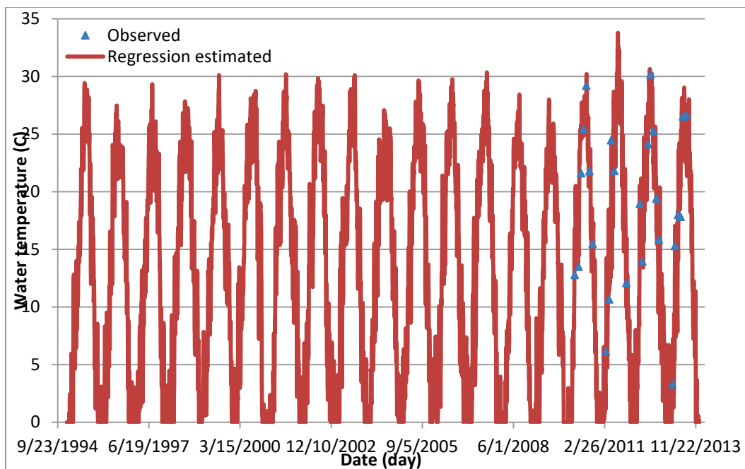
Figure C25. Regression computed versus observed water temperatures at BC25.
