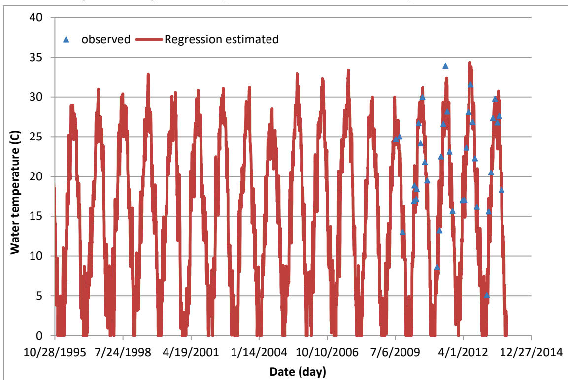
Figure C7. Regression computed versus observed water temperatures at BC7.
