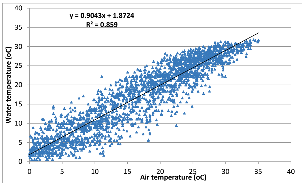
Figure 7. Scatter plot of observed water versus air temperatures at USGS 0689300.
