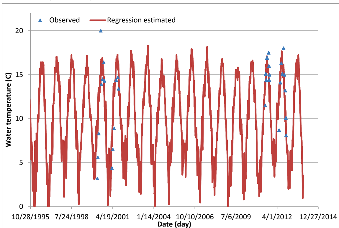
Figure A5. Regression computed versus observed water temperatures at BC5.
