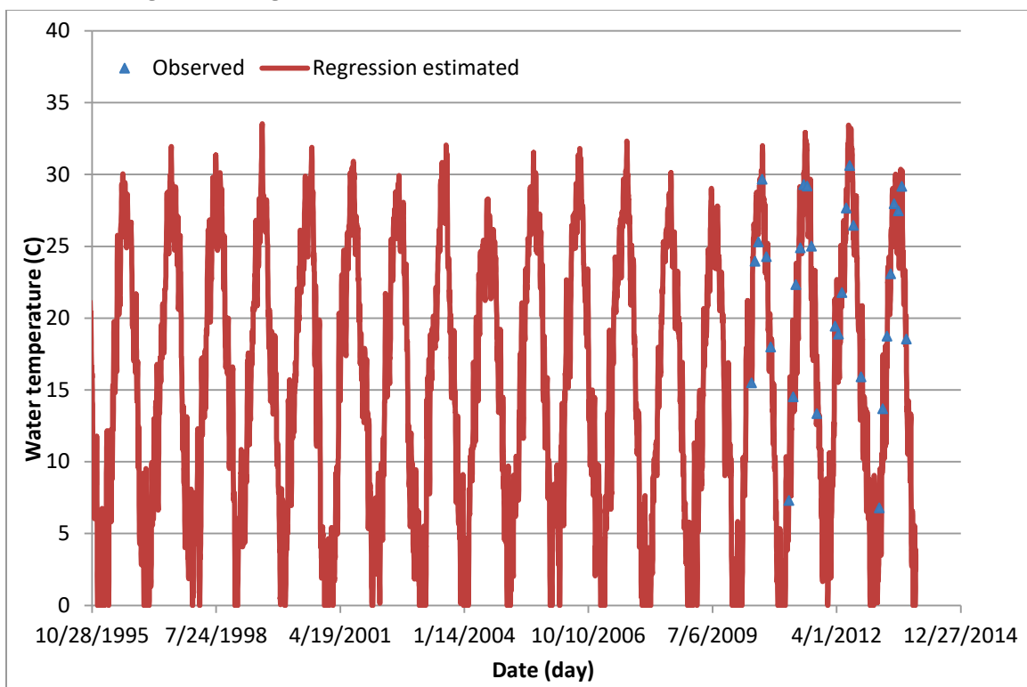
Figure C6. Regression computed versus observed water temperatures at BC6.
