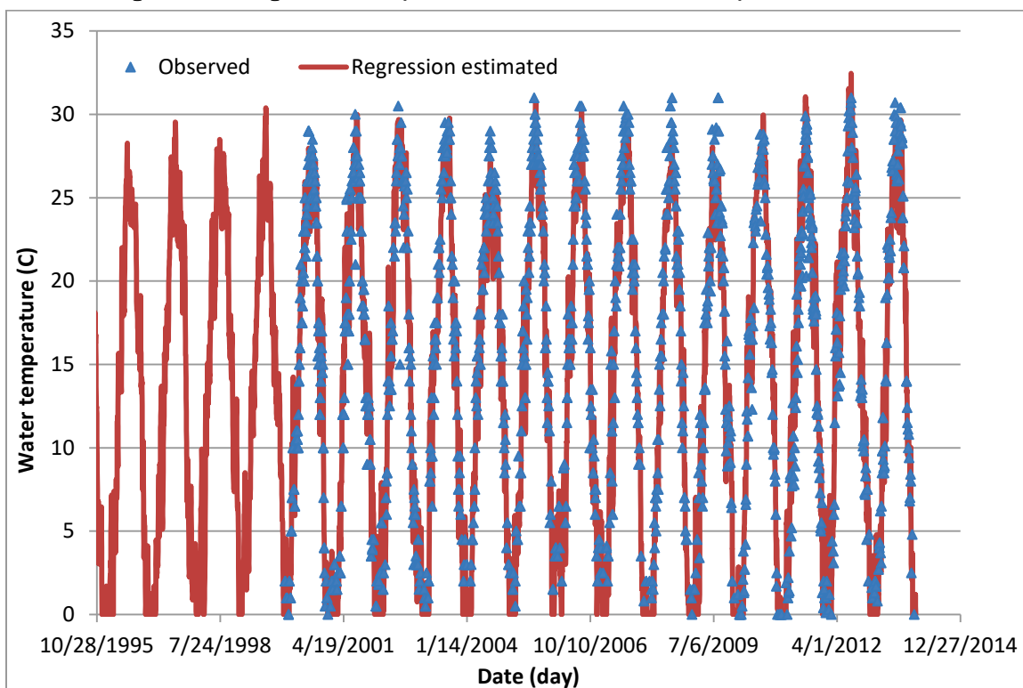
Figure B13. Regression computed versus observed water temperatures at BC13.
