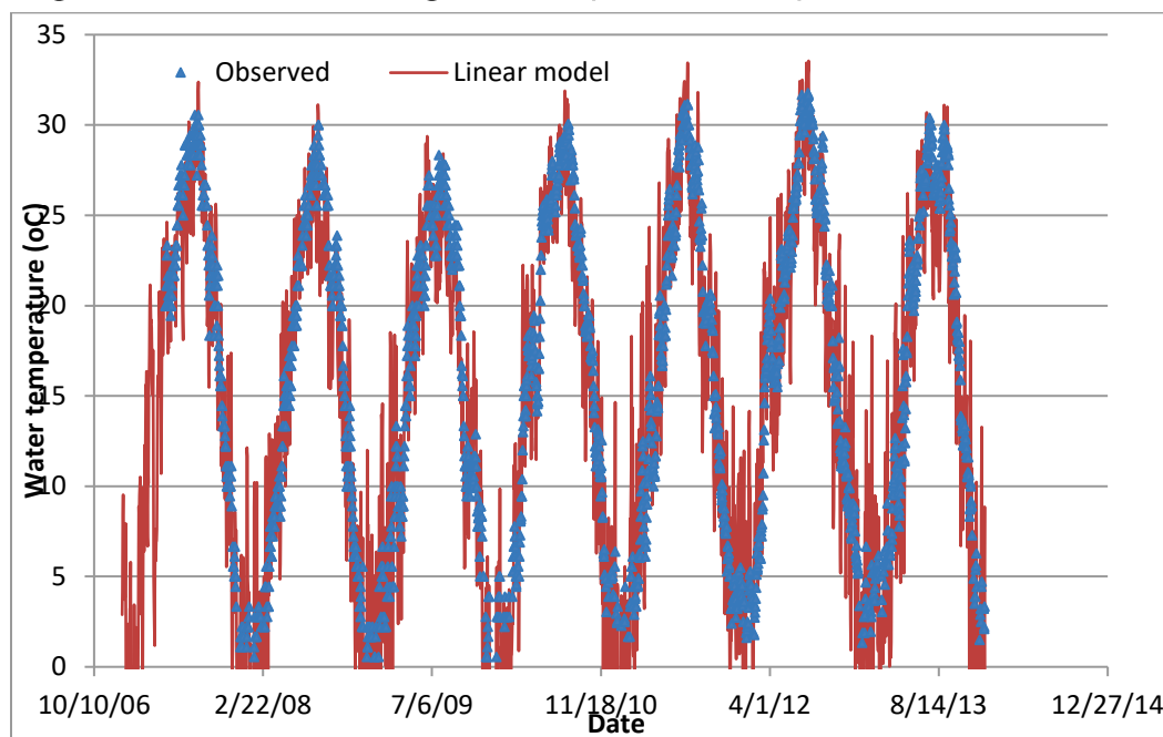
Figure 8. Observed vs. linear-regression-computed water temperatures at USGS 0689300.
