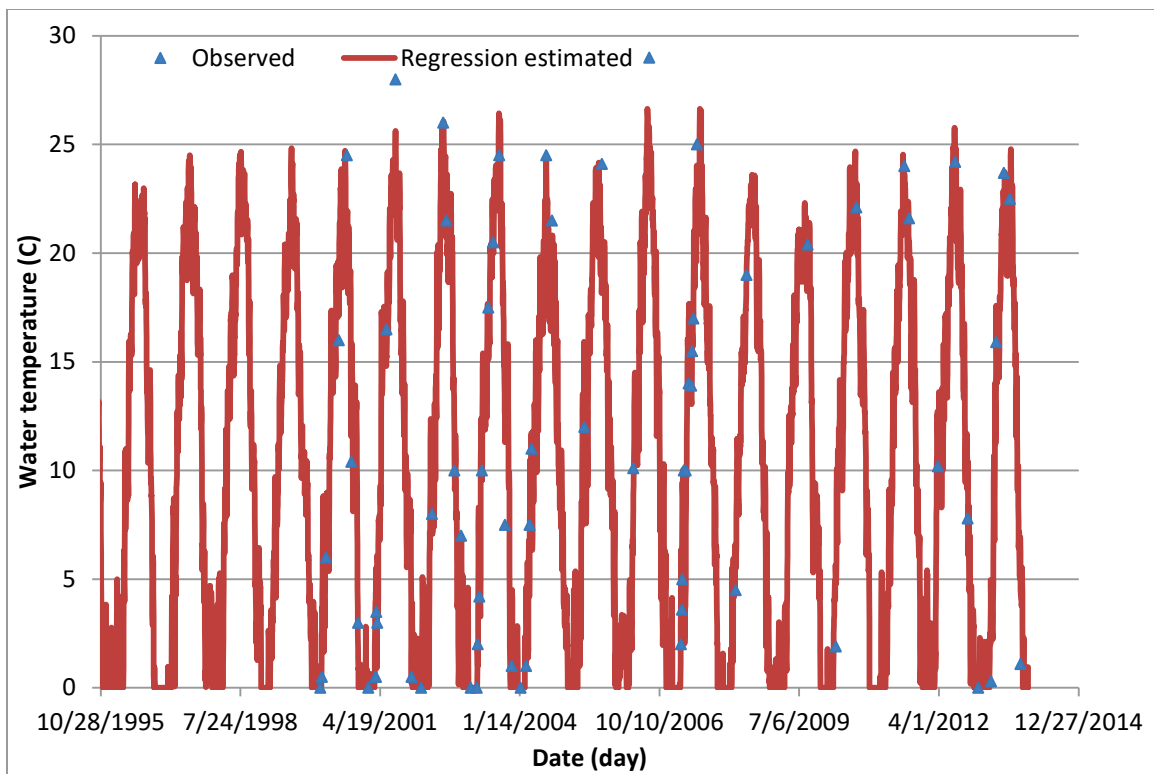
Figure A8. Regression computed versus observed water temperatures at BC8.
