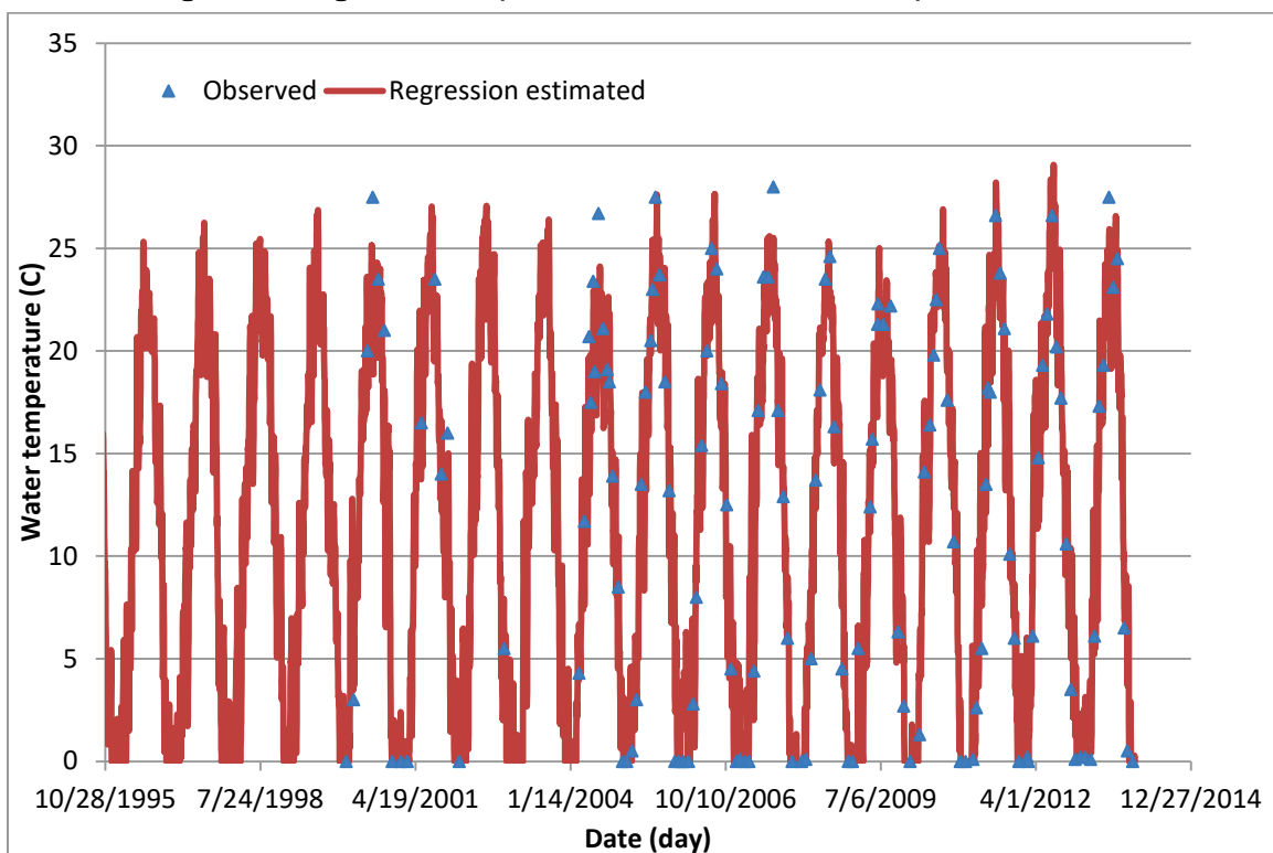
Figure B5. Regression computed versus observed water temperatures at BC5.
