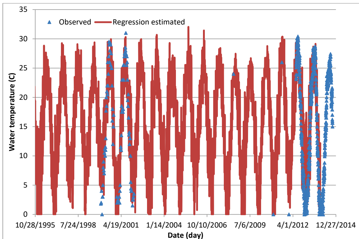
Figure B1. Regression computed versus observed water temperatures at BC1.
