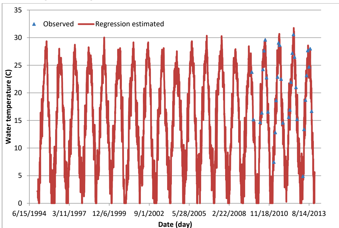
Figure C16. Regression computed versus observed water temperatures at BC16.
