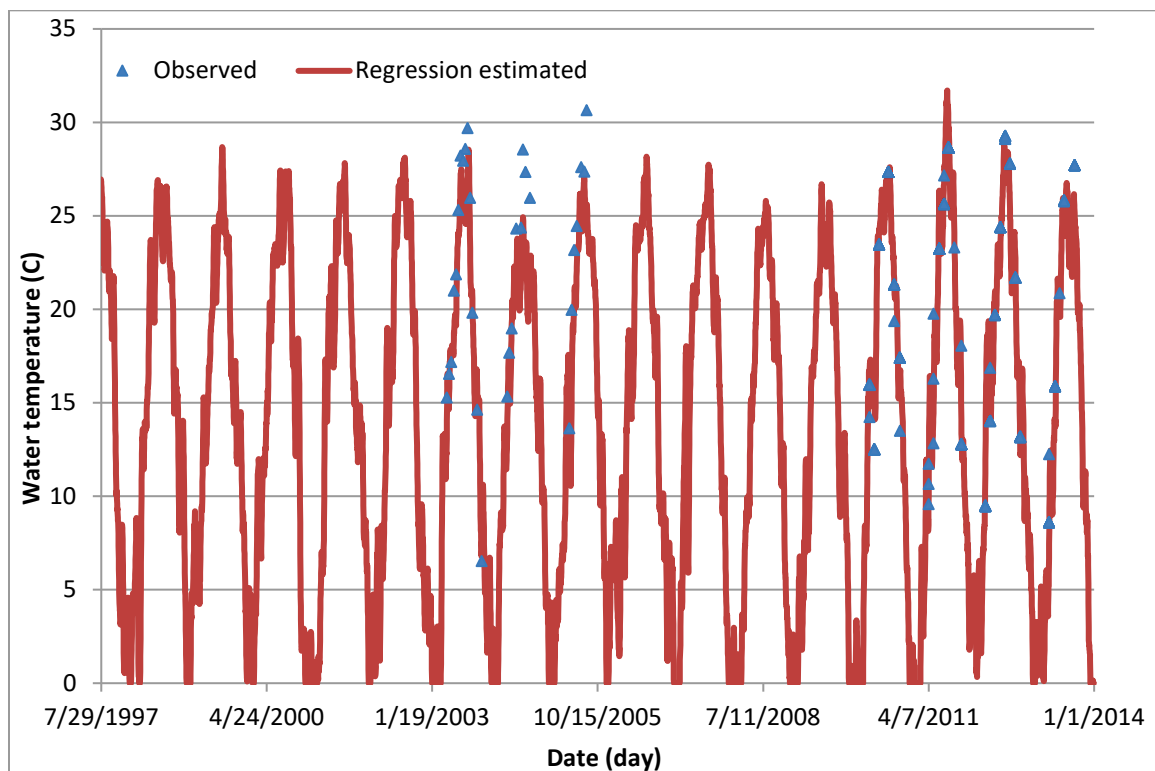
Figure C1. Regression computed versus observed water temperatures at BC1.
