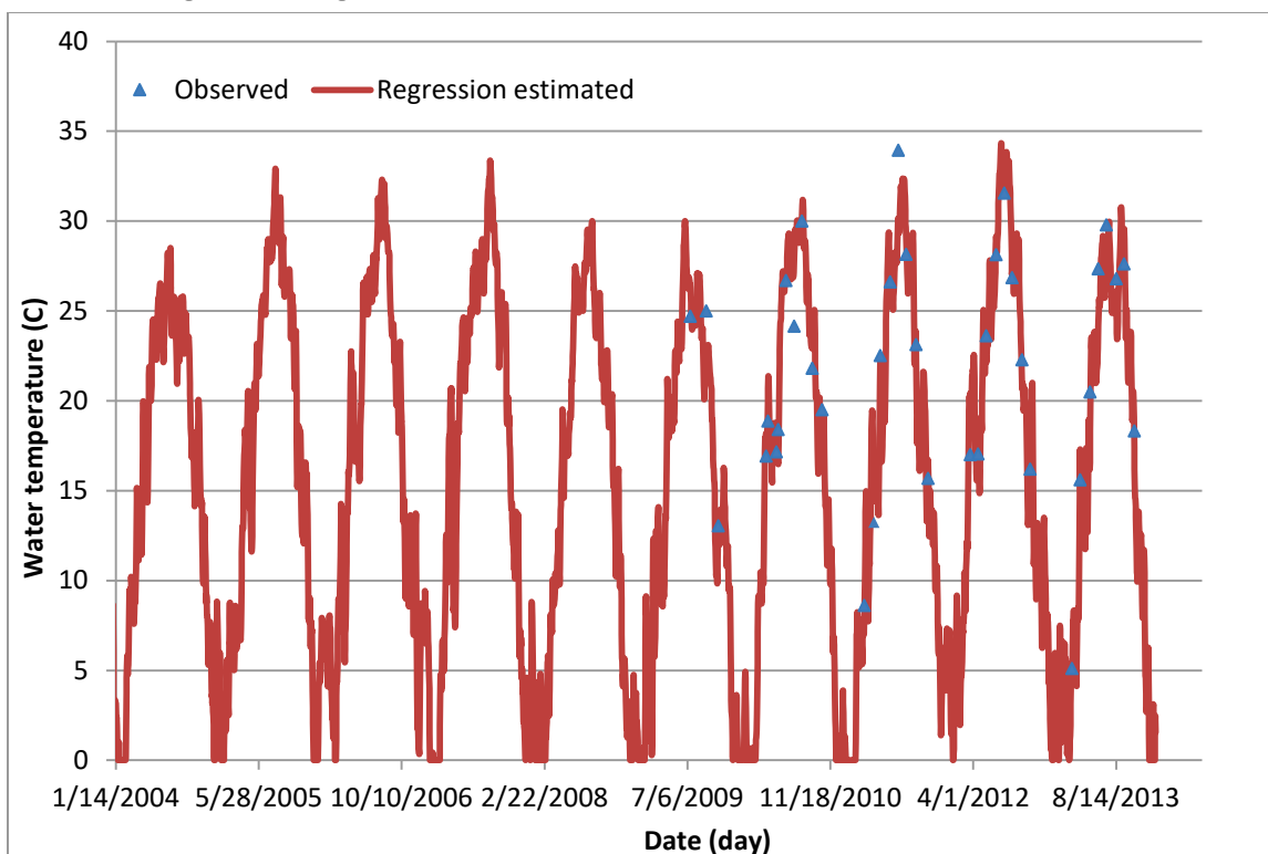
Figure C2. Regression computed versus observed water temperatures at BC2.
