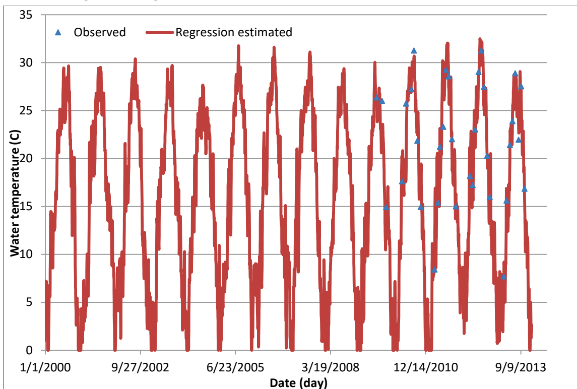
Figure C4. Regression computed versus observed water temperatures at BC4.
