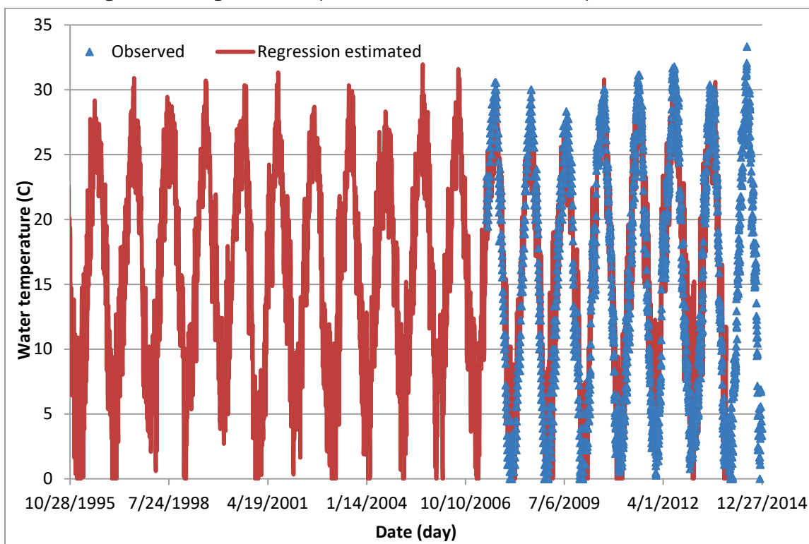
Figure C11. Regression computed versus observed water temperatures at BC11.
