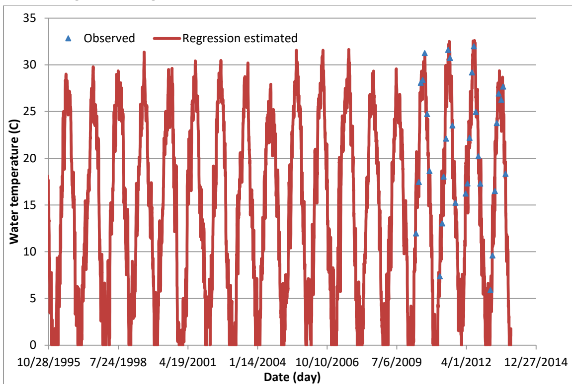
Figure C20. Regression computed versus observed water temperatures at BC20.
