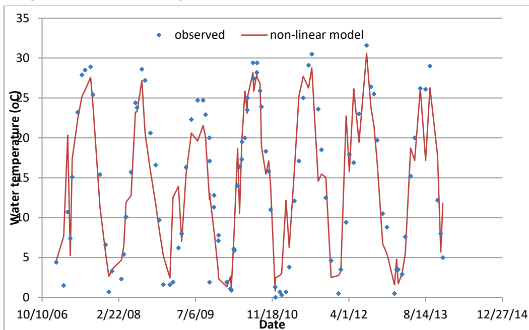
Figure 12. Observed and regression computed water temperatures at USGS 05587455.
