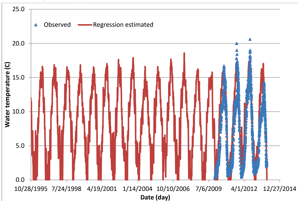
Figure A4. Regression computed versus observed water temperatures at BC4.
