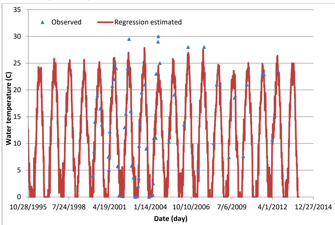
Figure A2. Regression computed versus observed water temperatures at BC2.
