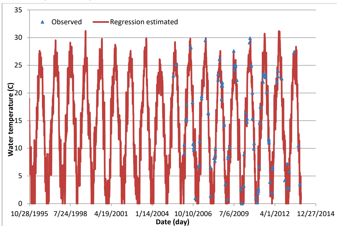
Figure C12. Regression computed versus observed water temperatures at BC12.
