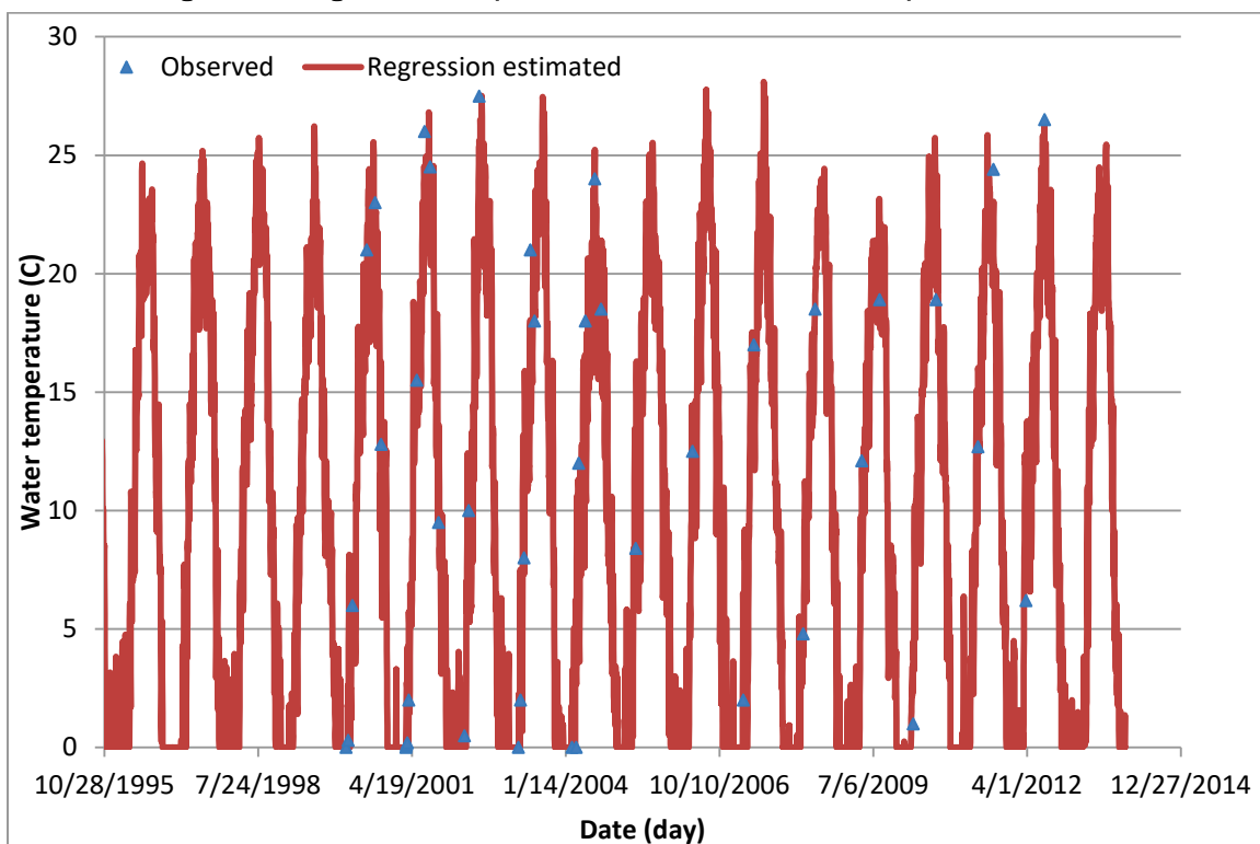
Figure A7. Regression computed versus observed water temperatures at BC7.
