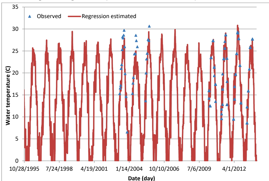
Figure C3. Regression computed versus observed water temperatures at BC3.
