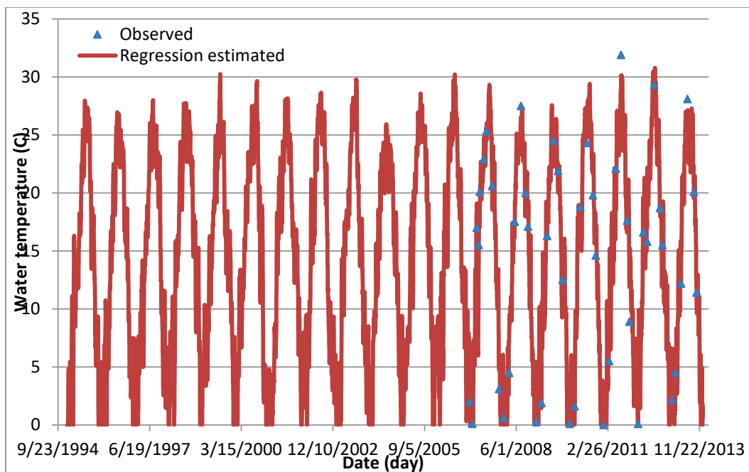
Figure C27. Regression computed versus observed water temperatures at BC27.
