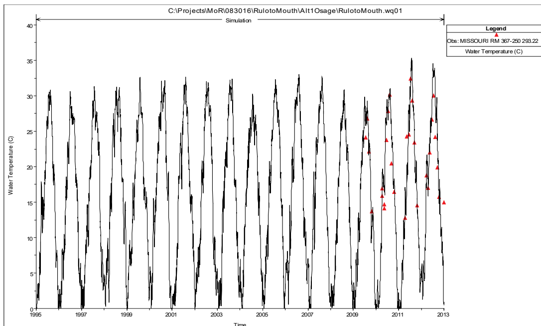
Figure 43. HEC-RAS predicted versus observed water temperatures of the Missouri River at Waverly, MO (USGS 06895500).
