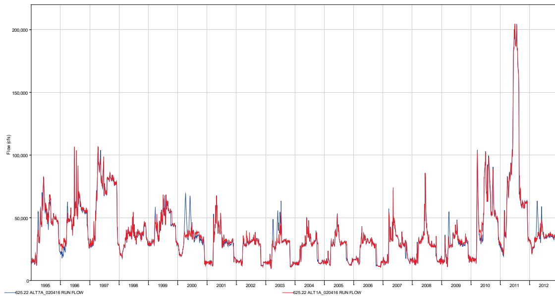
Figure 46. Model predicted daily mean flow discharge at Missouri River RM 625.22 for alternatives 1 and 7.
