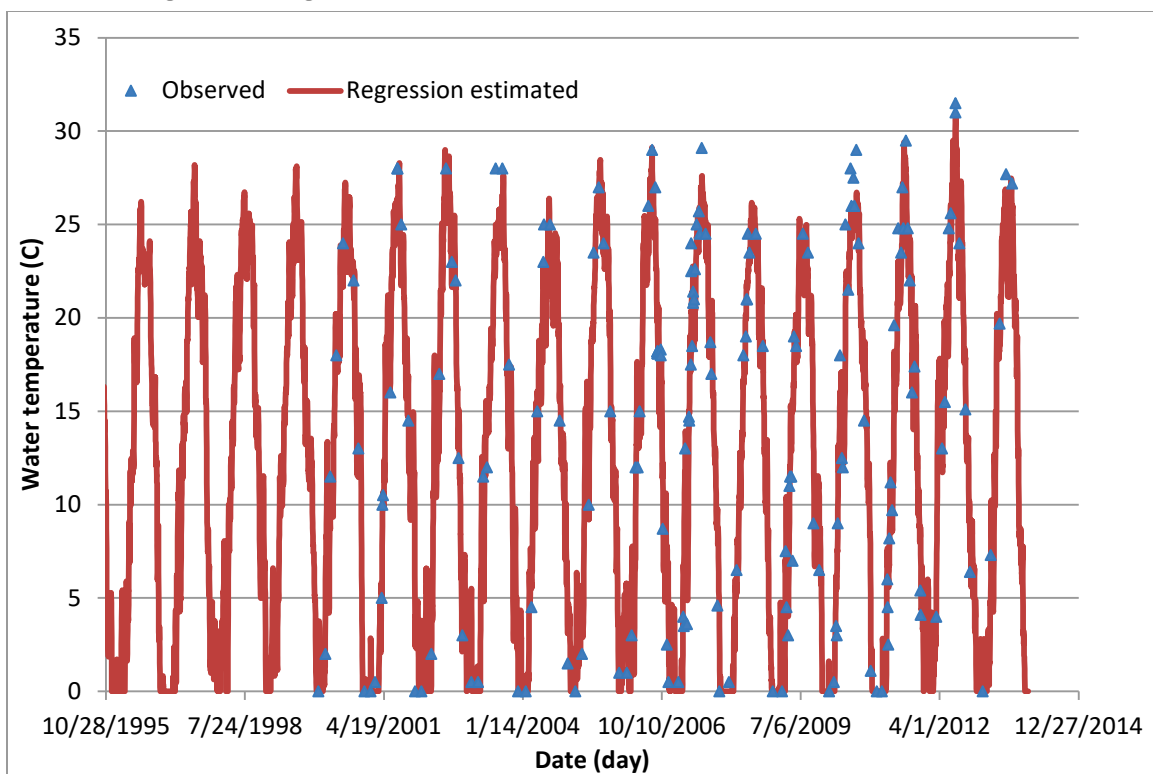
Figure B4. Regression computed versus observed water temperatures at BC4.
