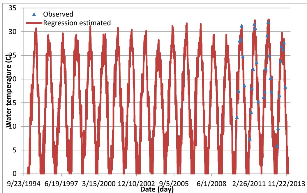
Figure C26. Regression computed versus observed water temperatures at BC26.
