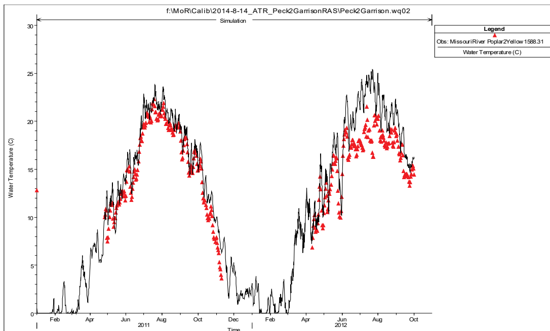
Figure 19. HEC-RAS predicted versus observed water temperatures of the Missouri River at Nohly, MT.
