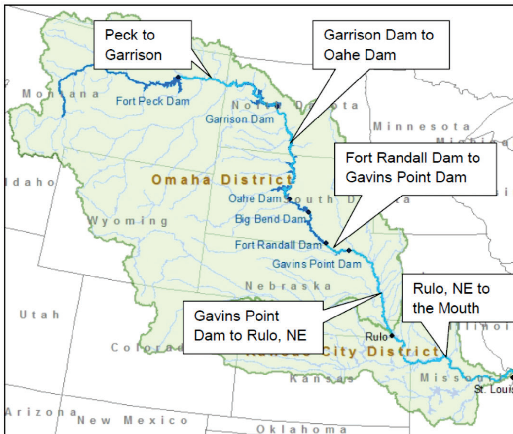
Figure 2. HEC-RAS modeled reaches on the Missouri River (USACE 2015).
