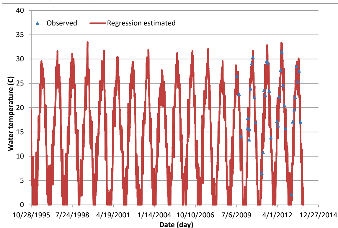
Figure C5. Regression computed versus observed water temperatures at BC5.
