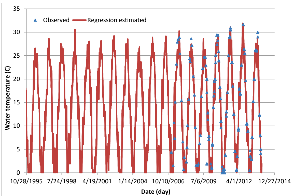
Figure C8. Regression computed versus observed water temperatures at BC8.
