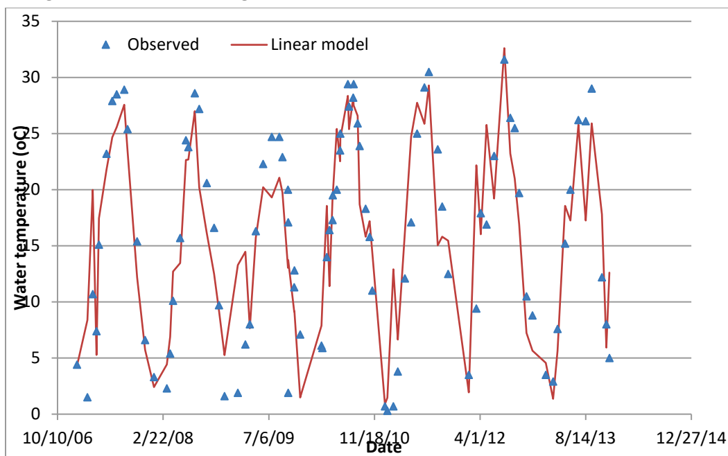
Figure 10. Observed vs. regression-computed water temperatures at USGS 05587455.
