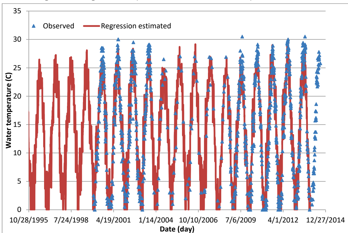
Figure B11. Regression computed versus observed water temperatures at BC11.
