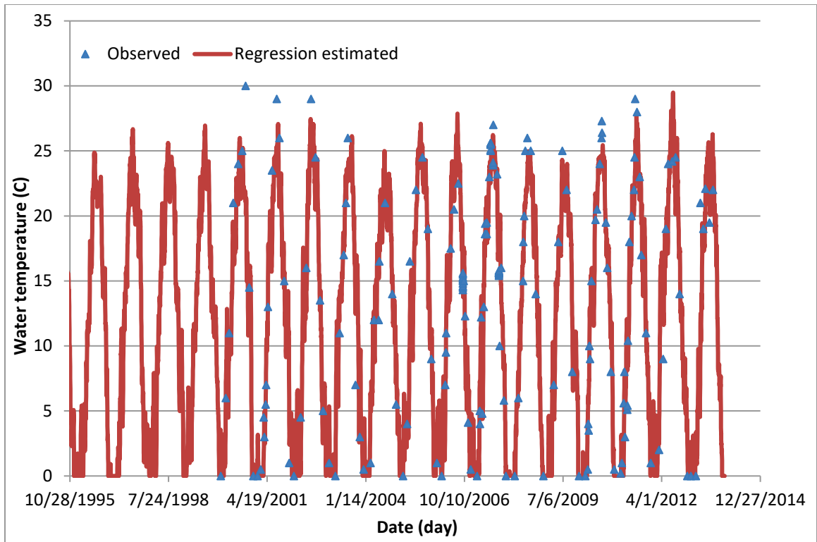
Figure B16. Regression computed versus observed water temperatures at BC16.
