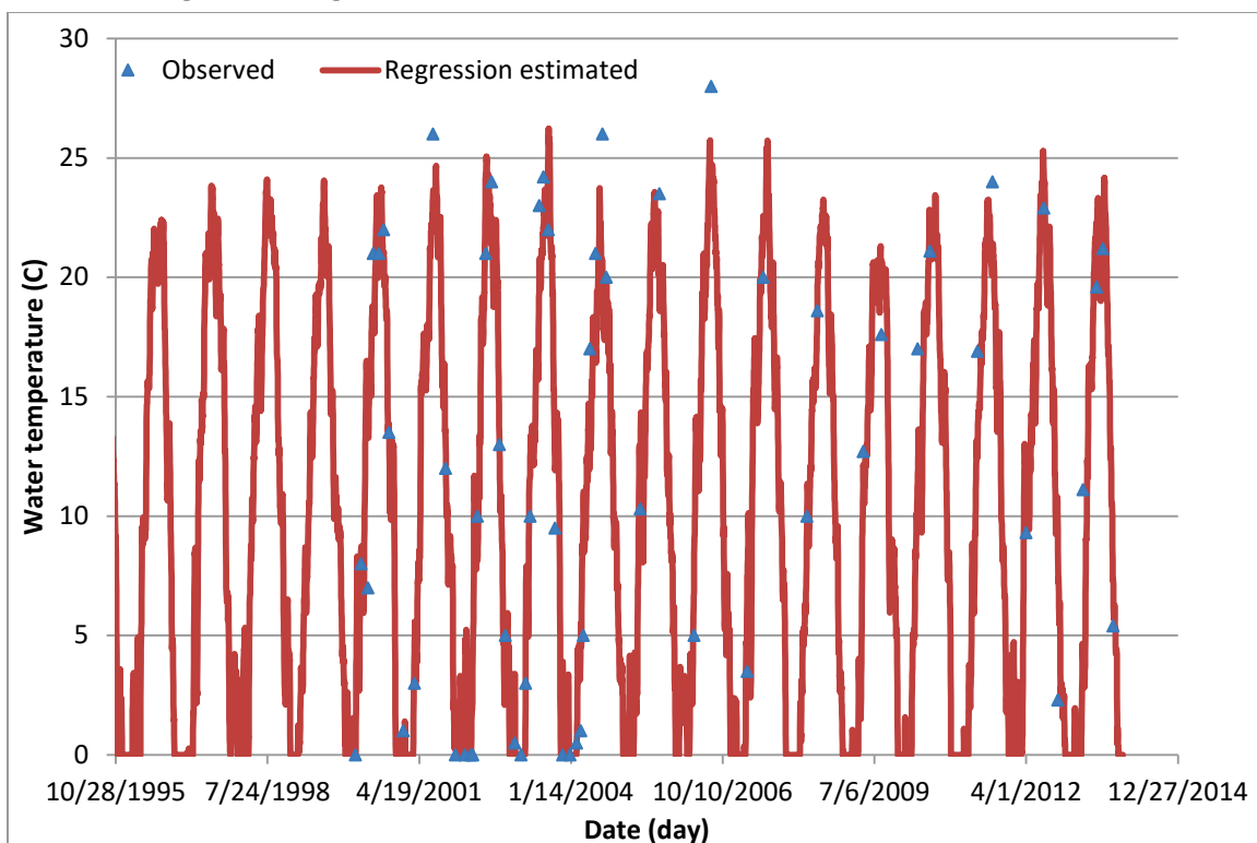
Figure A6. Regression computed versus observed water temperatures at BC6.
