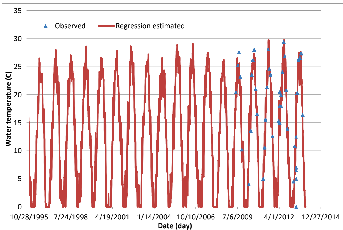
Figure B10. Regression computed versus observed water temperatures at BC10.
