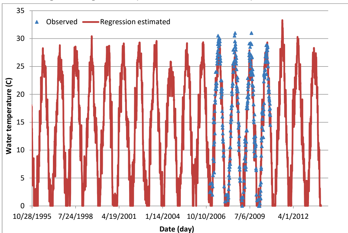
Figure C9. Regression computed versus observed water temperatures at BC9.
