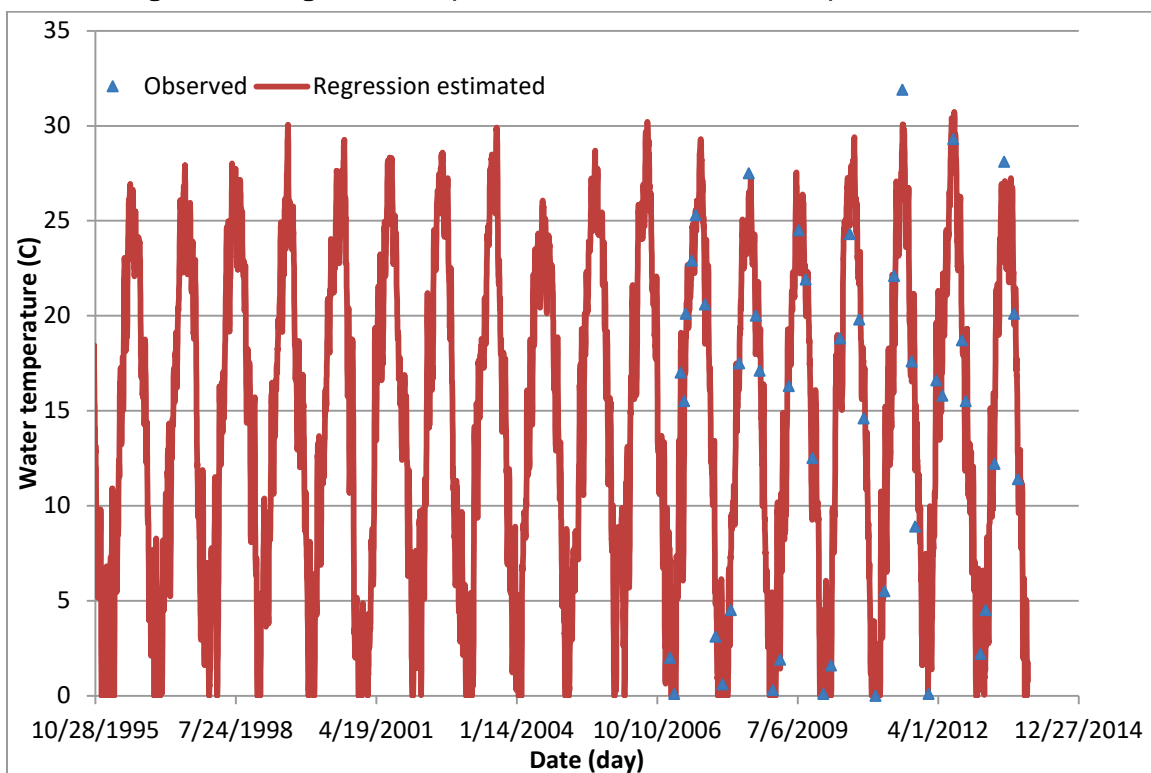
Figure C21. Regression computed versus observed water temperatures at BC21.
