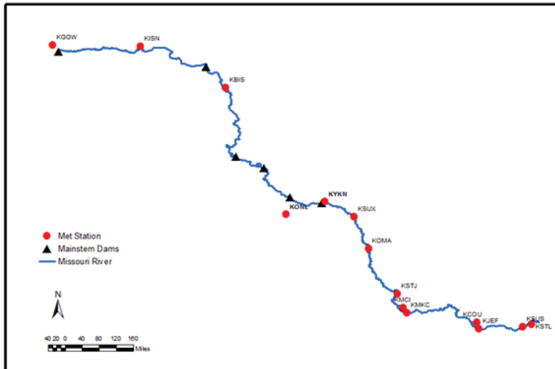
Figure 4. Distribution of meteorological stations used in the Missouri River HEC-RAS models.
