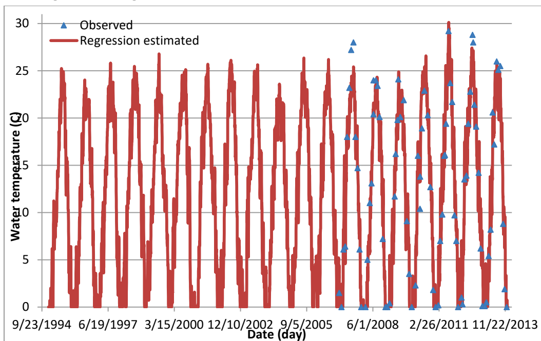
Figure C24. Regression computed versus observed water temperatures at BC24.
