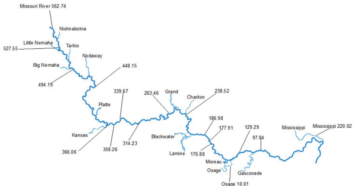
Figure 39. Schematic representation of inflow boundary locations included in the HEC-RAS model from Rulo to the mouth of the Missouri River.
