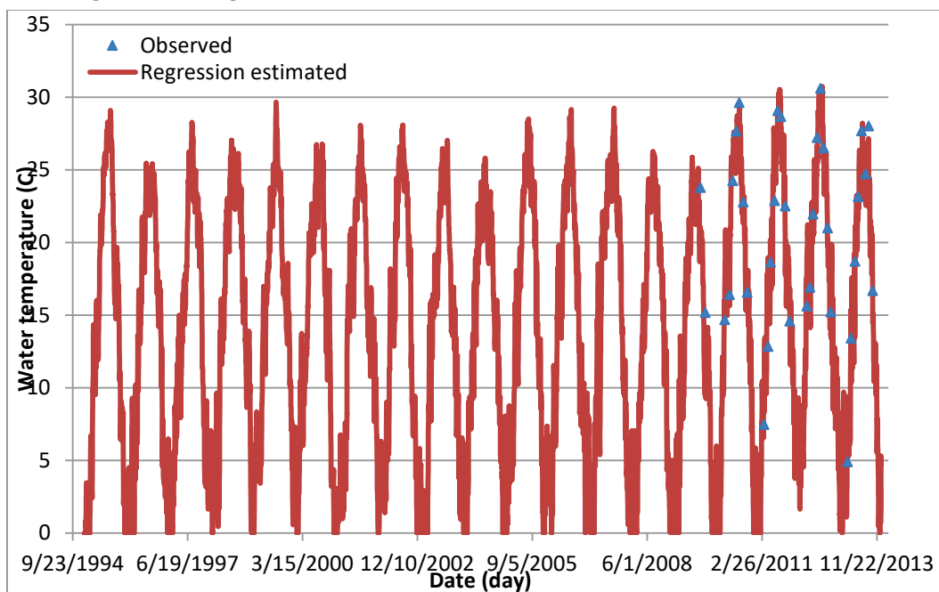
Figure C22. Regression computed versus observed water temperatures at BC22.
