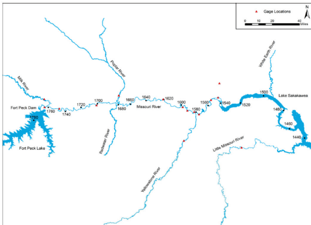
Figure 15. HEC-RAS model extent for the Fort Peck Dam to Garrison Dam reach (USACE 2015).
