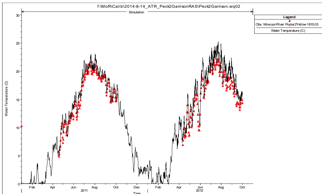
Figure 18. HEC-RAS predicted versus observed water temperatures of the Missouri River at Culbertson, MT.
