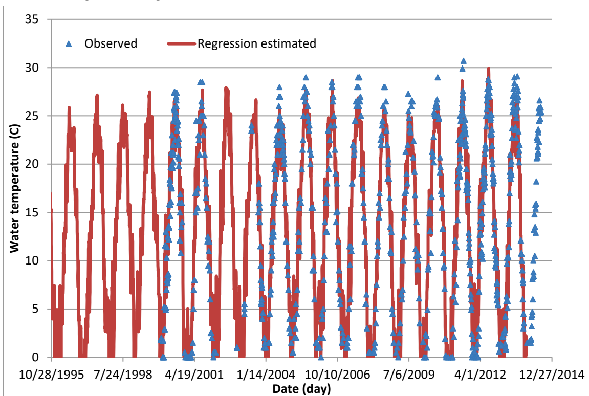
Figure B8. Regression computed versus observed water temperatures at BC8.
