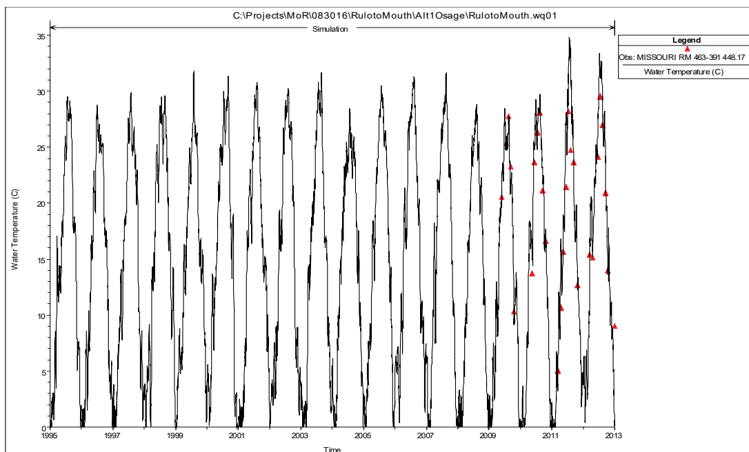
Figure 41. HEC-RAS predicted versus observed water temperatures of the Missouri River at St. Joseph, MO (USGS 06818000).
