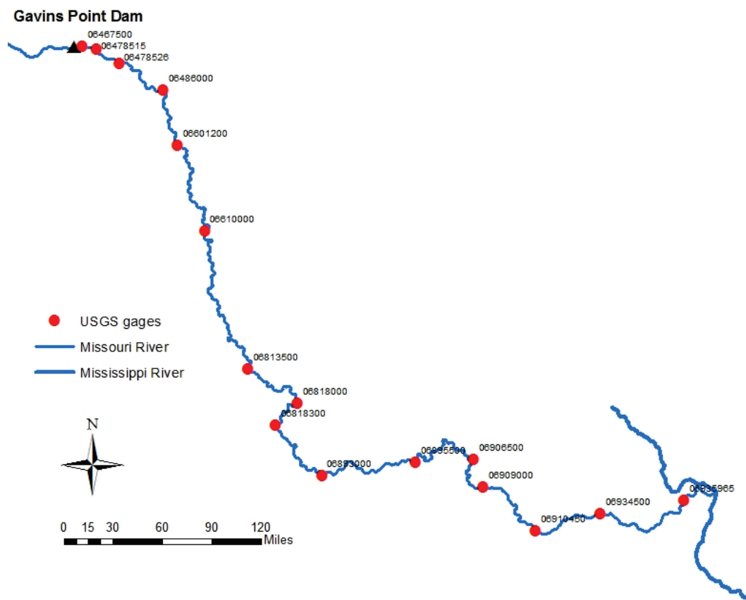
Figure 31. HEC-RAS water temperature calibration locations from the Gavins Point Dam to the mouth of the Missouri River.
