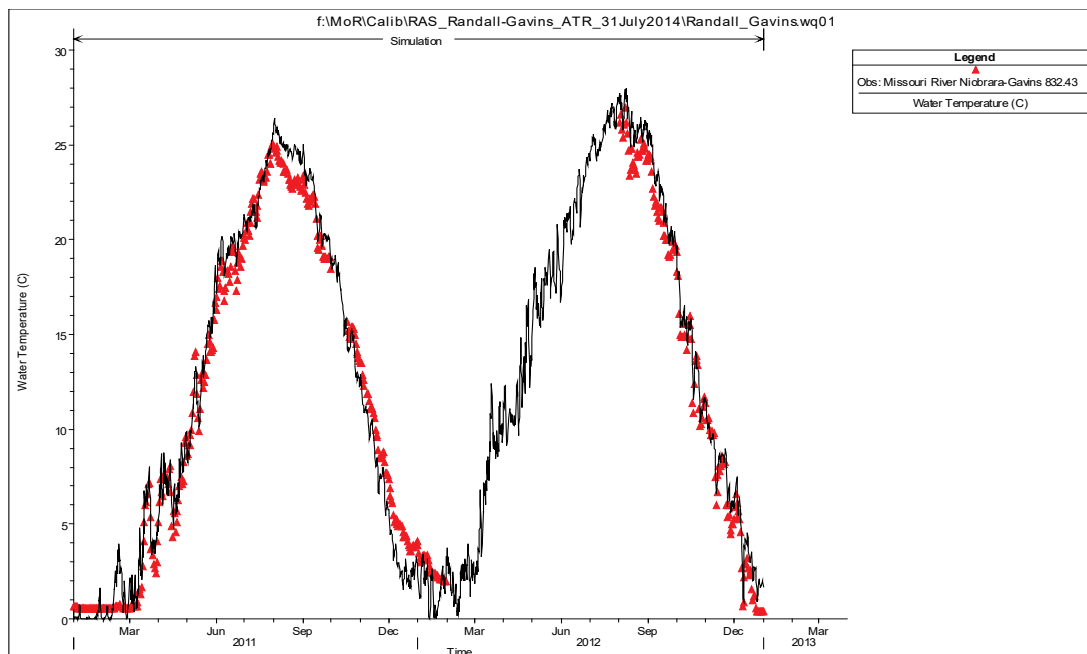
Figure 27. HEC-RAS predicted versus observed water temperatures of the Missouri River at Springfield, SD (USGS 06466700).
