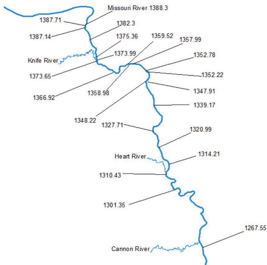
Figure 22. Schematic representation of inflow boundary locations included in the HEC-RAS model for the Garrison Dam to Oahe Dam reach.
