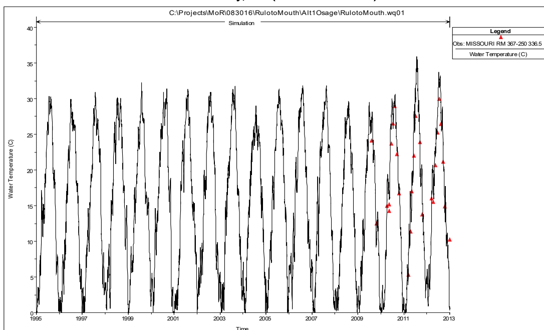
Figure 42. HEC-RAS predicted versus observed water temperatures of the Missouri River at Kansas City, MO (USGS 06893000).
