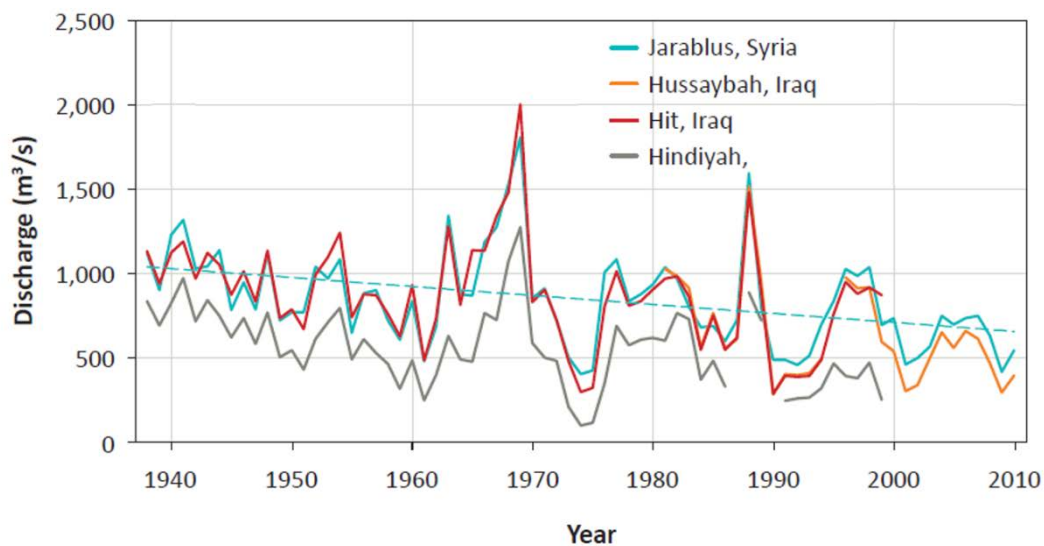
Figure 12. Euphrates Mean Annual Discharge (m³/s) 1937 to 2010
