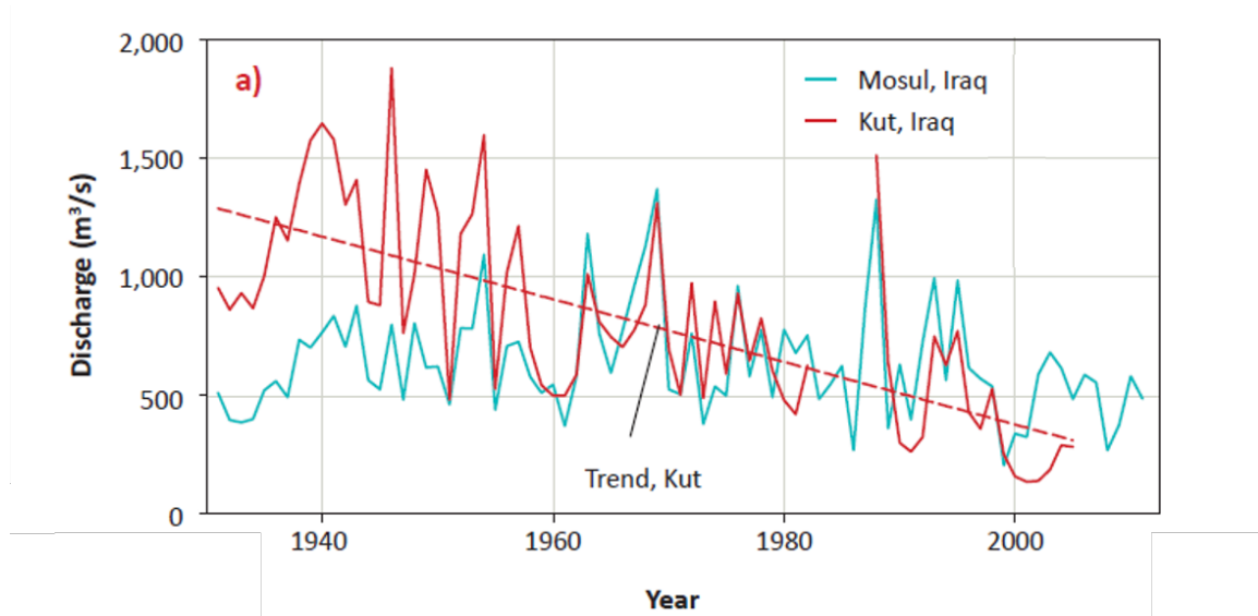
Figure 13. Tigris Mean Annual Discharge (m³/s) 1931 to 2011
