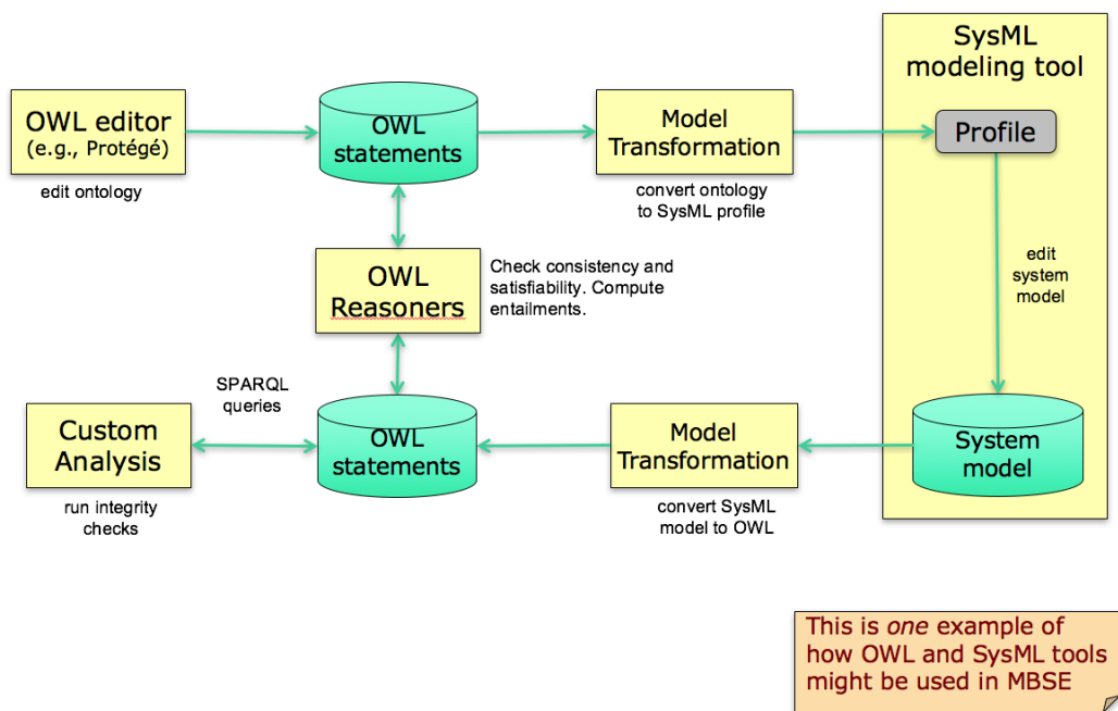
Figure 8. From Ontologies to SysML Profiles and Back to Analyzable OWL / RDF
