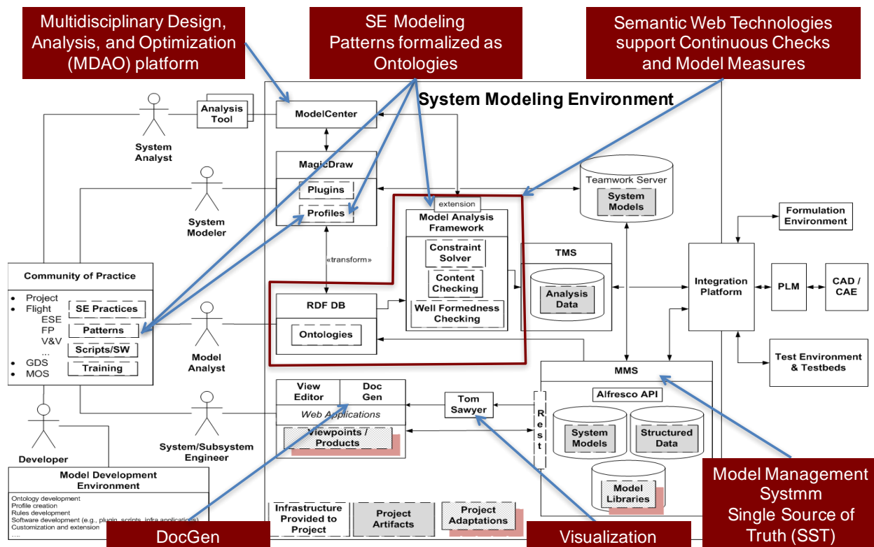
Figure 57. OpenMBEE Instantiation (2014)[118]
