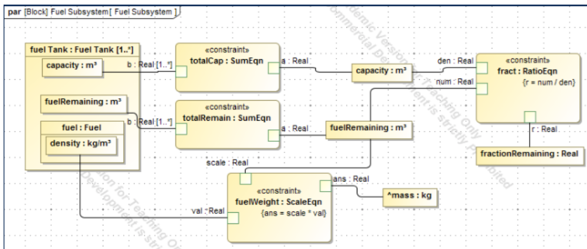
Figure 46. Parametric Diagram of Fuel System
