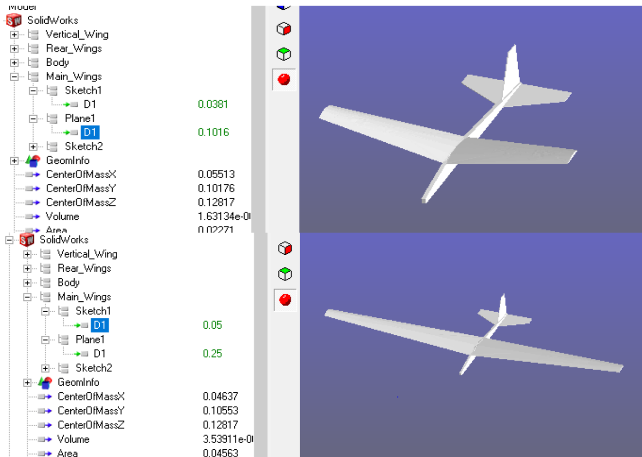
Figure 33. MDAO Workflow with SolidWorks Computer Aided Design Model
