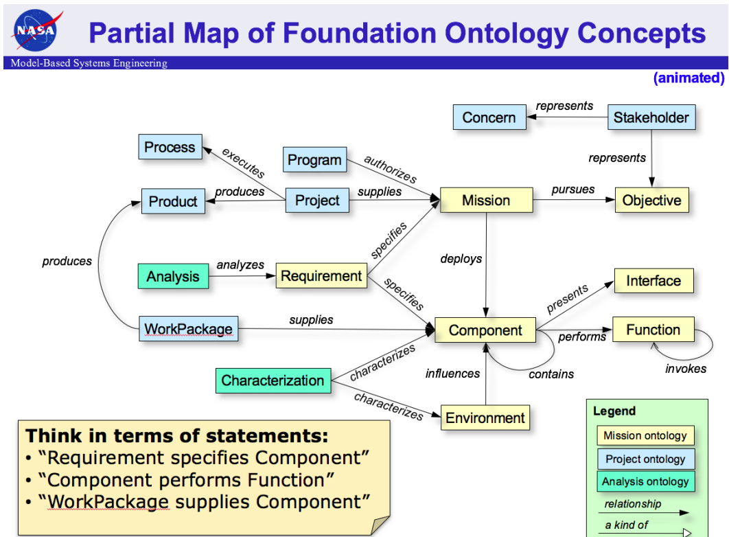
Figure 7. NASA/JPL Foundational Ontology for Systems Engineering
