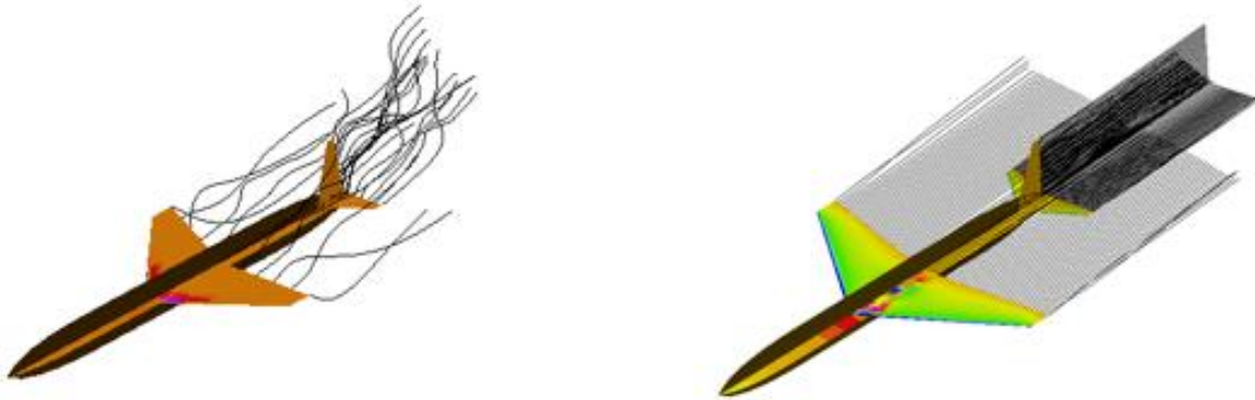
Figure 34. CFD Mesh Fidelity Importance
