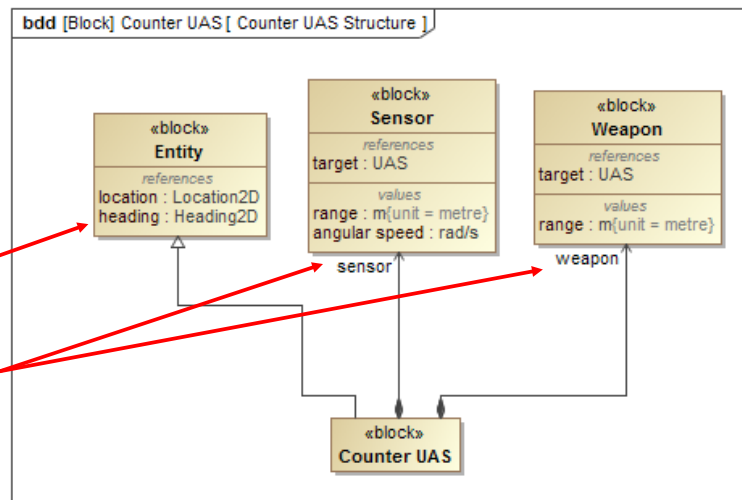
Block Definition diagram (model system attributes)
