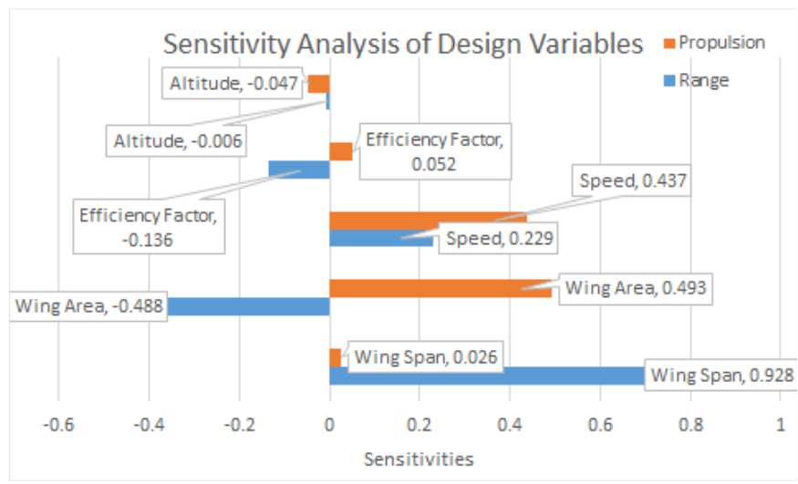
Figure 32. Sensitivity of Objectives to Design Variables
