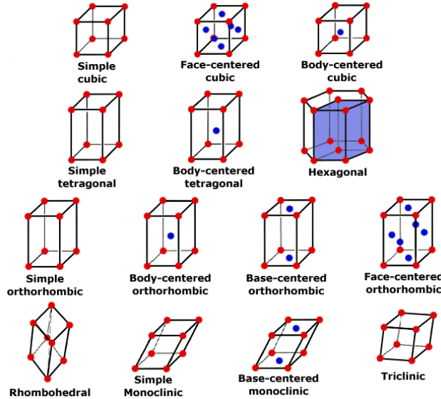
Figure 10: 14 Types of Bravais Crystal Unit Cells
