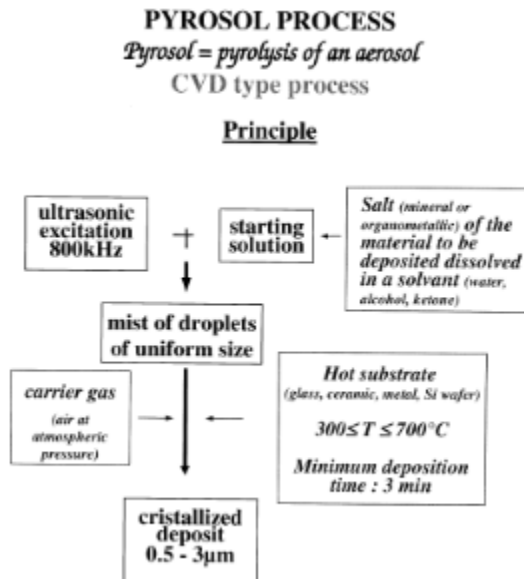
Figure 40: Schematic Description of the Pyrosol Process [224]
