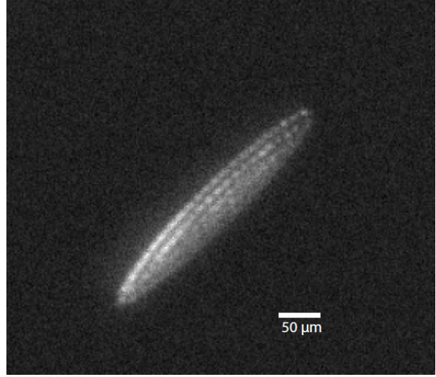
(b) A crystal of trapped Yb + ions
