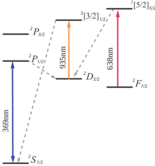
(a) Yb + energy levels
