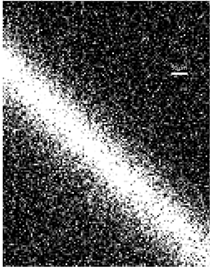
(b) Yb fluoresce
