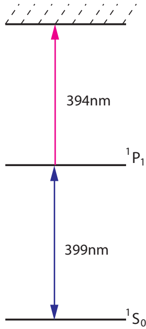
(a) Yb ionization scheme
