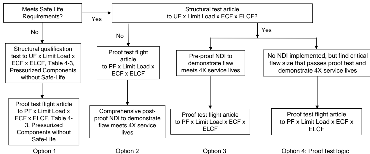
Figure 5-1. Qualification strategies for engine elements, excepting qualification by analysis (no test option), and by similarity. ECF - Environmental correction factor, ELCF - External load correction factor, UF - Ultimate Factor, PF – Proof Factor
