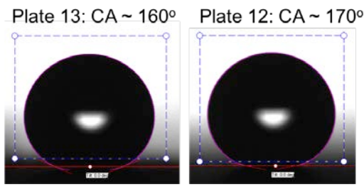
Figure 13. (a) The CA of the best coating (plate 13) is approximately 160^\circ . The coating based on micron size silica (i.e. plate 12) has the highest CA that is approximately 170^\circ . However, their sheet resistance values are not consistent. (b) Particle size analysis of the micron size spherical silica. The mean size is 9.2 \pm 2.8 \mu\text{m} .
