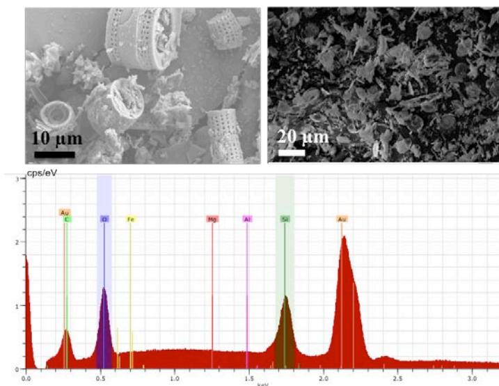
Figure 4. EDX spectrum and SEM images of the DE particles that were used in the fabrication of the coatings.
