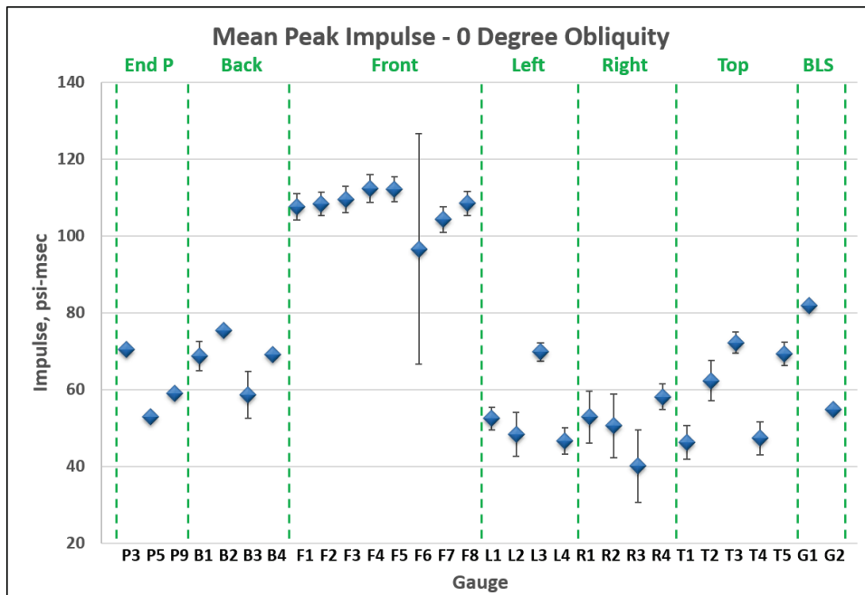
Figure 45. 95% confidence intervals on measured peak impulse for 0-degree obliquity.
