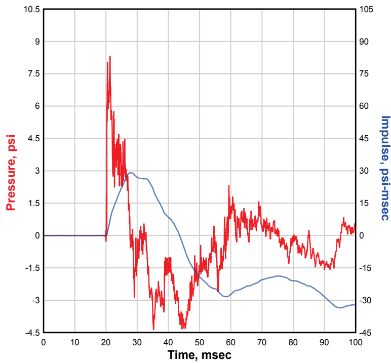
NATE 8x8, Single-Structure, 30 Degree, 4-ft Gap, Test 10 PBR3
