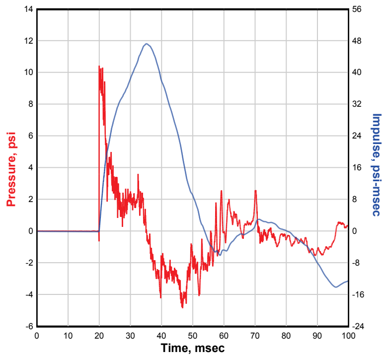
NATE 8x8, Single-Structure, 30 Degree, 4-ft Gap, Test 6 PBT5
