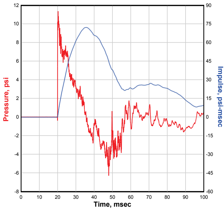
NATE 8x8, Single-Structure, 30 Degree, 4-ft Gap, Test 8 PBT5
