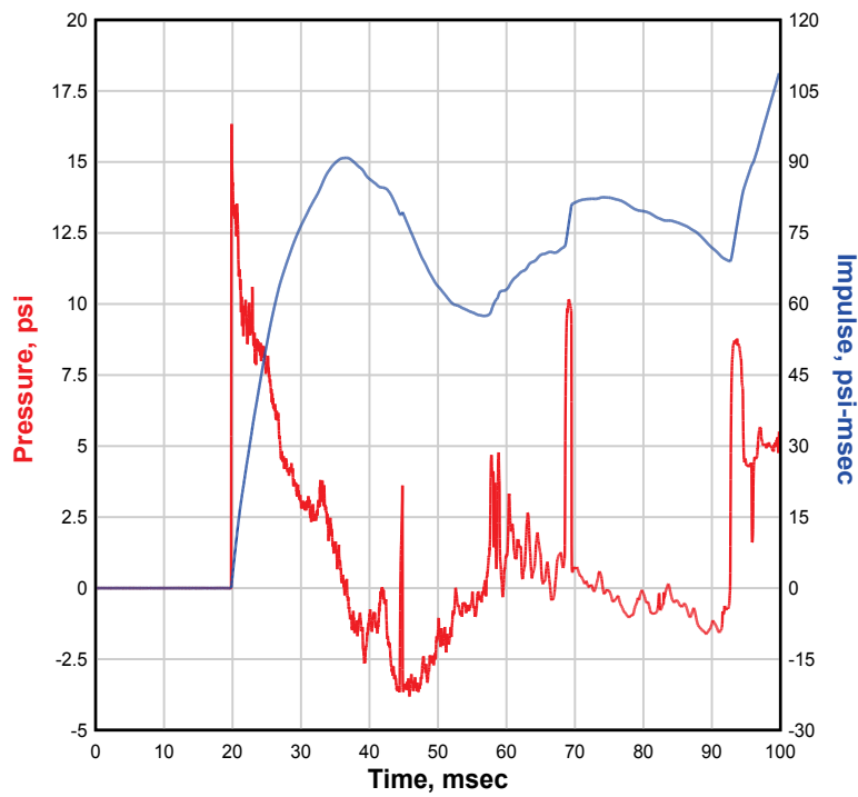
NATE 8x8, Single-Structure, 30 Degree, 4-ft Gap, Test 10 PBL3
