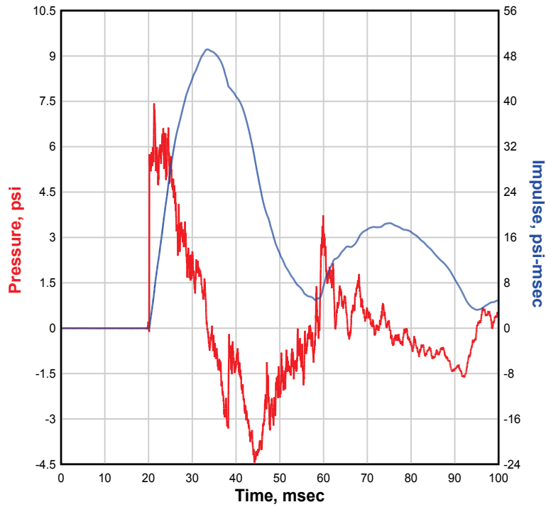
NATE 8x8, Single-Structure, 45 Degree, 4-ft Gap, Test 14 PBB3
