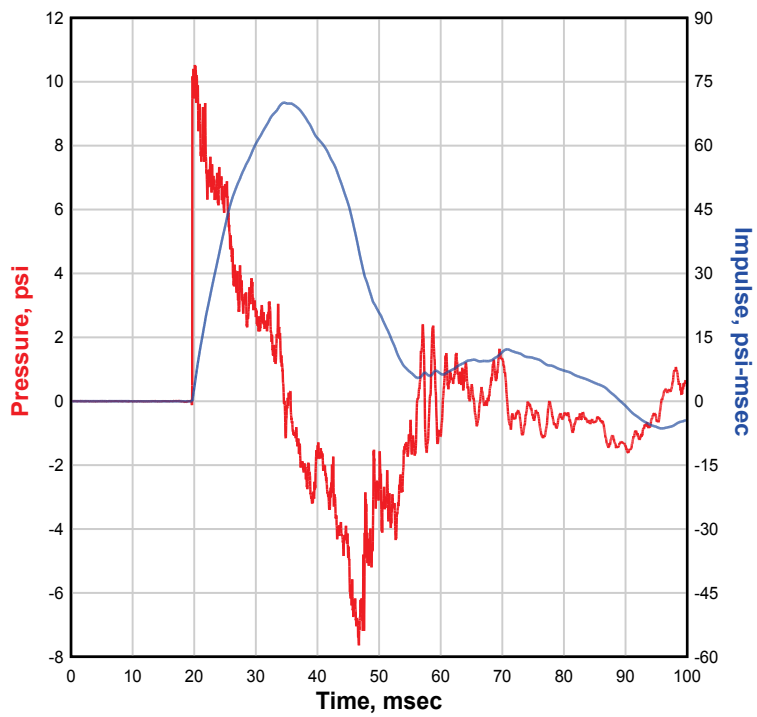
NATE 8x8, Single-Structure, 45 Degree, 4-ft Gap, Test 16 PBT5
