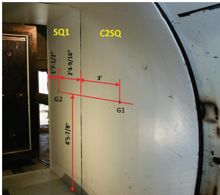
Figure 12. Gauge layout on the BLS side walls.
