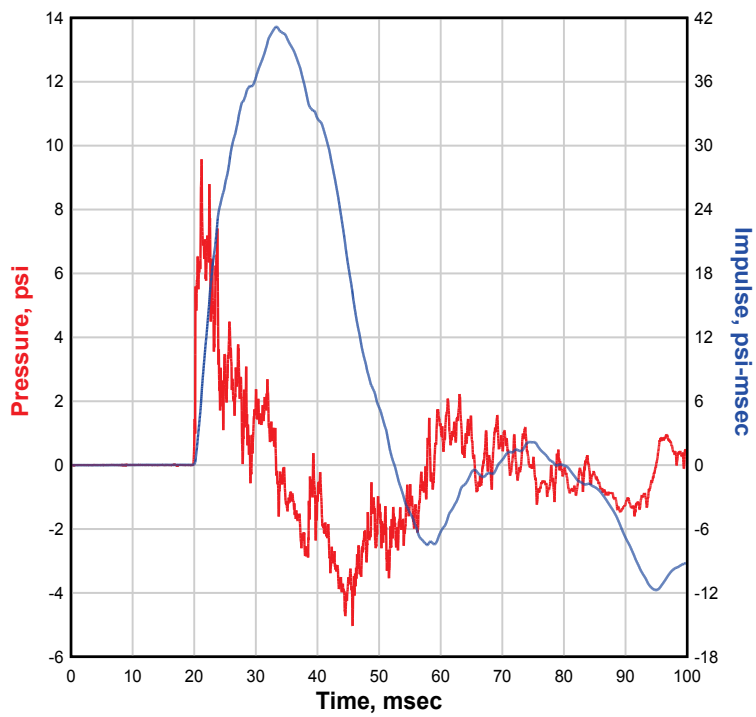
NATE 8x8, Single-Structure, 45 Degree, 4-ft Gap, Test 13 PBB1
