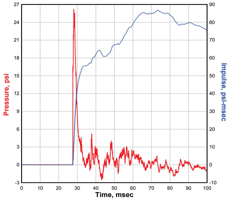
NATE 8x8, Single-Structure, 0 Degree, 4-ft Gap, Test 4 Burst Pressure = 778 psi CP5
