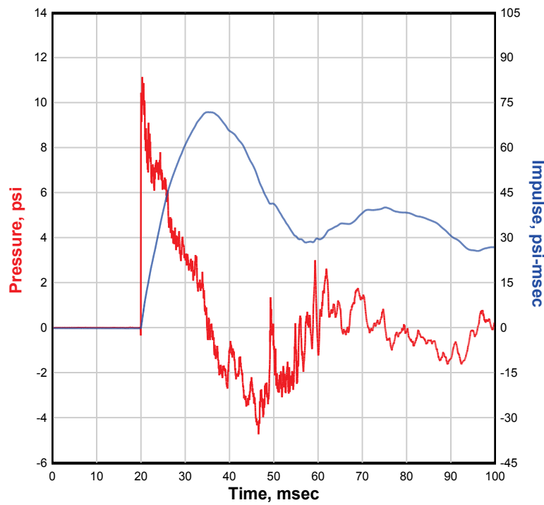
NATE 8x8, Single-Structure, 30 Degree, 4-ft Gap, Test 9 PBT5
