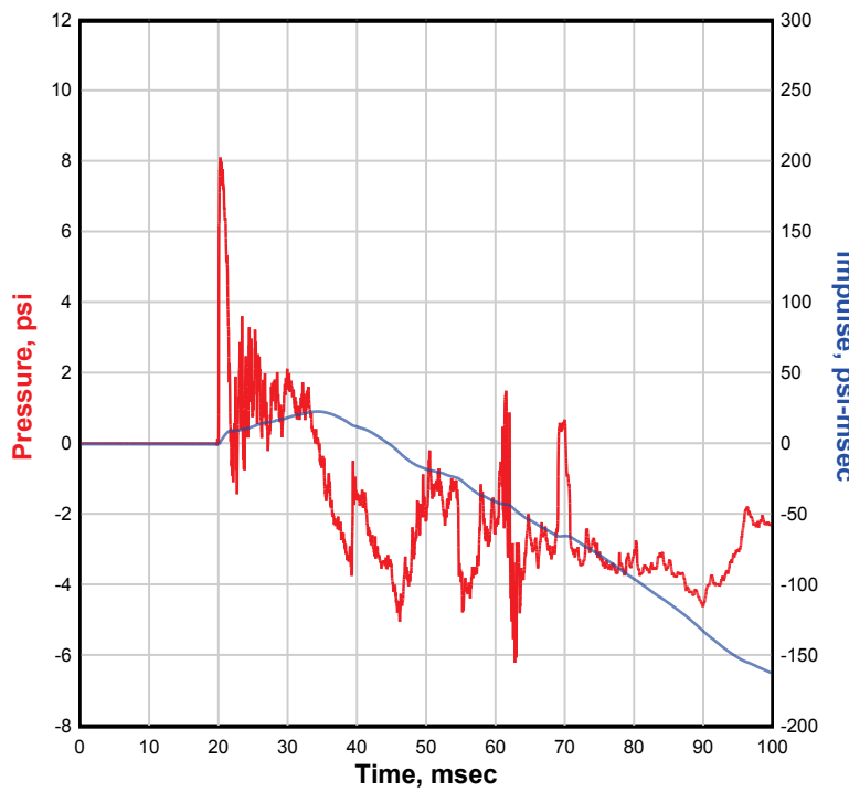
NATE 8x8, Single-Structure, 30 Degree, 4-ft Gap, Test 7 PBR3
