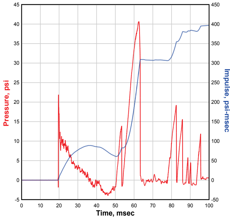
NATE 8x8, Single-Structure, 45 Degree, 4-ft Gap, Test 12 PBB1
