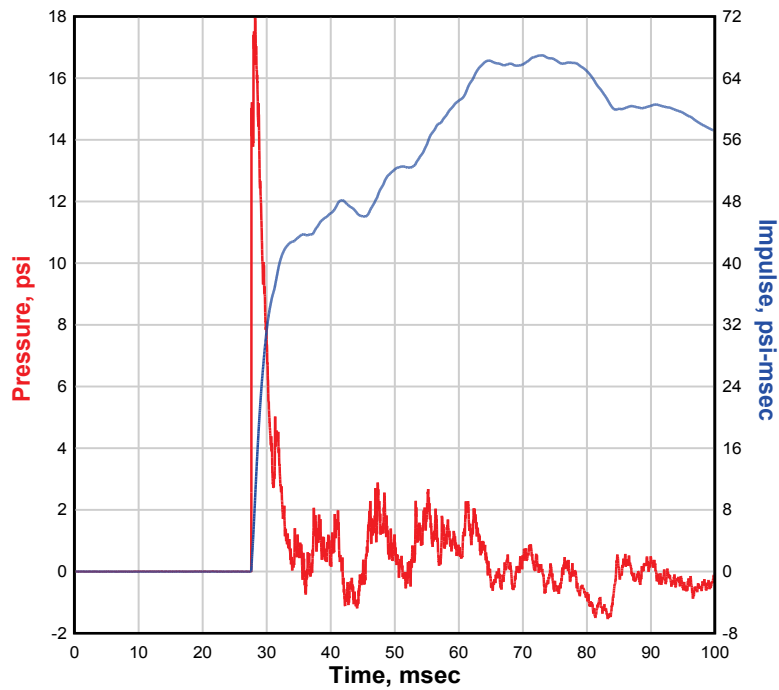
NATE 8x8, Single-Structure, 0 Degree, 4-ft Gap, Test 4 Burst Pressure = 778 psi CP5
