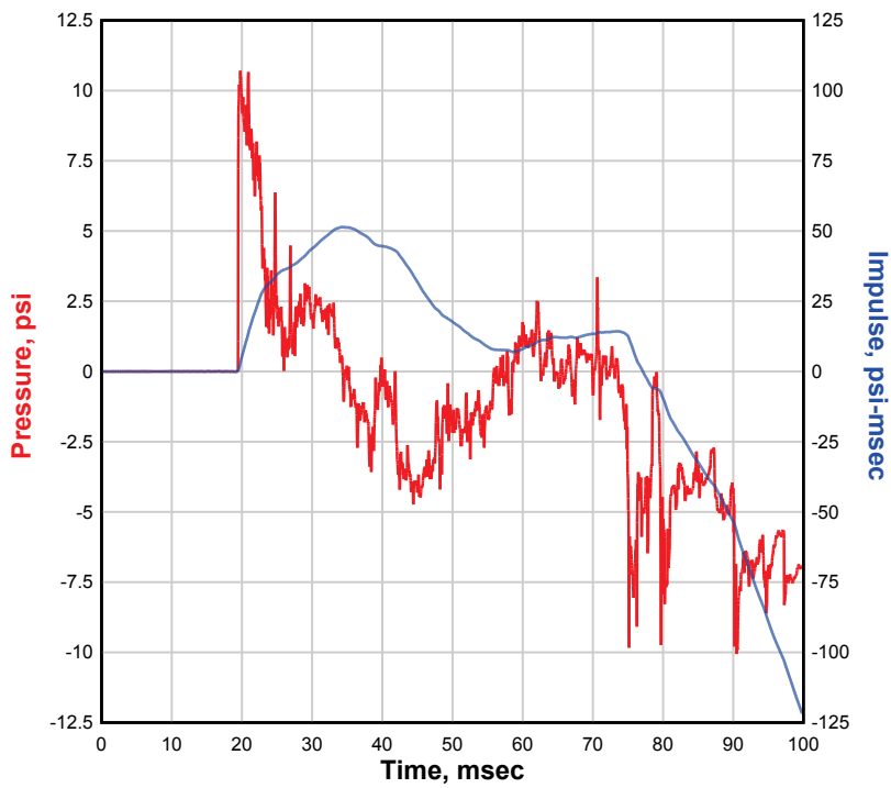
NATE 8x8, Single-Structure, 0 Degree, 4-ft Gap, Test 1 PBL1
