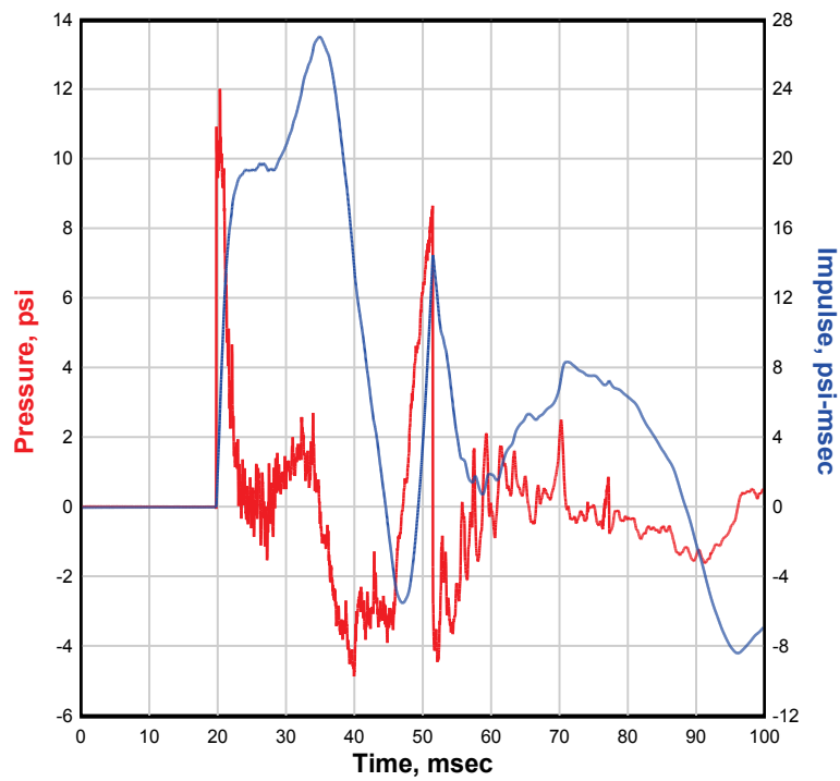
NATE 8x8, Single-Structure, 30 Degree, 4-ft Gap, Test 6 PBT1
