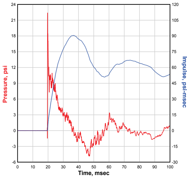
NATE 8x8, Single-Structure, 45 Degree, 4-ft Gap, Test 16 PBB1
