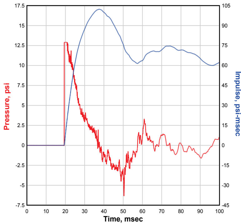
NATE 8x8, Single-Structure, 45 Degree, 4-ft Gap, Test 13 PBR1
