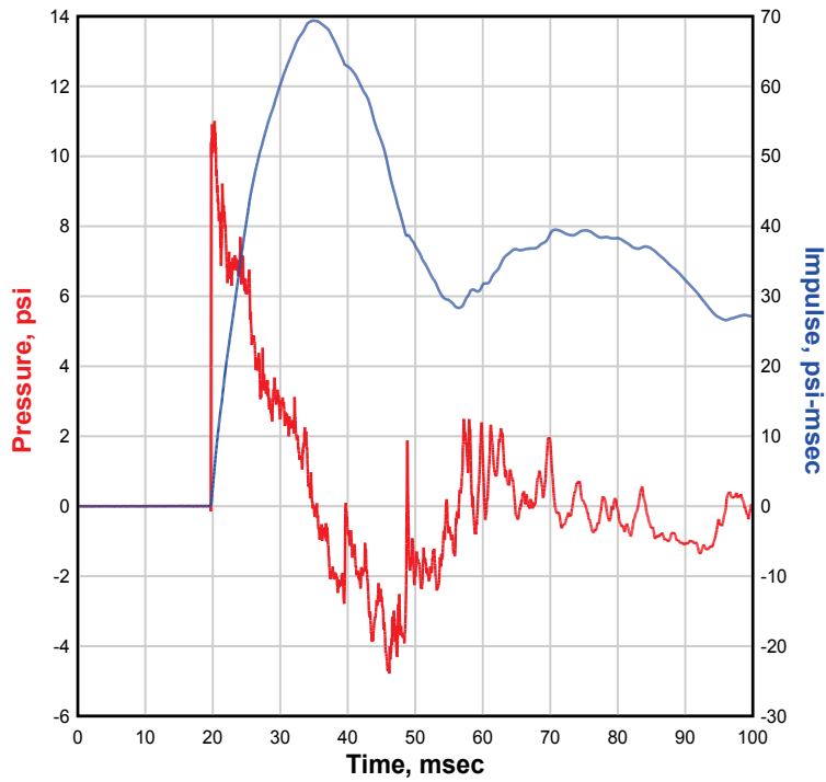
NATE 8x8, Single-Structure, 45 Degree, 4-ft Gap, Test 12 PBT3
