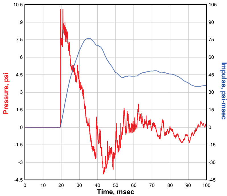
NATE 8x8, Single-Structure, 0 Degree, 4-ft Gap, Test 4 Burst Pressure = 778 psi G1
