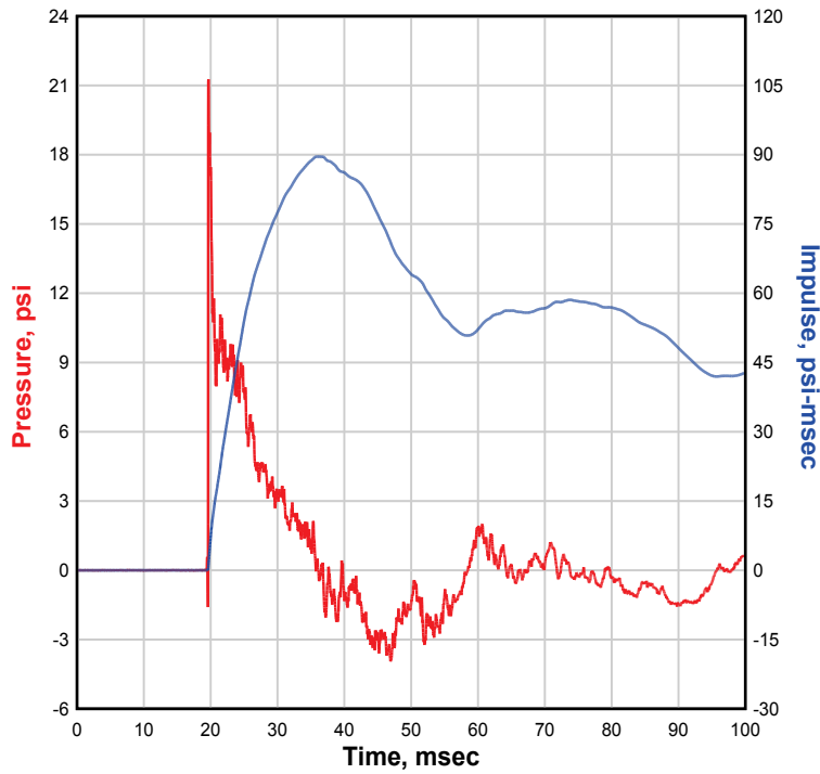
NATE 8x8, Single-Structure, 45 Degree, 4-ft Gap, Test 14 PBB1
