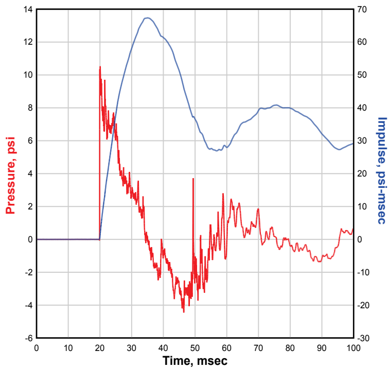
NATE 8x8, Single-Structure, 45 Degree, 4-ft Gap, Test 11 PBT3
