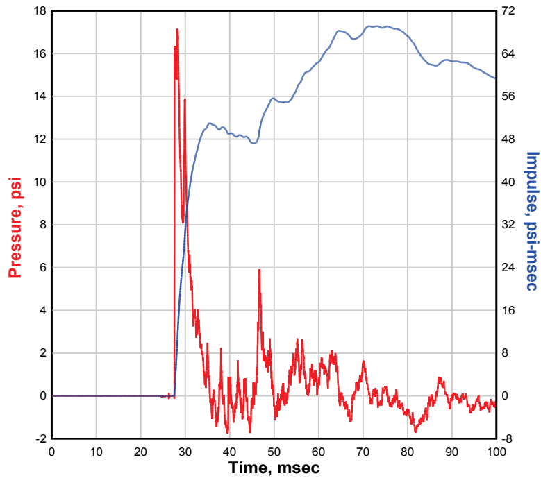
NATE 8x8, Single-Structure, 0 Degree, 4-ft Gap, Test 4 Burst Pressure = 778 psi G1
