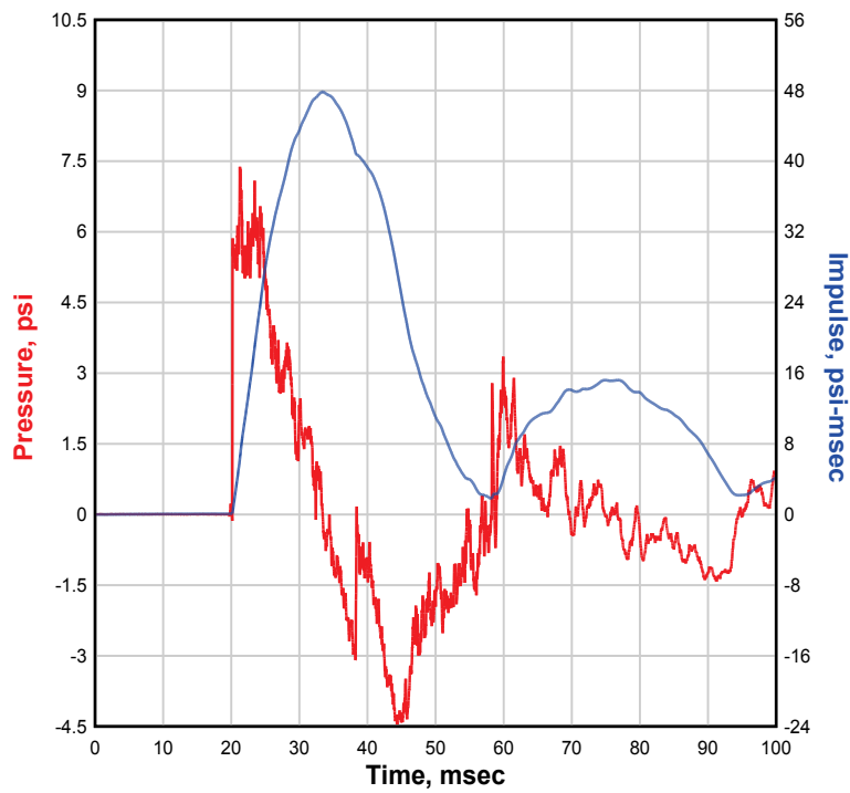
NATE 8x8, Single-Structure, 45 Degree, 4-ft Gap, Test 15 PBB3
