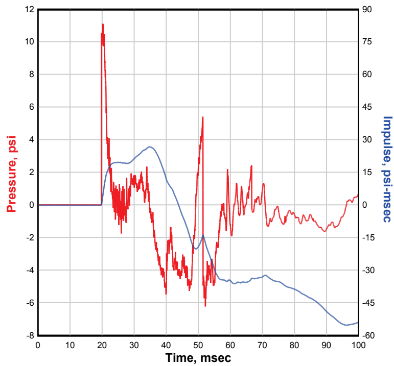
NATE 8x8, Single-Structure, 30 Degree, 4-ft Gap, Test 8 PBT1
