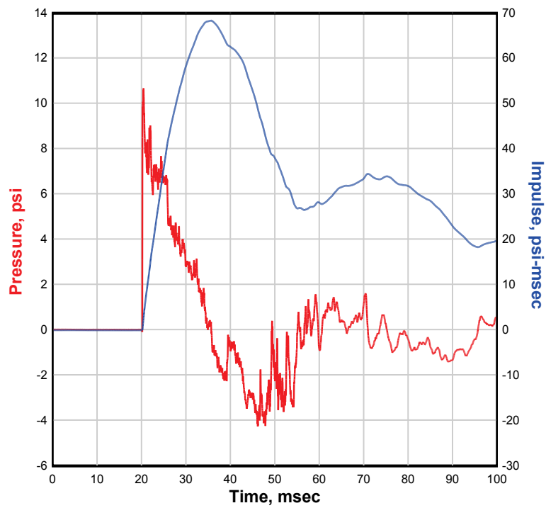
NATE 8x8, Single-Structure, 30 Degree, 4-ft Gap, Test 8 PBT3
