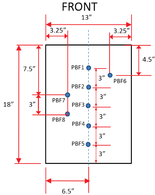
Figure 13. Gauge layout on the front of box structure.
