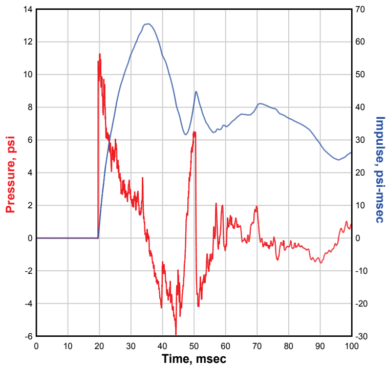
NATE 8x8, Single-Structure, 45 Degree, 4-ft Gap, Test 16 PBT1
