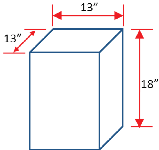
Figure 6. Box structure dimensions.
