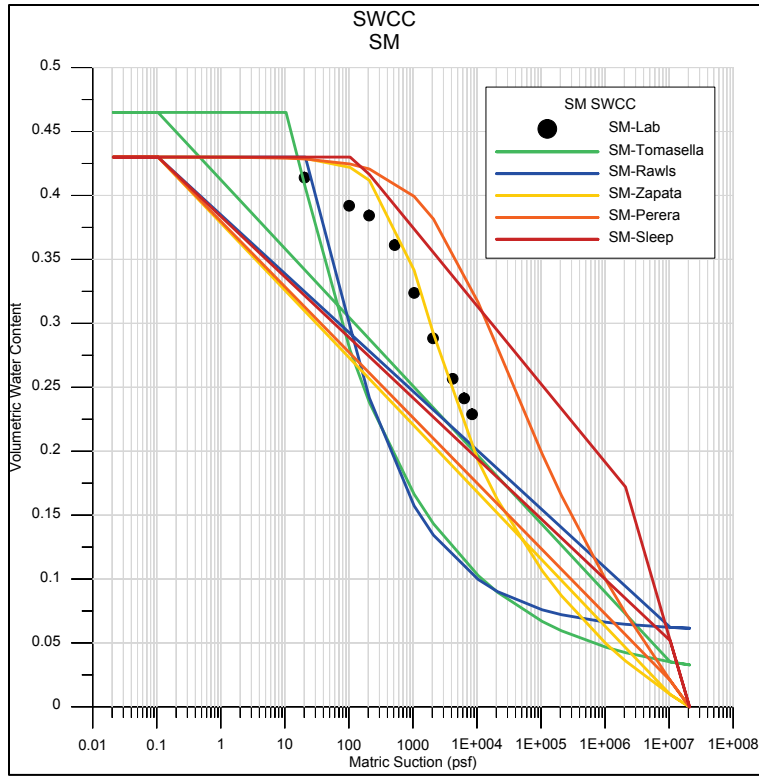
Figure 6. Predicted and laboratory SWCC for SM material.
