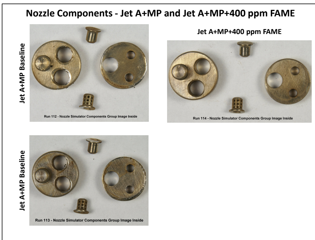
Figure 15 - Visible Deposition in Nozzle Screen Components
