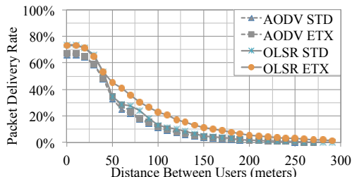
(b) Curve 25%
