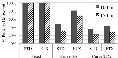
(b) OLSR
