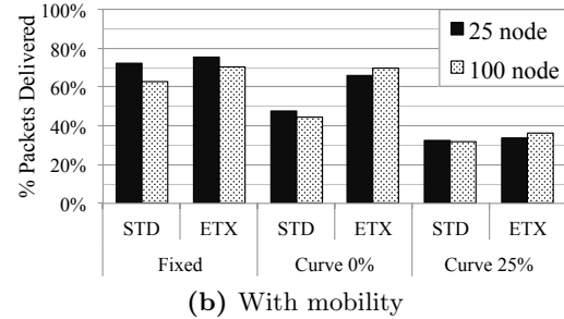
Figure 3: OLSR 100 meter radius: Packet delivery success rate
