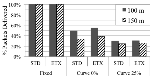
(a) AODV
