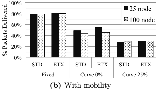
Figure 2: AODV 100 meter radius: Packet delivery success rate and queue overflows, data rates are set arbitrarily high. All of our simulations are performed using the OPNET network modeler [37], which has AODV and OLSR implemented according to IETF specifications.
