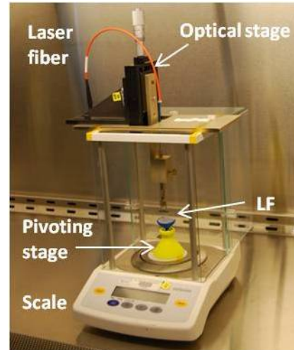
Figure 2: Laser fiber and LF holding fixture on scale.
