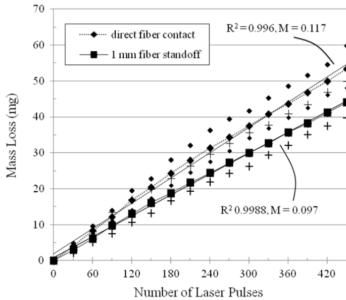
Figure 9: Average, maximum, and minimum mass loss of LF treated with Ho:YAG through 600 \mu\text{m} fiber, 5 Hz, 600 mJ.
