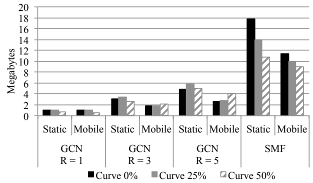
Figure 11: Number of bytes sent over-the-air with of GCN and SMF
