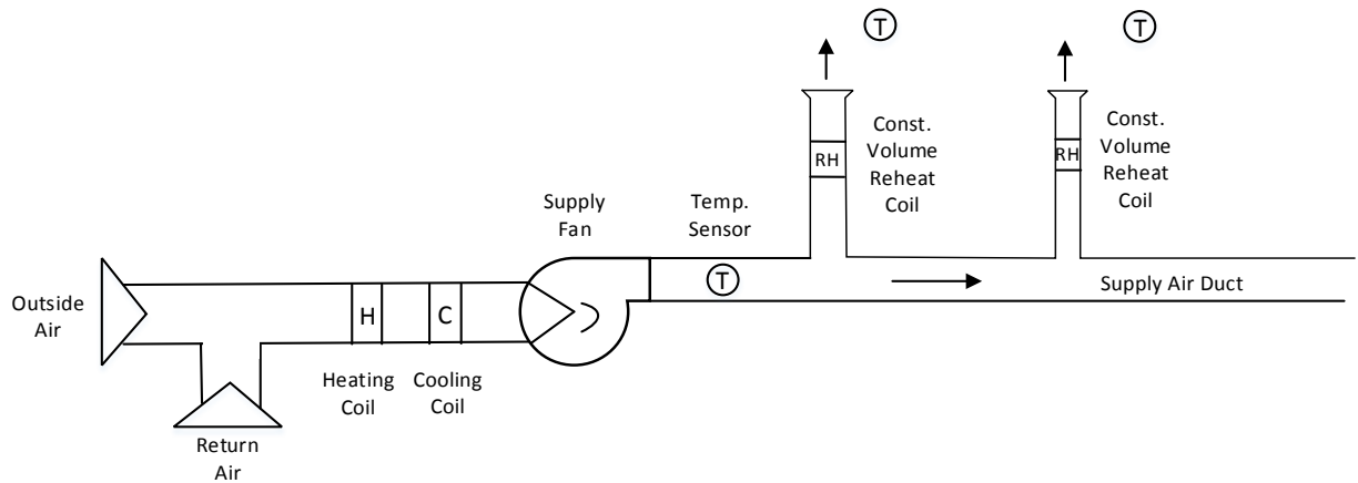
Figure 1. A Typical Single-duct CAV System Schematic
