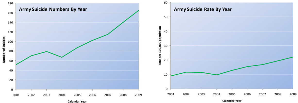
Diagram 3-5: Army Suicides 2001–2009
