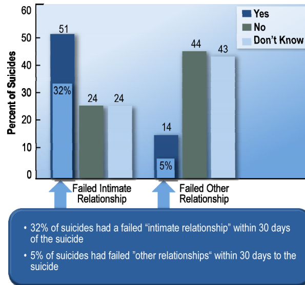
Diagram 7-2: Relationship History
